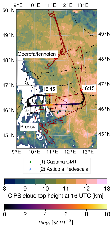
Figure 3. HALO flight track of F15 on the 13 July 2021 during CIRRUS-HL over Germany, Austria, Switzerland and Italy. The flight track is shown in red. Between 15:45 and 16:15 UTC (positions marked with red crosses) aerosol particle concentrations ( n_{500} ) are shown color-coded on the flight track, with bright yellow colors indicating high aerosol particle concentrations. Wind barbs displayed in this time section indicate wind speed and direction as measured by HALO research aircraft (half barb mark 5 \text{ m s}^{-1} , full barbs 10 \text{ m s}^{-1} ). The background depicts CiPS cloud top height at 16:00 UTC derived from MSG geostationary satellite images. White areas indicate clear sky conditions. The green and blue stars mark the precipitation measuring weather stations, Castana CMT and Astico a Pedescala, respectively. The flight track is shifted to account for parallax effect of the satellite viewing angle and is shown as it is seen from the satellite point of view. Red triangles mark the start and landing airport Oberpfaffenhofen (EDMO, Germany) and the dive location in Brescia-Montichiari (LIPO, Italy). MSG satellite imagery courtesy of EUMETSAT and ESA
