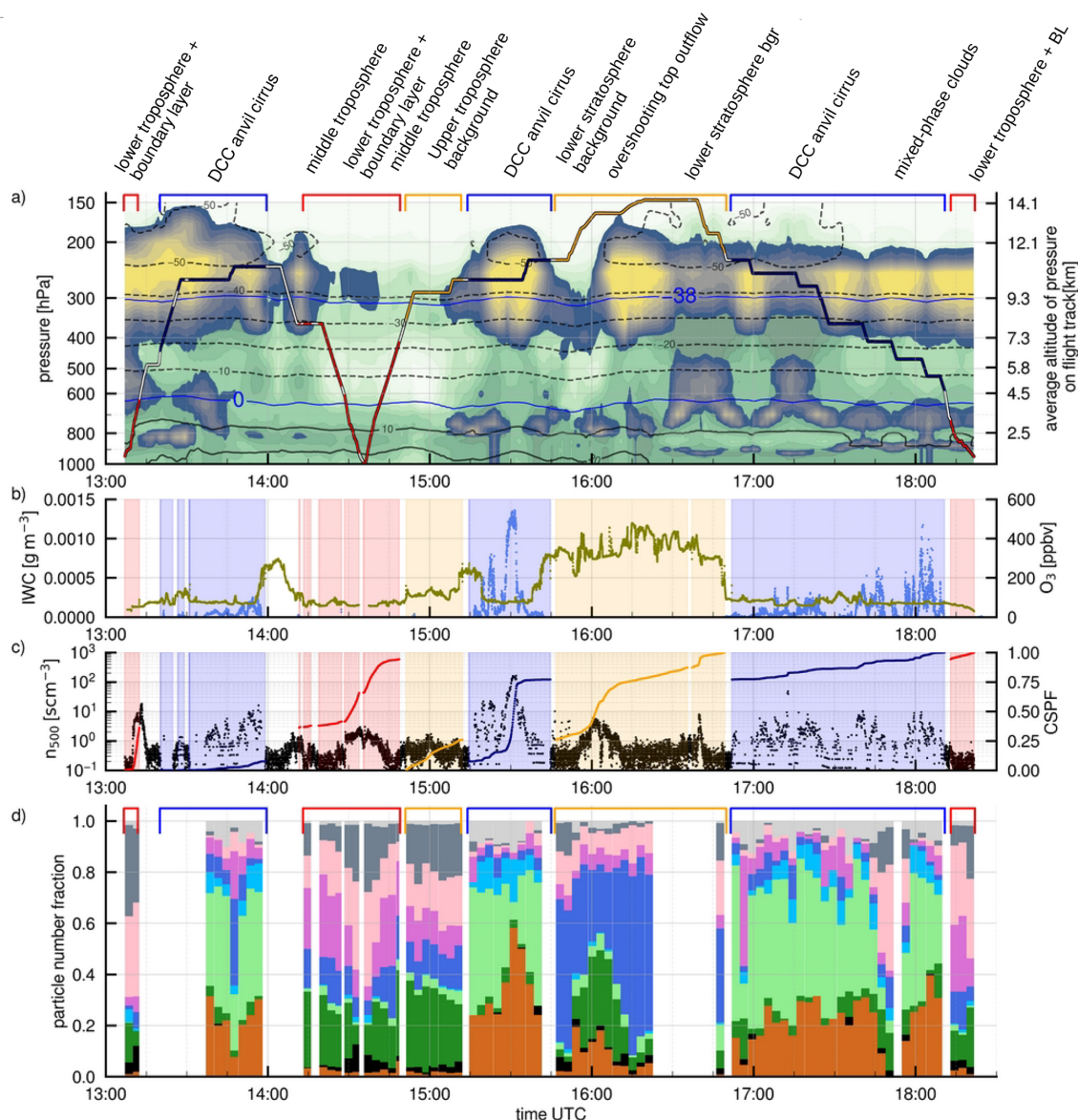
Figure 4. Multi panel time series (UTC) with a flight cross section of F15 in the top panel (a). The colored lines indicate the flight altitude and HERA filter position (orange, blue, red). In the background are ERA5 reanalysis vertical cross section along the flight path. Green contours show relative humidity with respect to liquid water while blue/yellow contours show cloud cover. Isotherms are marked with black lines. While all data is plotted on pressure levels, the right-hand axis indicates the average altitude of the pressure level on the flight track. For more precise height information of the flight track, see Fig. S10c. Panel (b) shows ice water content (IWC, blue) calculated from the Cloud Combination Probe (CCP, De La Torre Castro et al., 2023) and ozone trace gas concentrations (olive green, Zahn et al., 2012). Panel (c) shows concentration of large aerosol particles. The shaded background area marks filter sampling section analogous to the top panel color coding. Outside clouds, measurements of aerosol particle concentrations ( d > 500 nm, n_{500} ) are shown. Inside cloud (blue shaded areas), CPR concentrations ( n_{500} , enrichment factor not accounted for) are shown, measured by the ALABAMA OPC. The colored lines (same sample color coding) corresponds to the right hand axis and indicate the cumulative sampled particle fraction (CSPF) of n_{500} for each filter sample. Panel (d) shows the particle number fraction separated into 10 categories using the dominant mass spectra component as measured by the ALABAMA. The clamps above mark the simplified HERA sampling sections. White sections indicate either very low number of detected particles ( < 30 \text{ min}^{-1} ) or the ALABAMA not being connected to the same aircraft inlet as HERA.
