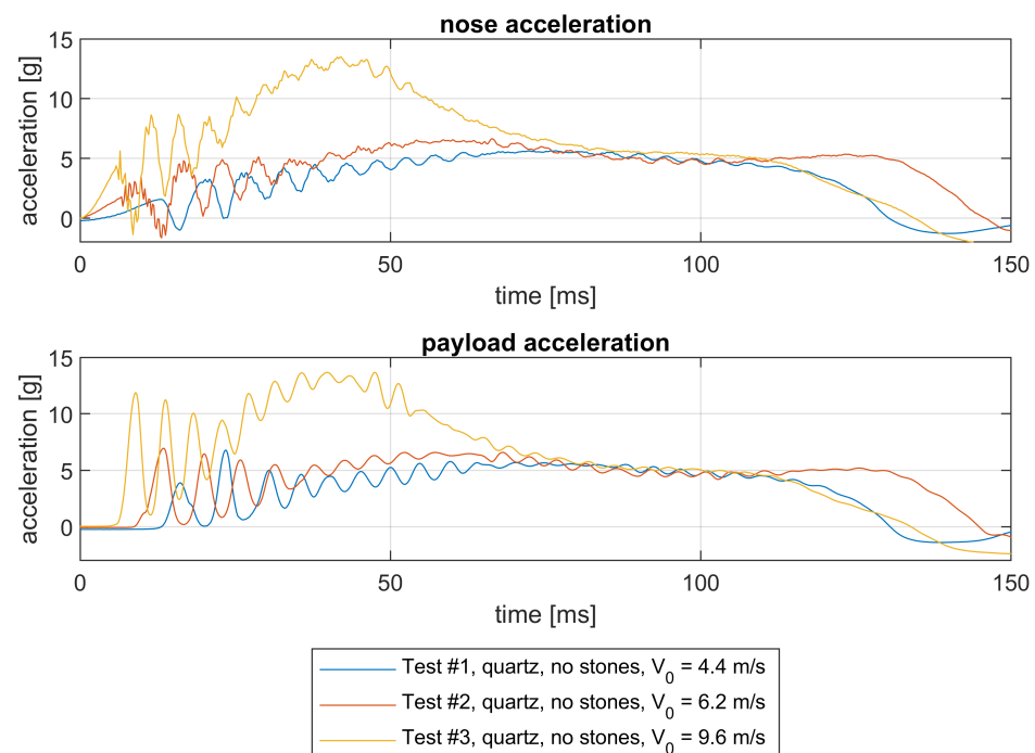
Figure 16. Acceleration data of test #1, #2, and #3. Quartz soil without any stones was used.
