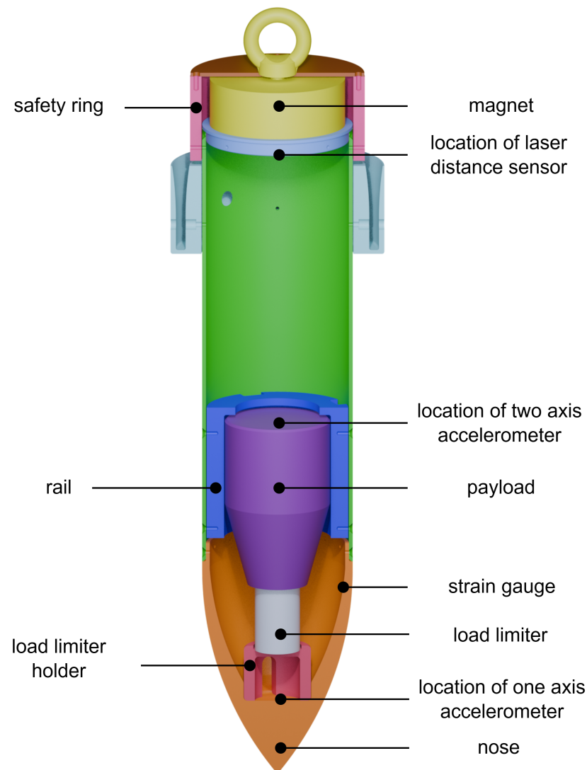
Figure 13. Cross-section view of the test penetrator.
