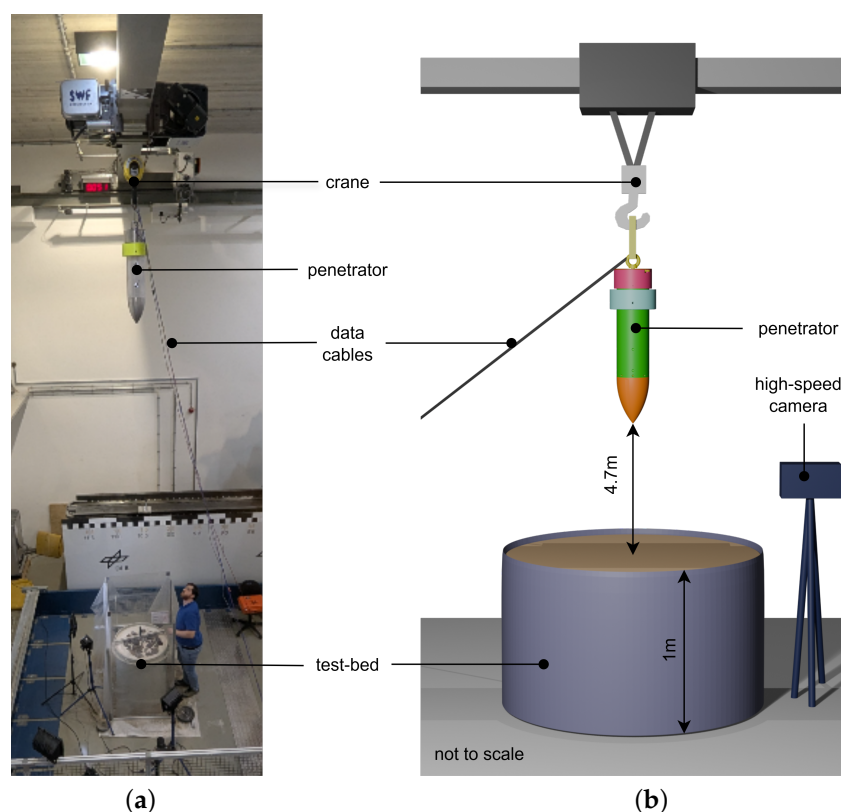
Figure 14. Implemented (a) and planned test setup (b).
