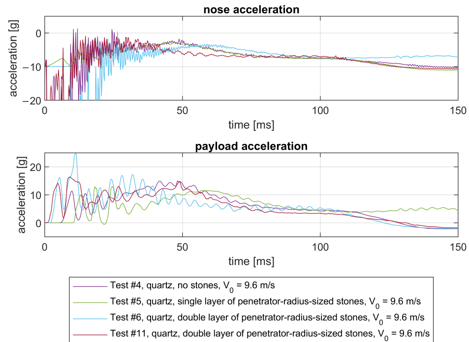
Figure 19. Acceleration data of tests #4, #5, #6, and #11. Test #11 is repetition of Test #6.
