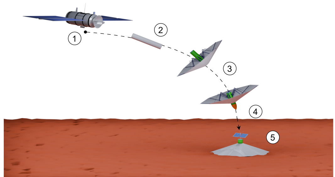
Figure 1. Concept of operations of the micro Mars lander concept.
