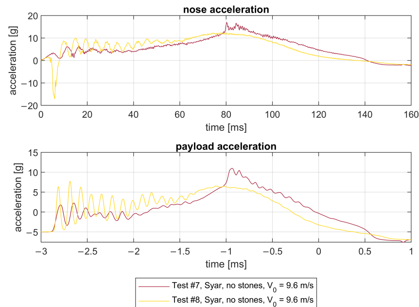
Figure 21. Acceleration data of test #7 and #8.
