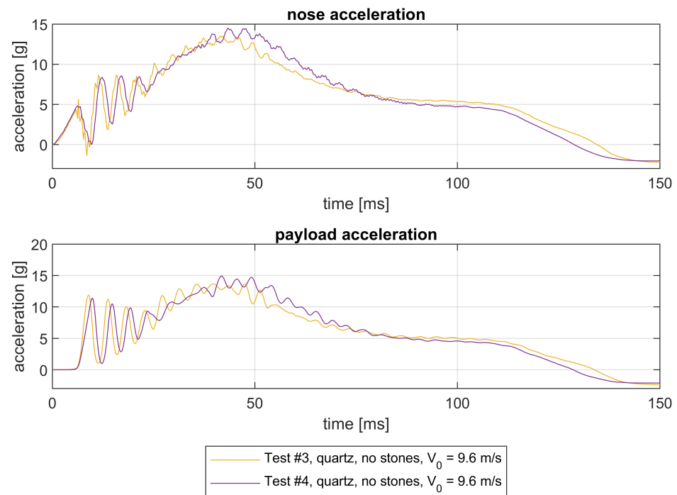
Figure 17. Acceleration data of tests #3 and #4.
