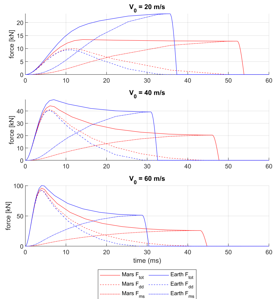
Figure 11. A comparison of the effects of Mars and Earth gravity on F_{tot} , F_{ms} and F_{dd} for impact velocities of 20 m/s, 40 m/s, and 60 m/s.
