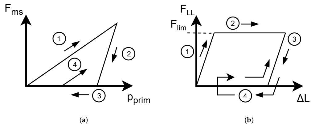
Figure 7. (a) elastic-plastic force law and (b) force–displacement behavior of the load limiter (cases are shown in Table 4). Both are modified schematics by Witte et al. [36].
