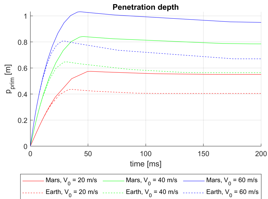
Figure 12. A comparison of the effects of Mars and Earth gravity on penetration depth for impact velocities of 20 m/s, 40 m/s, and 60 m/s.
