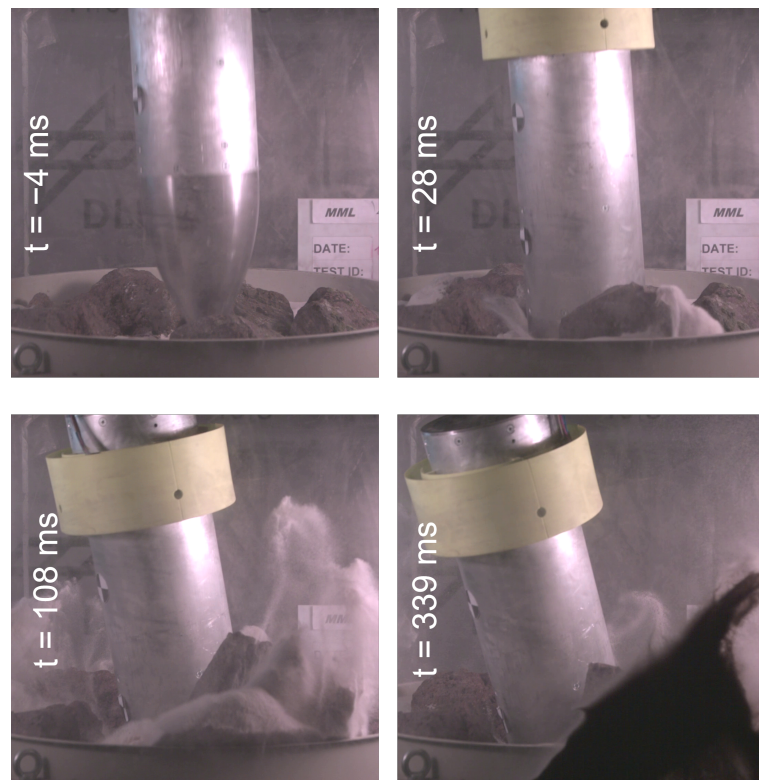
Figure 28. Screenshots taken from the high-speed video of test #13. The impact begins at t = 0 ms with V_0 \approx 9.6 m/s.
