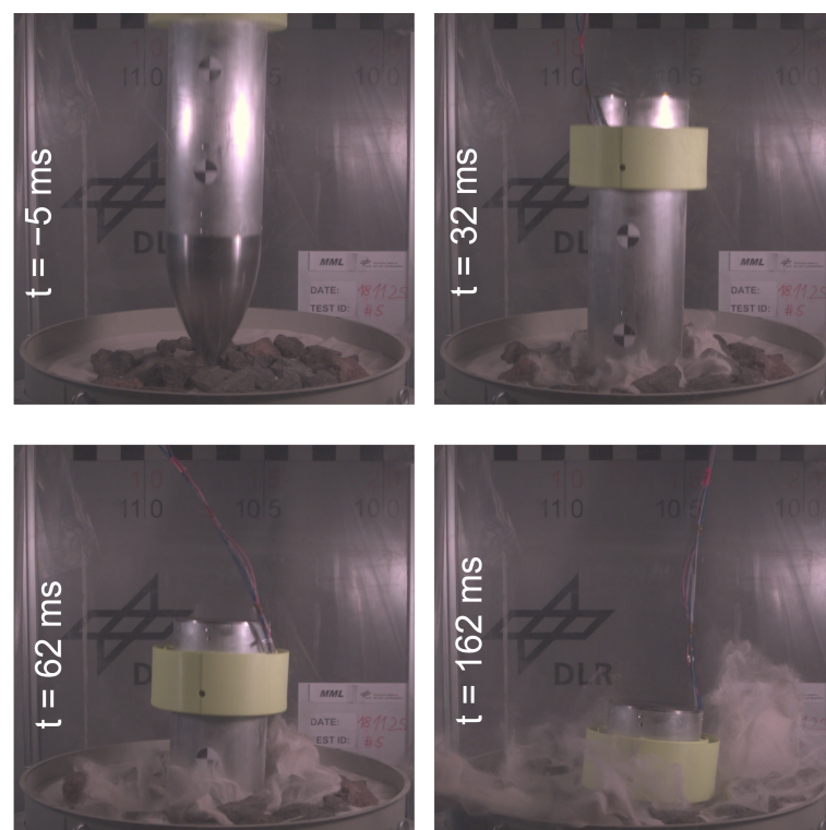
Figure 20. Screenshots taken from the high-speed video of test #5. The impact begins at t = 0 ms with V_0 \approx 9.6 m/s.
