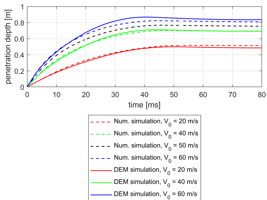
Figure 10. The displacement of penetrator over time during the penetration process by the discrete element method and numerical simulation.
