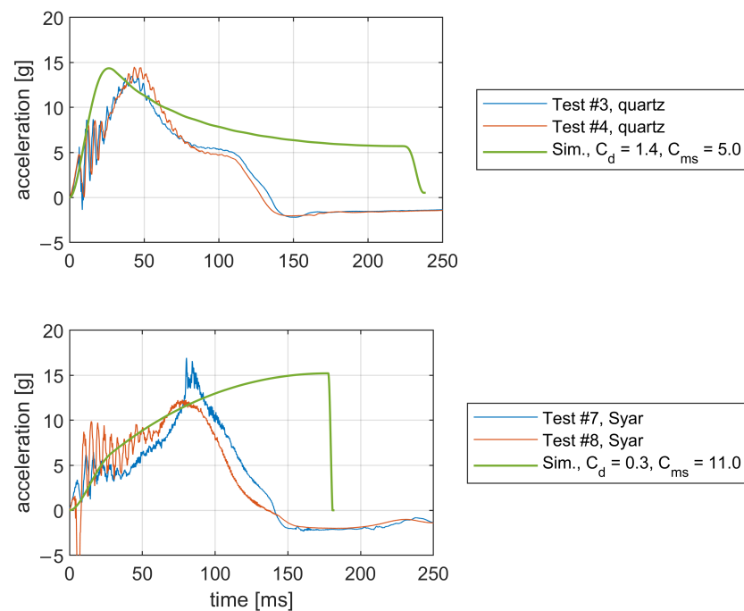
Figure 29. Simulated and measured acceleration profiles for Syar and quartz sand.
