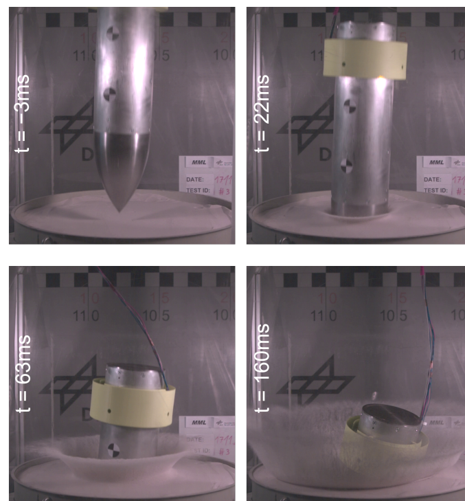
Figure 18. Screenshots taken from the high-speed video of test #3. The impact begins at t = 0 ms with V_0 \approx 9.6 m/s.
