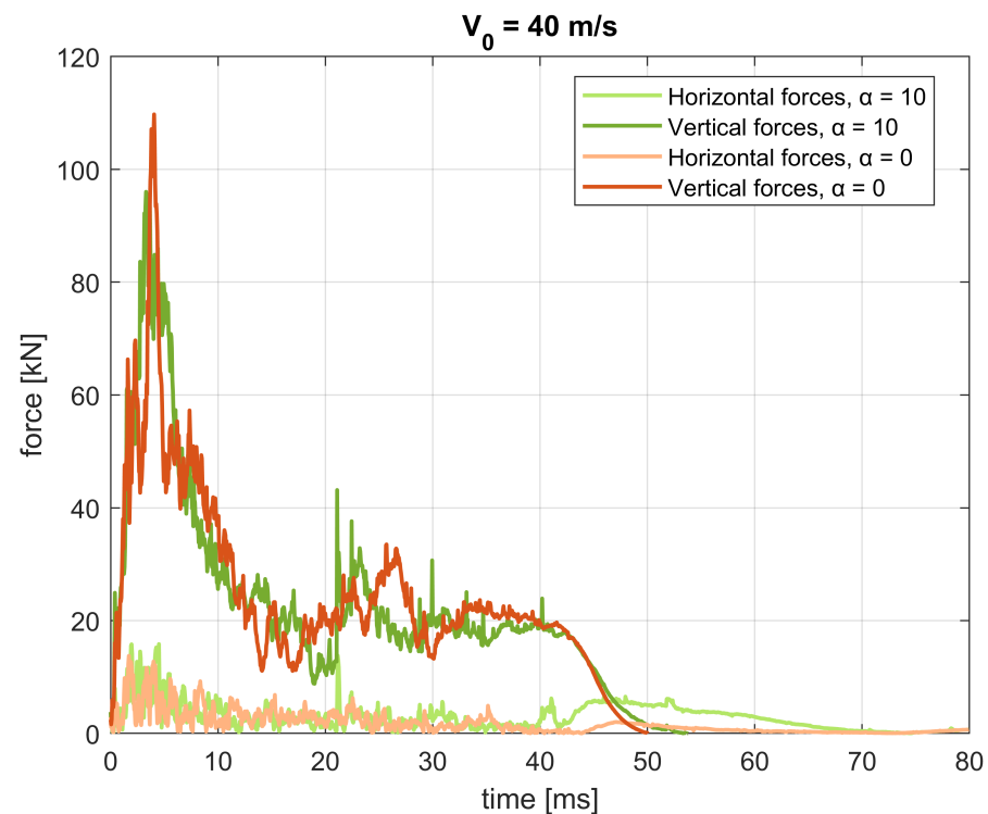
Figure 5. A comparison of the vertical and horizontal force response between an angle of attack of 0^\circ and 10^\circ with V_0 = 40 m/s.
