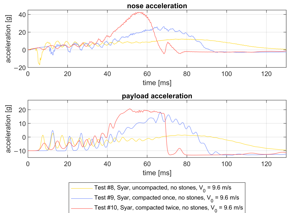
Figure 22. Acceleration data of tests #8, #9 and #10.
