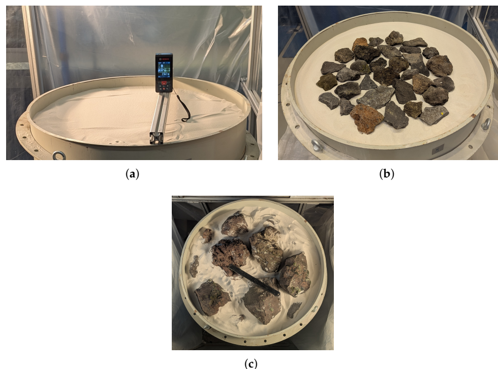
Figure 15. Test-bed setup variants. (a) WF 34 without any stones and measuring setup for the drop height. (b) WF 34 with a single layer of penetrator-radius stones. (c) Penetrator-diameter-sized stones.
