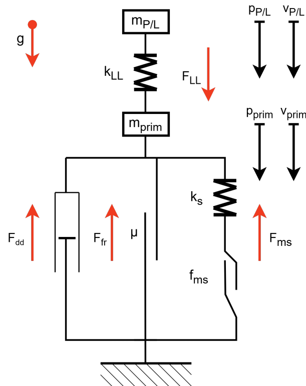
Figure 6. Force model of the semi-empirical penetration simulation.
