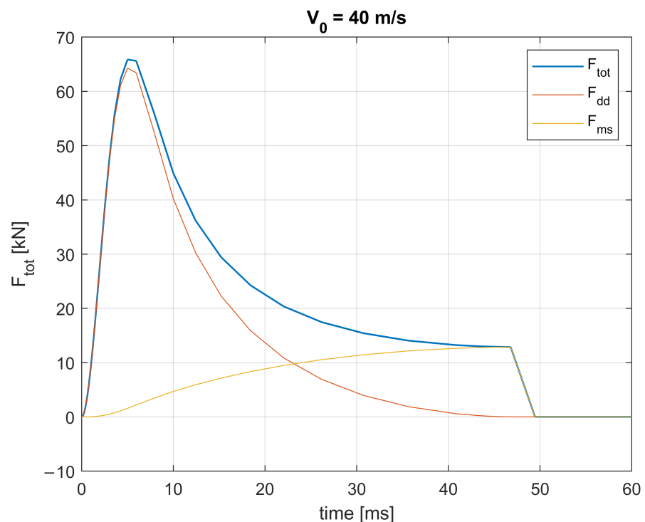
Figure 8. Breakup of the total Force F_{tot} into the displacement drag F_{dd} and mechanical strength F_{ms} according to the numerical simulation. The penetrator impacts with a velocity of V_0 = 40 m/s.
