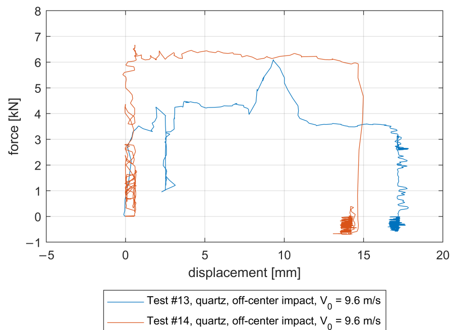
Figure 27. Force–displacement diagram of the load limiter during tests #13 and #14.
