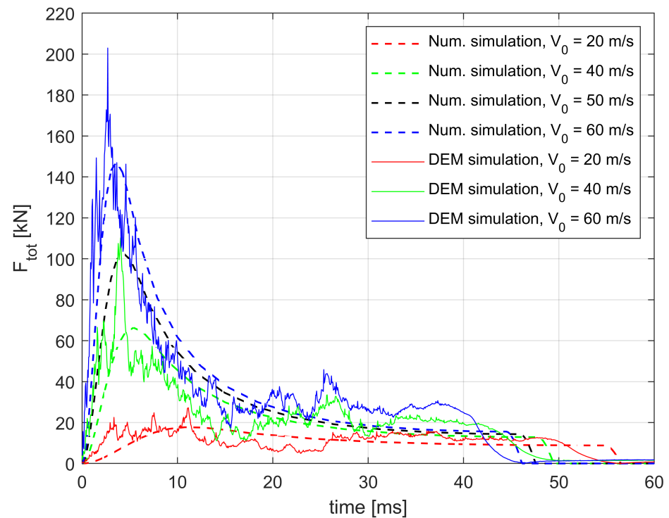
Figure 9. The magnitude of the force acting on the penetrator over time during the penetration process by the discrete element method simulation and numerical simulation.
