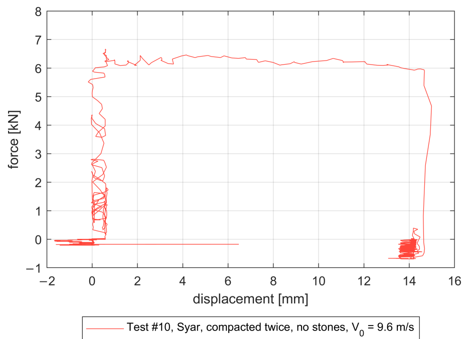
Figure 23. Force-displacement diagram of the load limiter during test #10.
