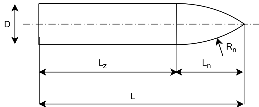
Figure 2. Dimensions used to describe the dimensions of the penetrator. The values are shown in Table 1. The nose has the shape of a tangent ogive.
