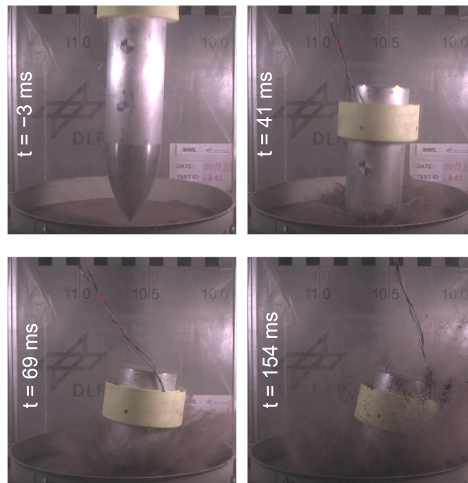
Figure 24. Screenshots taken from the high-speed video of test #10. The impact begins at t = 0 ms with V_0 \approx 9.6 m/s.
