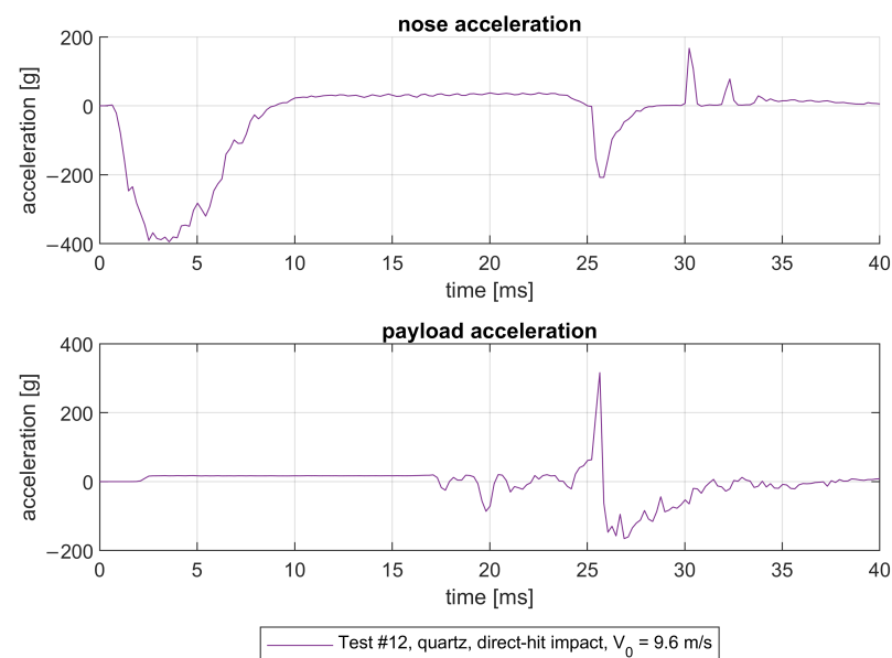
Figure 25. Acceleration data of test #12.
