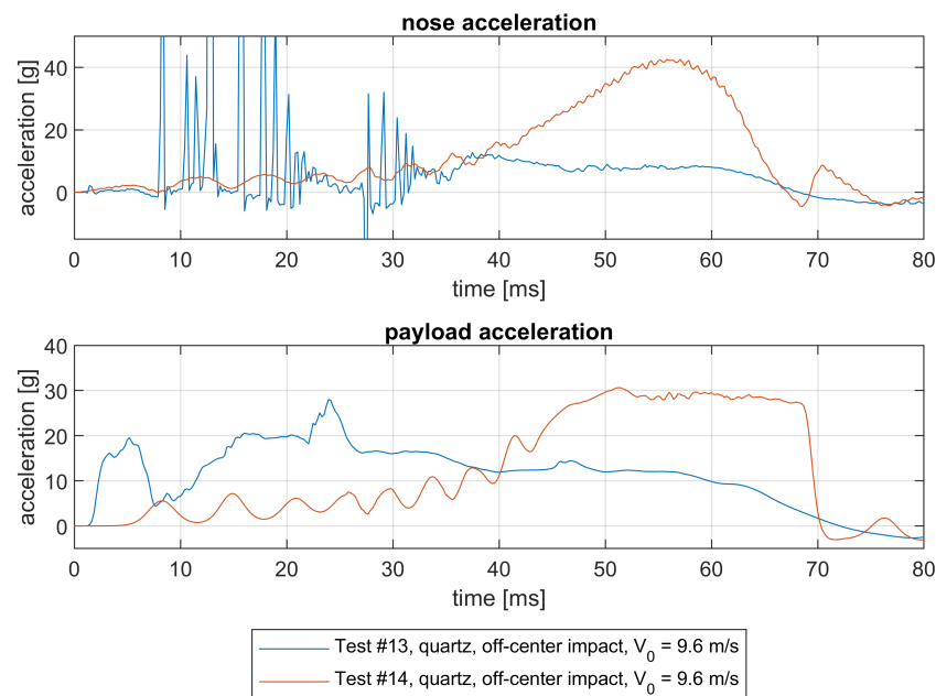
Figure 26. Acceleration data of test #13 and #14.
