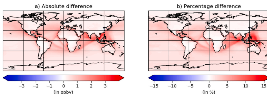
Fig. A1. a) Absolute and b) Percentage difference in the annual mean surface ozone simulated in NoSNPm-Base and No-tag-Base simulations. This difference illustrates the effect of exclusion of SNPm in the EMEP simulations and quantifies the range in the upper and lower limits of the effect of NO x emitted from ships on surface ozone mixing ratio.
