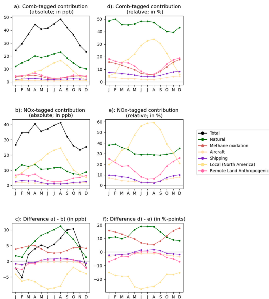
Fig. 6. All quantities shown here are seasonal cycles simulated over NE US. For the results over other receptor regions, see supplementary figures as indicated in the brackets next to the panel description in this text. These supplementary figures also show the disaggregated contributions to the Natural, Remote Land Anthropogenic and Shipping components for all receptor regions analysed in our study. a) (S9-S11) Surface ozone and its contributing tagged components simulated in the Comb-tag-Base simulation ( O_3^{\text{Tag(Comb)}} ) (in ppbv). b) (S2-S4) Surface ozone and its contributing tagged components simulated in the NO x -tag-Base simulation ( O_3^{\text{Tag(NOxT)}} ) (in ppbv). c) (S15-S17) Difference between the quantities (in ppbv) shown in a) and b). d) (S12-S14) Relative contribution of the tagged components to total ozone simulated in the Comb-tag-Base simulation (in %). e) (S5-S7) Relative contribution of the tagged components to total ozone simulated in the NO x -tag-Base simulation (in %). f) (S18-S20) Difference between the quantities (in %-points) shown in d) and e).
