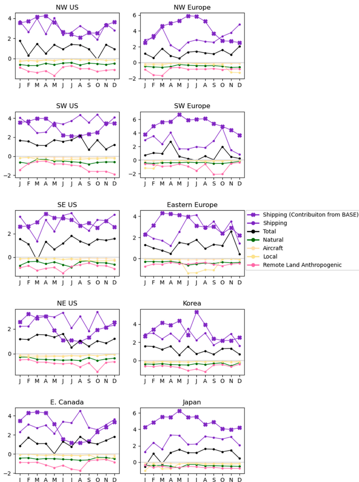
Fig. 9. Scaled responses of surface ozone and various NOx-tagged components (in ppb) to the Ship perturbation ( O_3^{TAG(Pert-NOxT)} ). The responses are shown over the receptor regions considered in our study. Also shown is the ship-tagged component in the NOx-Tag-Base simulation (purple line with crossed marker: O_3^{SHP(NOxT)} ). Note that the “Local” and “Remote Land Anthropogenic” components are different for each of the receptor regions (Eg: Local component for European receptor regions is the Europe tag; Remote Land Anthropogenic component is the sum of all land region tags in Fig. 1b other than Europe). See Supplementary Figs. S21–S23 for the disaggregated contributions to the natural, remote land anthropogenic and shipping components shown here.
