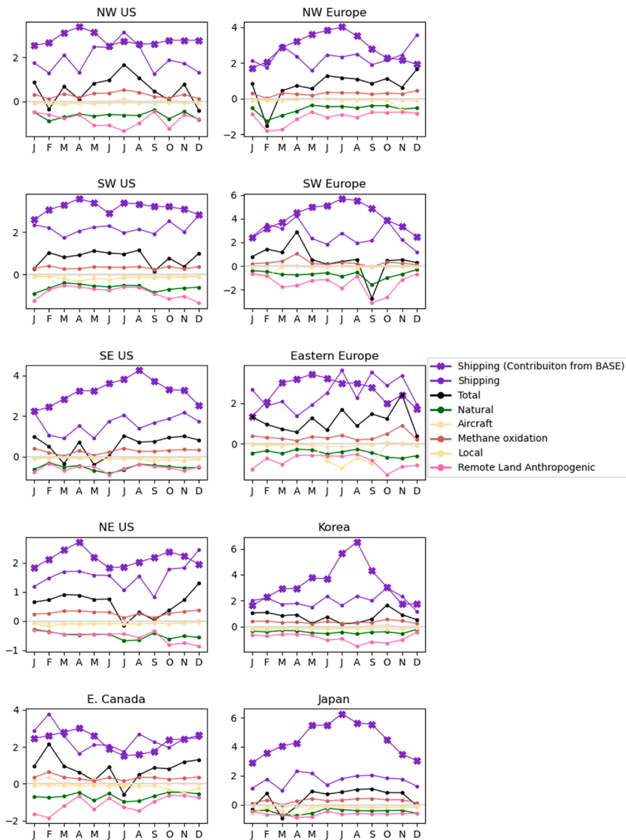
Fig. 10. Same as Fig. 9 but for Combined-tagged components. Also shown is the ship component in the Comb-Tag-Base simulation (purple line with crossed marker: O_3^{SHP(Comb)} ). See Supplementary Figs. S24–S26 for the disaggregated contributions to the natural, remote land anthropogenic and shipping components shown here.
