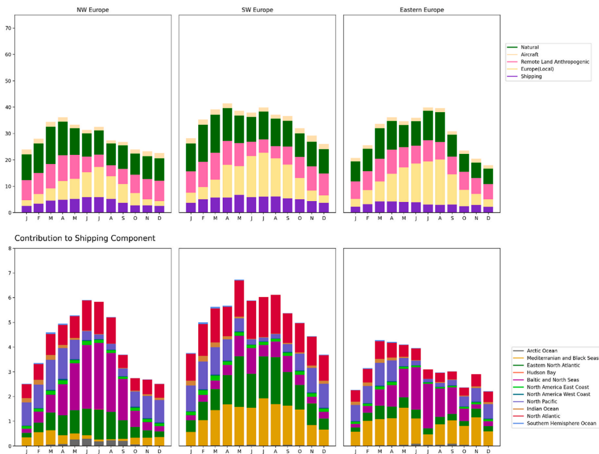
Fig. 4. Same as Fig. 3 but for European receptor regions (in ppbv). See supplement for the detailed contributions from various tags within the “Natural” and “Remote Land Anthropogenic” components shown here (Fig. S3) and the relative contributions (in %) of the tags to the total surface ozone.
