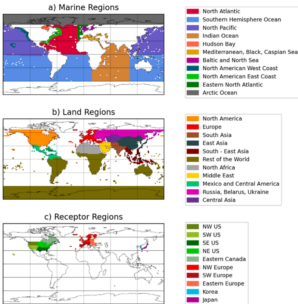
Fig. 1. a) Marine regions whose ship emissions to which our simulated ozone (see Table 1) is attributed. See Supplementary Fig. S1 for the magnitude of NO x emissions from these marine regions used in our study. b) Land regions whose anthropogenic precursor emissions to which ozone is attributed in our tagged simulations. Here we aggregate the tags as local/remote land regions based on the receptor region over which the model output is analysed. See supplement for the disaggregated contribution from these land regions. c) Receptor regions over which the simulated surface ozone is evaluated (section 2.2) and analysed (section 3) in our study.
