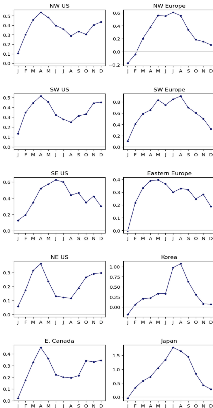
Fig. A2. Same as Fig. A1a but shown as a surface ozone seasonal cycle (in ppbv) and averaged over receptor regions shown in Fig. 1c.
