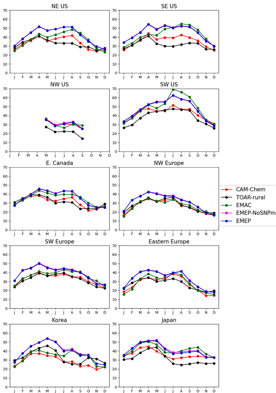
Fig. 2. Evaluation of surface ozone (in ppbv) simulated in the Base simulations (NO x -tag-Base (CESM; red), Comb-tag-Base (EMAC; green), No-tag-Base (EMEP; blue), and NoSNPm-Base (EMEP-NoSNPm; magenta)) of our study against gridded observations from TOAR dataset (rural only; black). Shown are the mean surface ozone fields over various HTAP Tier 2 regions and only over grid cells and during the months where/when the TOAR rural data is available. See Supplementary
