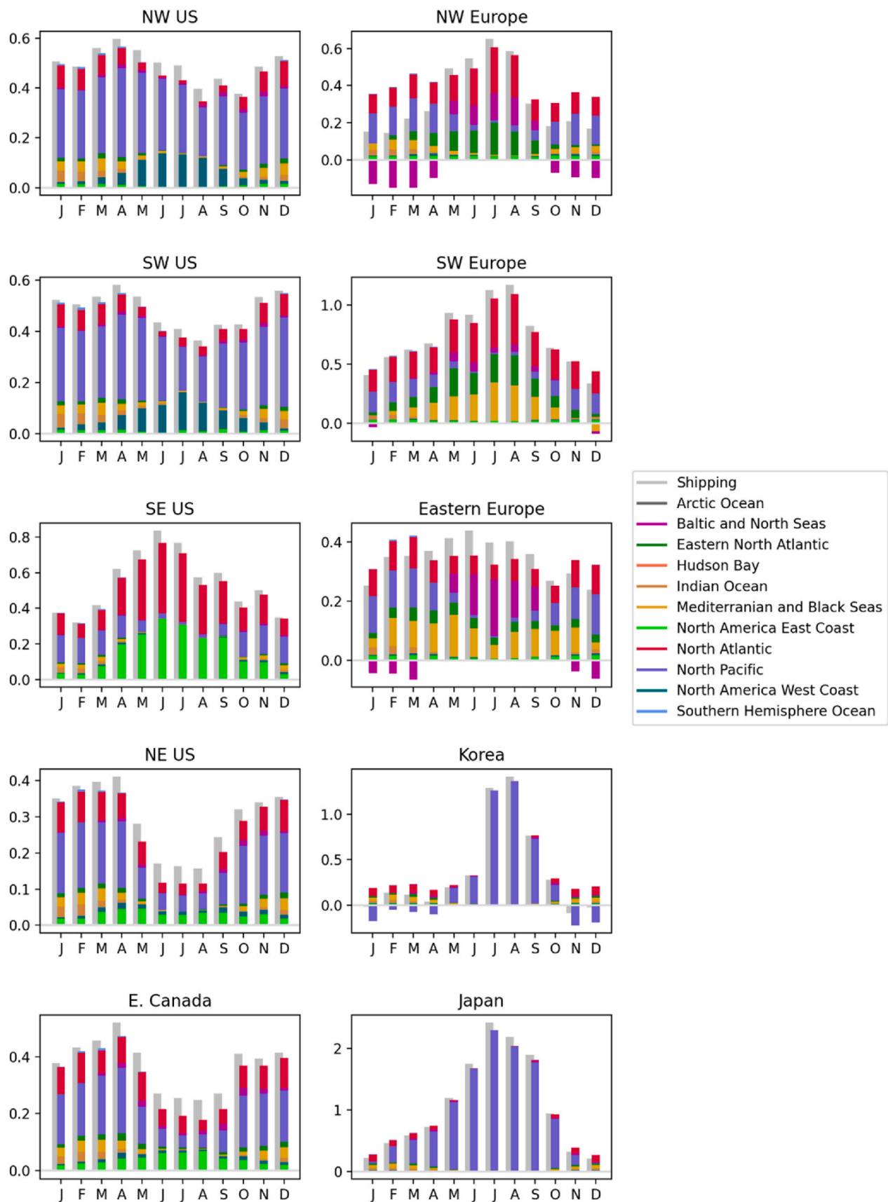
Fig. 7. Scaled responses to ship NO x perturbation (in ppbv) over various marine regions (see Fig. 1a) simulated by EMEP model, shown as coloured stacks representing the scaled responses to ship NO x perturbation over individual marine regions ( O_3^{Mreg(Pert)} ), calculated as explained in section 2.1.3. Also shown is the scaled response to perturbation in ship NO x over all marine regions simultaneously (grey bar adjacent to the coloured stacks: O_3^{SHP(Pert)} ). Responses are shown over all the receptor regions considered in our study (Fig. 1c).
