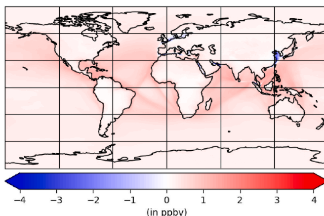
Fig. A3. Difference in the annual mean scaled response in surface ozone to all marine region NO x perturbation simulated without and with SNPm included ( O_3^{NoSNPm(Pert)} - O_3^{Ship(Pert)} ).
