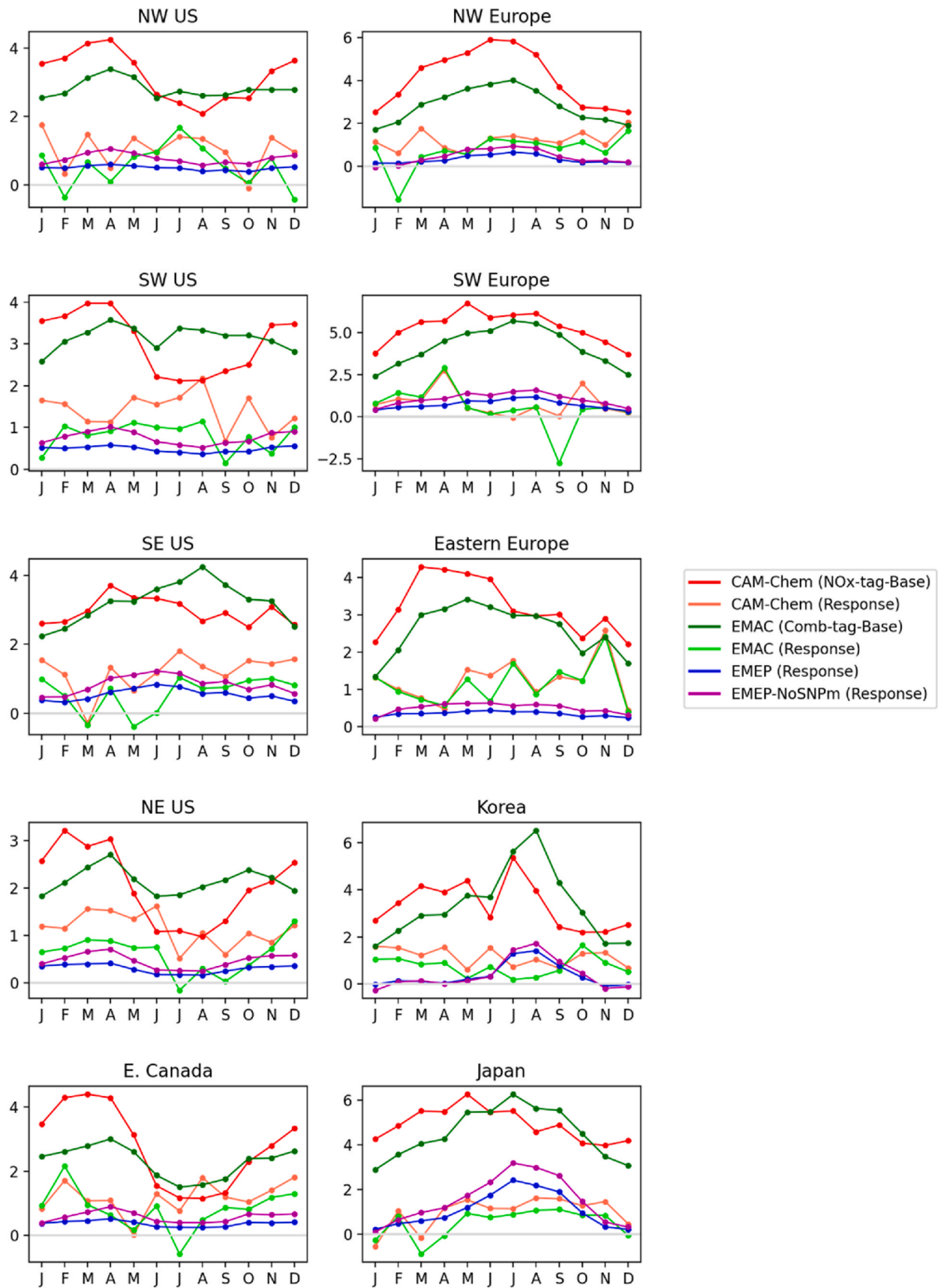
Fig. 8. Seasonal cycle in the tagged absolute contributions from the shipping component to the total surface ozone (in ppbv) in the NO x -tag-Base (Dark Red line: O_3^{SHP(NOxT)} ) and Combined-tag-Base (Dark Green line: O_3^{SHP(Comb)} ) simulations over the regions considered in our study. Also shown are the scaled responses to ship-NO x perturbations (orange line: O_3^{TOT(Pert-NOxT)} , light green line: O_3^{TOT(Pert-NOxT)} , blue line: O_3^{SHP(Pert)} and magenta line: O_3^{NoSNPm(Pert)} ) in each of the models considered in our study.
