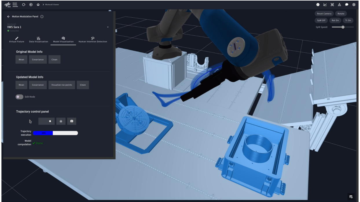
Fig. S8. Model Visualization tab during trajectory execution. The trajectory control panel shows the execution progress, and the digital twin of the robot moves in sync with the real robot.
