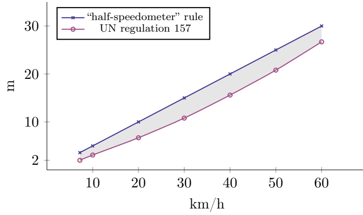
Figure 5.8: Safety distances according to the “half-speedometer” rule and the UN regulation 157, with the gray zone highlighted in between.
