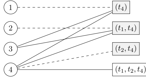
Figure 5.9: The bipartite graph G_S for the four scenarios of Example 5.4.3 . The left partition represents the sets S_1 to S_4 , and the right partition contains their elements. The maximum matching is given as dashed lines.
