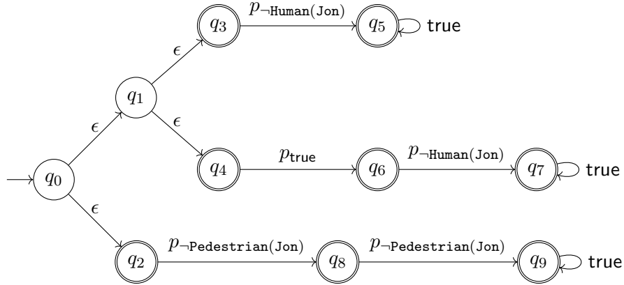
Figure 4.6: The nondeterministic replacement FA A_{\text{PA}(\text{FTN}(\Phi_{ex}(\text{Jon}), 2))} .
