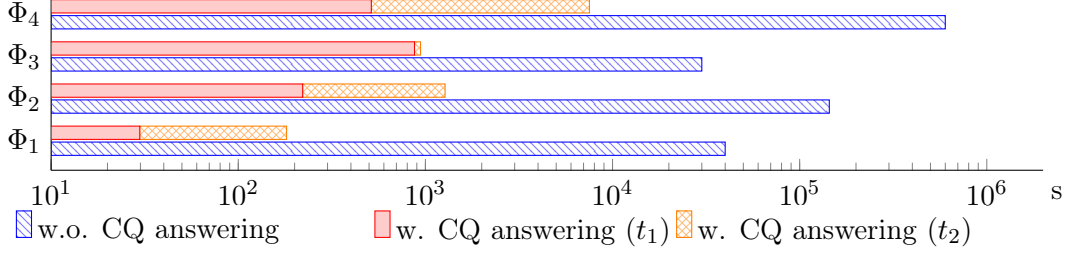
Figure 5.6: Log-scaled run times of Algorithm 1 with and without the CQ answering optimization enabled for the TOBM T-crossing S = 0, N = 3 . Run times without the optimization are extrapolated after one hour. The times spent in the first ( t_1 ) and second run ( t_2 ) are additionally given for the optimized implementation.
