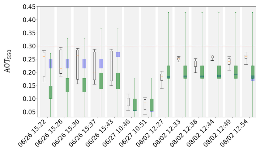
Fig. 10. Comparison of AOT_{550} estimates. Black: distribution of EmSFNN AOT_{550} estimates in single HyPlant acquisitions, box width show 25–75 % percentiles and whiskers show 5–95 % percentiles, the median is reported in orange, Blue: CIMEL measurements of the JOYCE AERONET station (FZJ-JOYCE, 2024) located at ~5 km from the SEL-2018 HyPlant acquisitions (left), box width shows the standard deviation of all measurements recorded within 20 min of the HyPlant acquisition time, Green: Deep Blue AOT_{550} products of MODIS Terra (MODIS Atmosphere Science Team, 2017a) and Aqua (MODIS Atmosphere Science Team, 2017b) at 10 km resolution, box width shows the standard deviation of available Terra and Aqua products within two hours of the HyPlant acquisition time and the whiskers represent the mean of the provided uncertainty of the estimates within a 30 km window around the location of the CKA-2020 estimates. Red: maximum AOT_{550} covered in simulation database. (For interpretation of the references to colour in this figure legend, the reader is referred to the web version of this article.)
