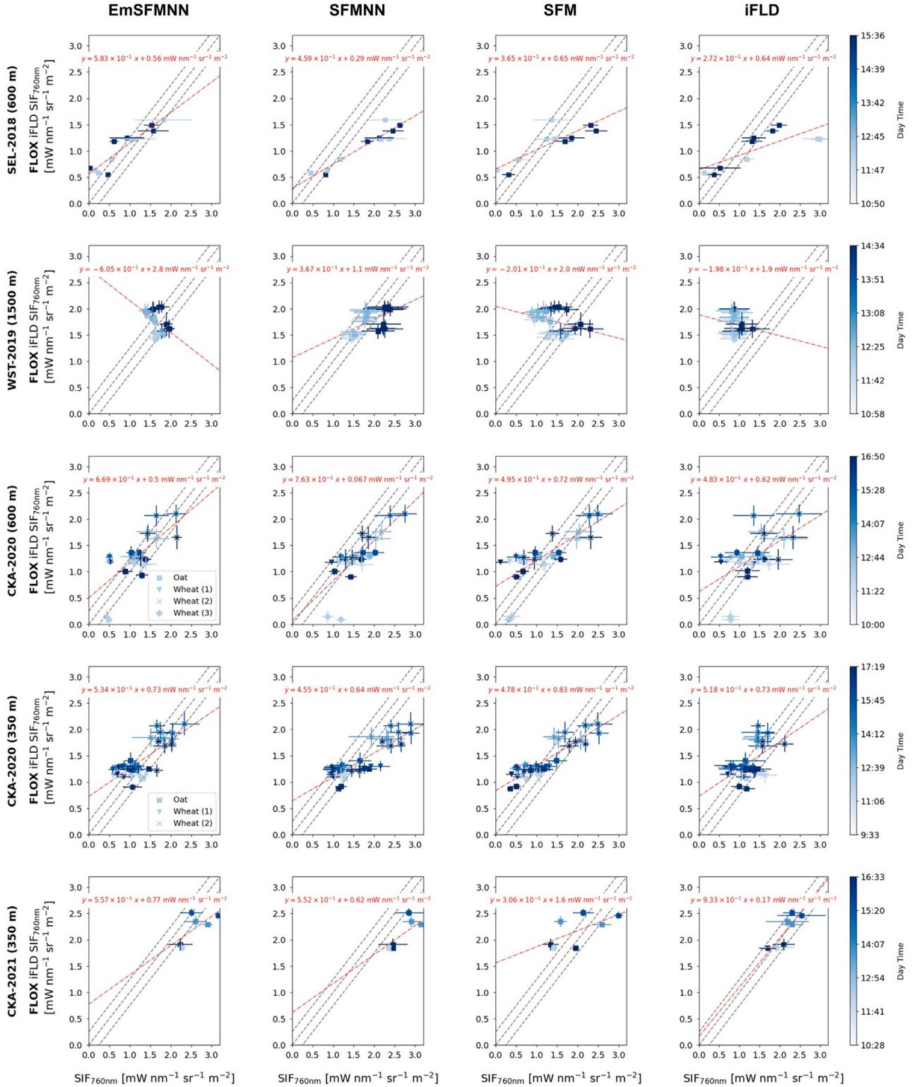
Fig. 6. FLOX-derived iFLD SIF vs. HyPlant-derived EmSFNN, SFMNN, SFM and iFLD SIF in the five in-situ validation data sets (see Table 1). The dashed line and the red floating labels report the linear relationship between airborne and in-situ FLOX iFLD estimates. In the CKA-2020 data sets FLOX measurements from different devices are reported separately. The x-axes of the subplots are shared and labelled at the bottom. (For interpretation of the references to colour in this figure legend, the reader is referred to the web version of this article.)
