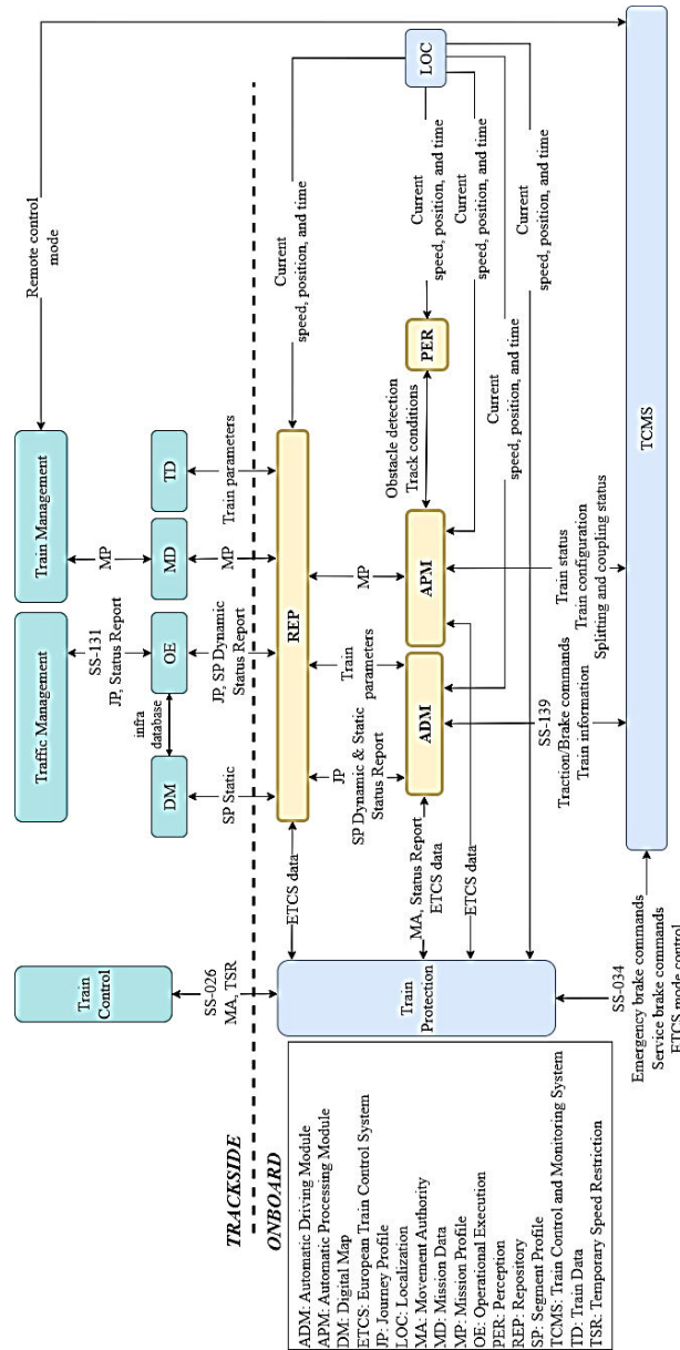
Figure 22.1 ATO up to GoA 4 - Logical reference architecture [11].
