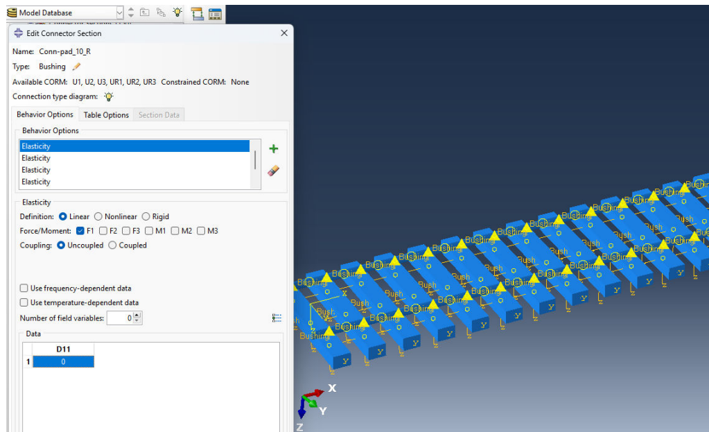
Figure 6.6 Track model in Abaqus (straight segment)
