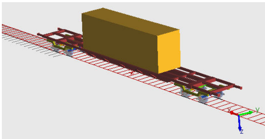
Figure 6.7 MBS model (track and vehicle)
