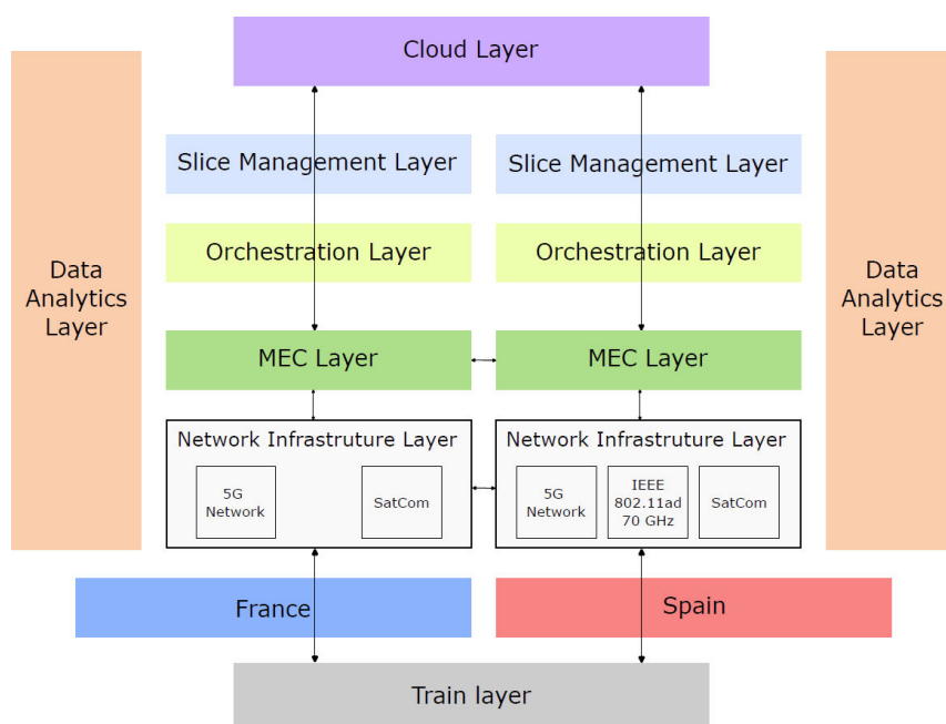
Figure 9.2: 5GMED Architecture [19]
