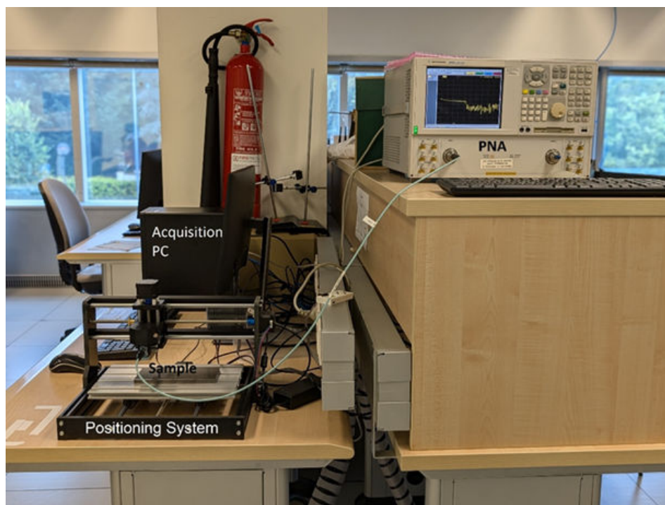
Figure 18.3 Experimental setup
