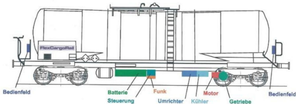
Figure 15.2 Representation of the components under the wagon body [6]
