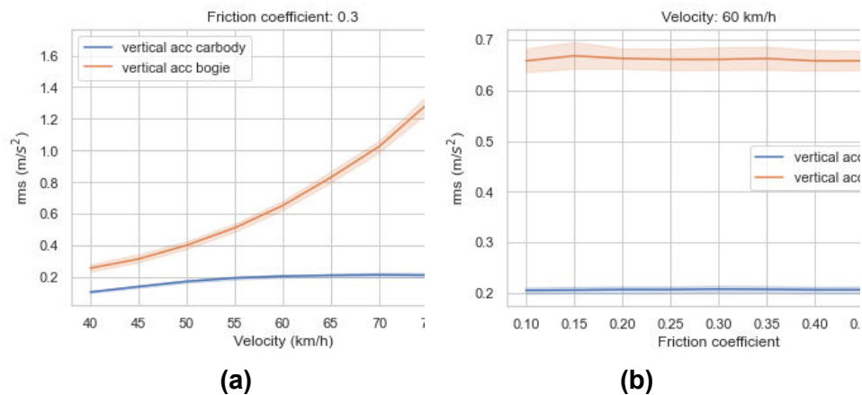
Figure 7.3: (a): Vertical acceleration measured in carbody and bogie frame for different running speeds. (b): Vertical acceleration in carbody and bogie frame for different friction coefficient values.
