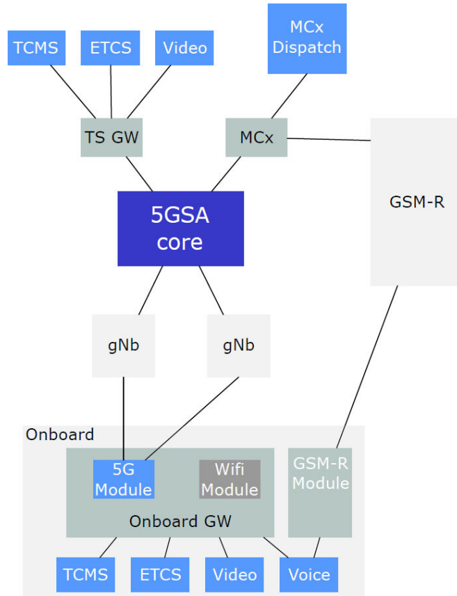
Figure 9.1: 5GRAIL lab test network configuration [16]
