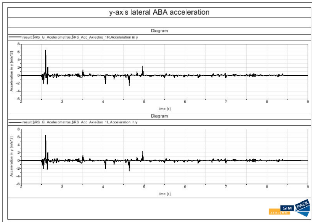
Figure 6.8 Simpack Post synthetic ABA data graph
