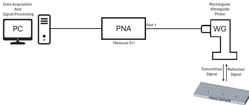
Figure 18.2 Schematic diagram of the measurement setup.
