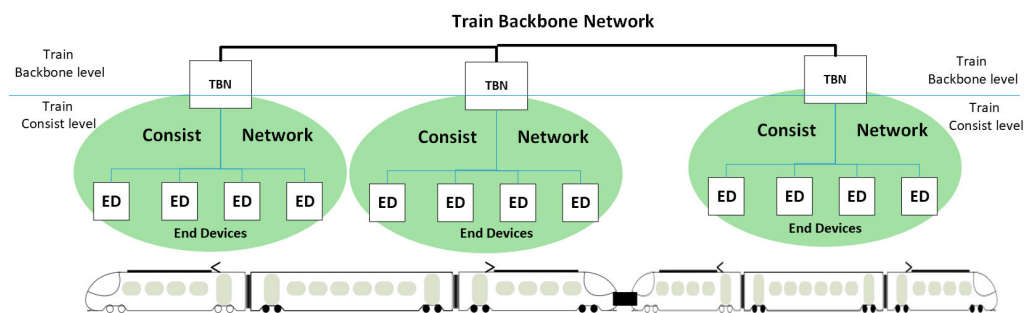
Figure 5.1 Wired TCN Architecture
