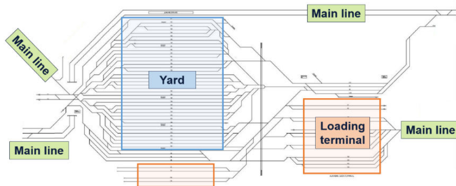
Figure 11.1 The Alnabru terminal has a loading terminal next to the yard (Bane NOR, 2024)
