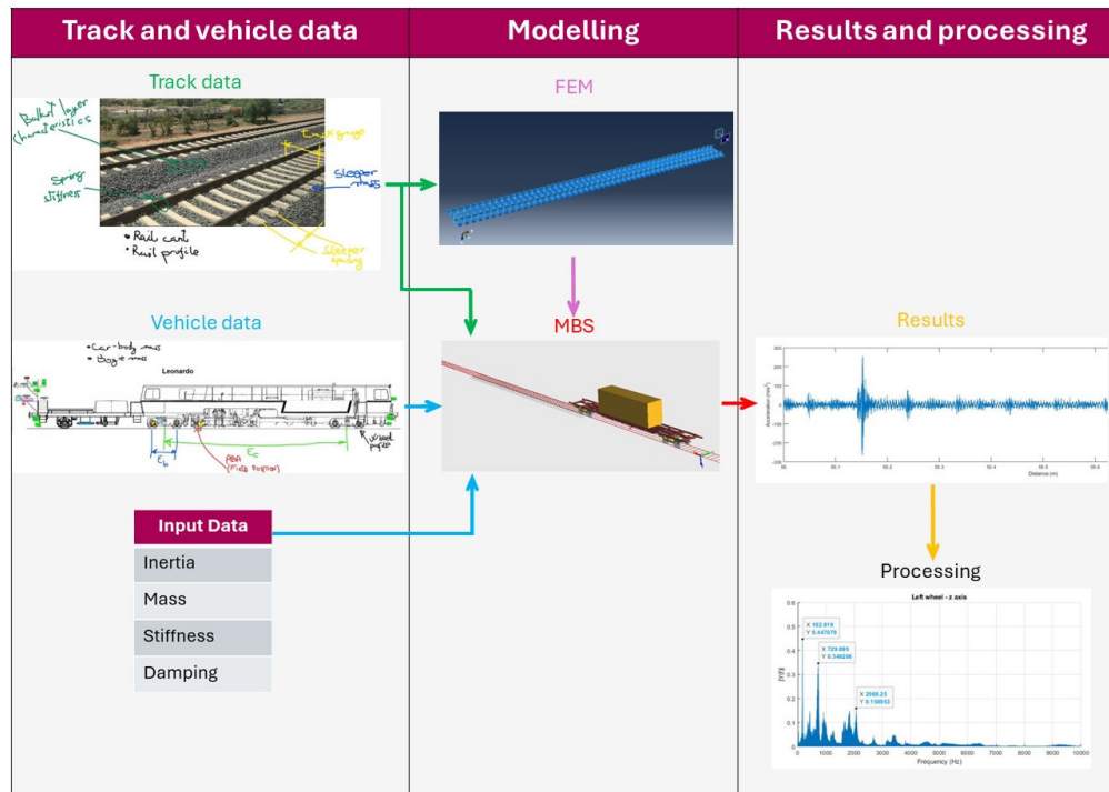
Figure 6.5 Workflow of the virtual model creation
