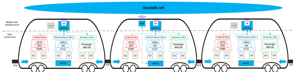
Figure 5.3: 5G Network Slicing in wireless Train backbone Network
