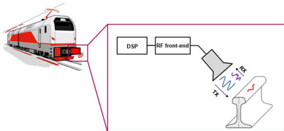
Figure 18.1 Railway inspection using microwaves
