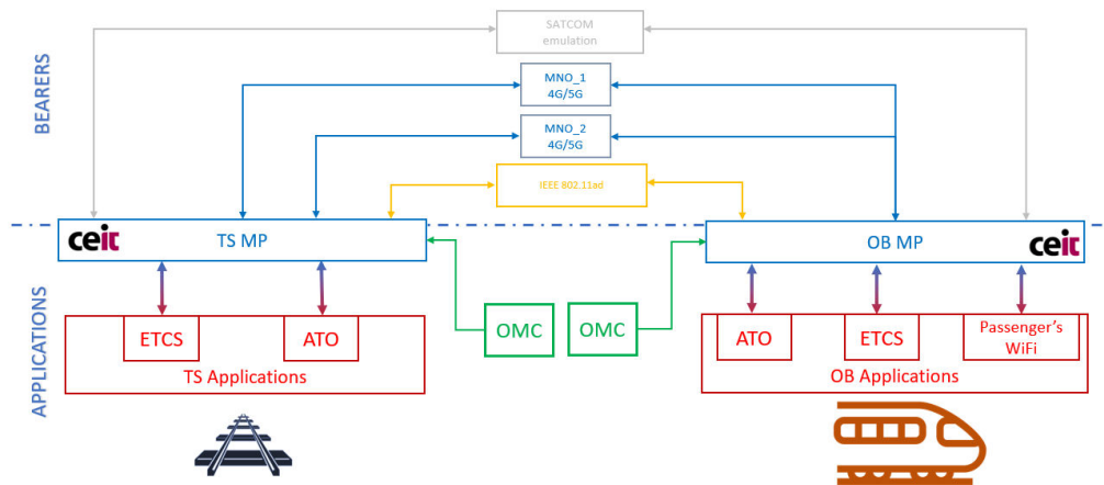
Figure 9.4 CEIT Multi-connectivity platform diagram
