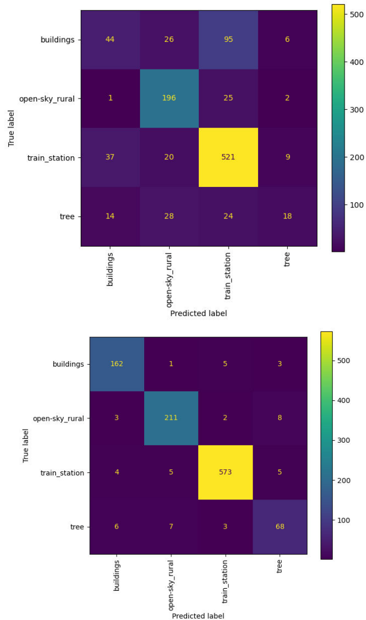
Figure 20.4 Confusion matrix for Multi-class Logistic Regression (above) and XGBoost (below)
