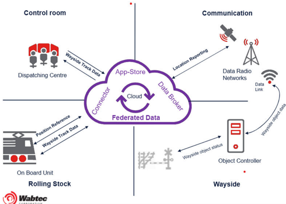
Figure 13.2 G2 regional lines high level architecture
