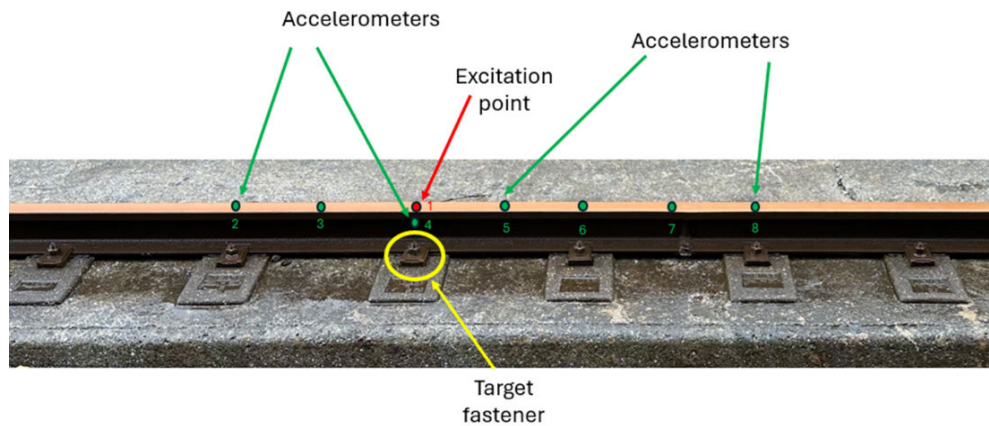
Figure 6.2 Designed hammer test layout to be applied
