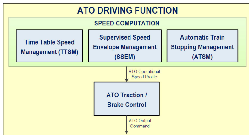
Figure 10.3 Schematic speed calculation process defined in the SUBSET-125 [15].
