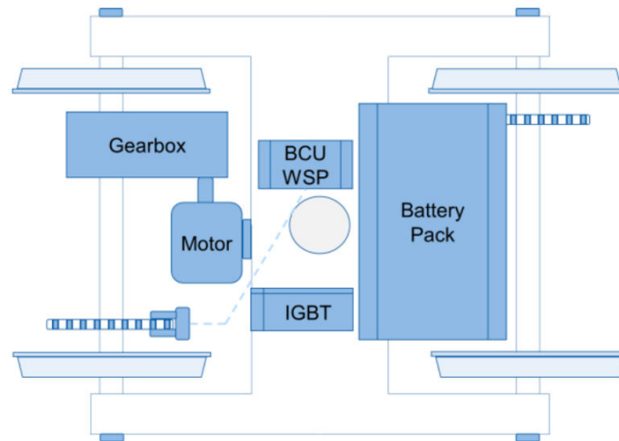
Figure 17.4 Conceptual layout of a fully-integrated self-propelled bogie, with all necessary systems for converting a conventional wagon to an SPFW, including a brake control unit (BCU) and wheel slide protection (WSP) [2]
