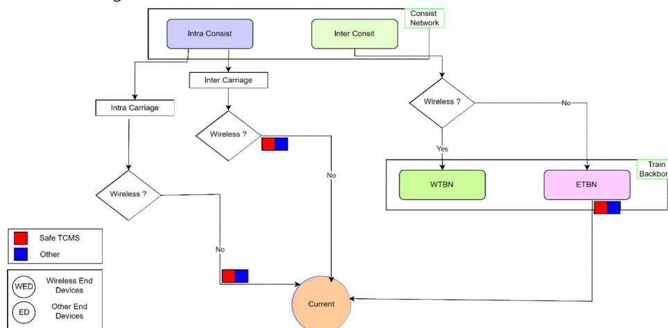
Figure 4.4 Current TCN usage case
