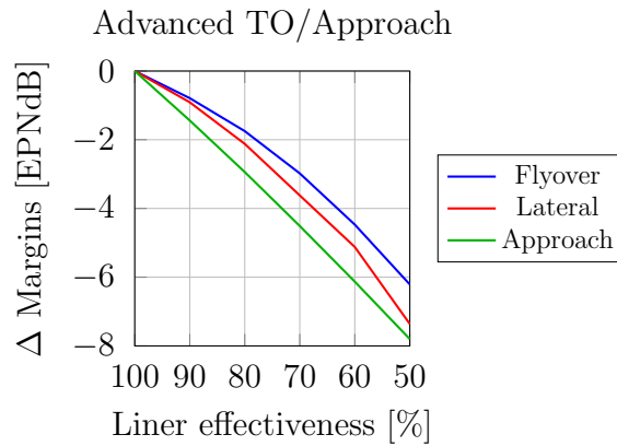
Figure 6.17: Variation in LTO certification levels when liner effectiveness is reduced
