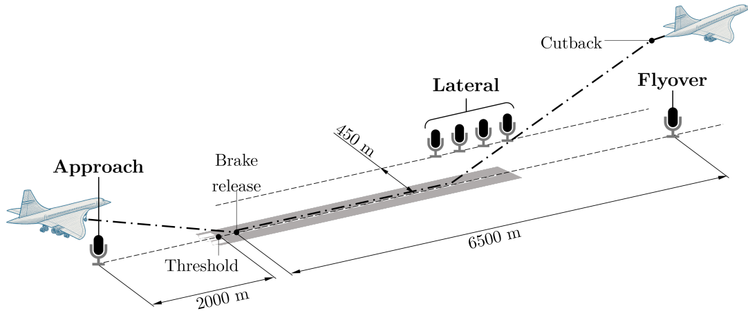
Figure 4.2: Certification points on take-off and landing according to ICAO with relevant operational points
