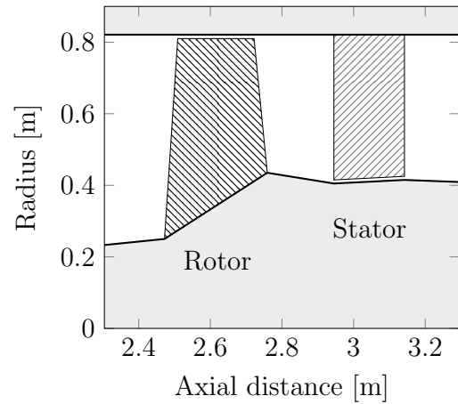
Figure 5.4: Single-stage fan schematic in meridional view
