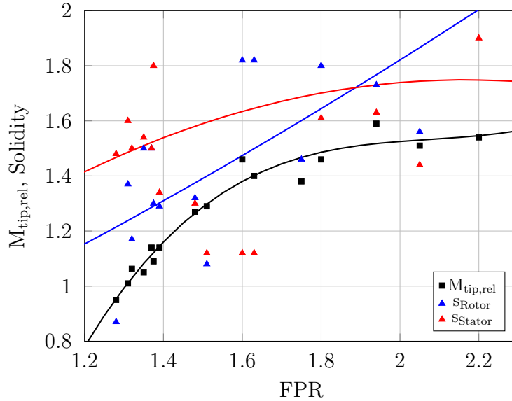
Figure 5.1: Turboman design data from internal database with polynomial regression curves 3
