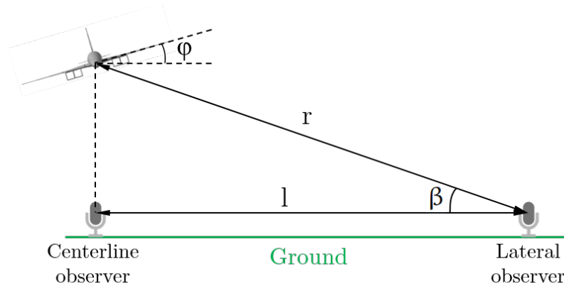
Figure 4.4: Measurements relevant to attenuating effects: roll angle \varphi , elevation angle \beta , observer distance r and lateral distance l
