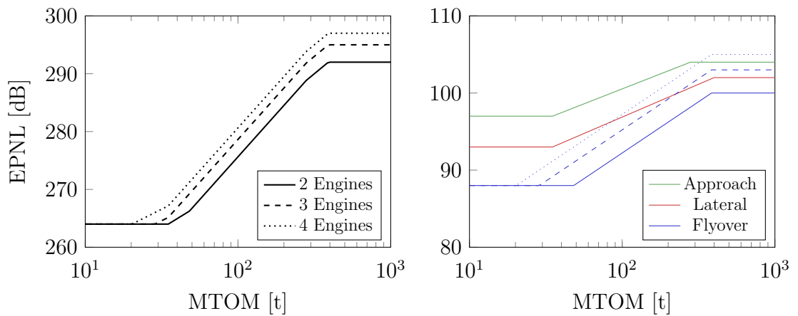
Figure 4.3: Maximum certification noise levels according to Chapter 14 , cumulative on the left and individual certification points on the right
