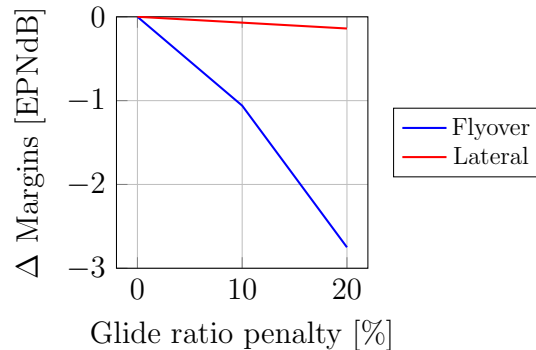
Figure 6.12: Change in certification margins for a degraded glide ratio on a standard take-off profile
