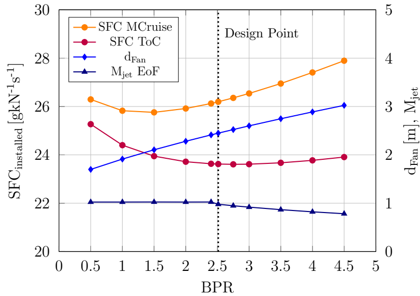
Figure 2.4: SFC at Top of Climb (ToC) and Mid Cruise (MCruise), fan diameter ( D_{\text{Fan}} ) and End of Field exhaust jet Mach number ( M_{\text{jet}} EoF) as function of the design point BPR for the installed engine, as shown by Plohr [103]
