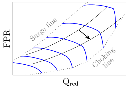
Figure 2.6: Generic SST fan map showing the shift of working lines when the nozzle throat is opened
