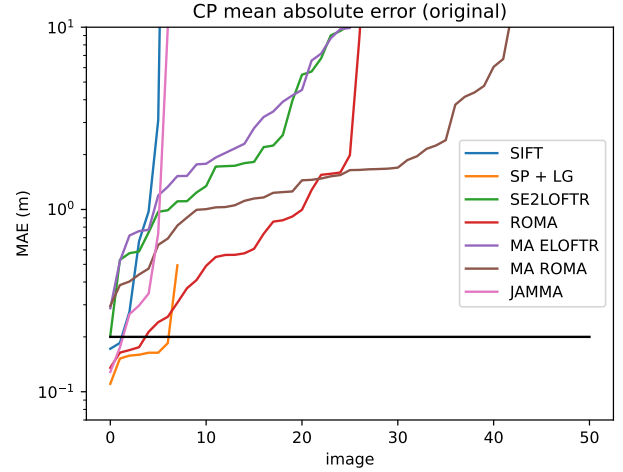
Figure 3. Per image checkpoint MAE for the different matchers for matching original and 20 cm reference imagery.
