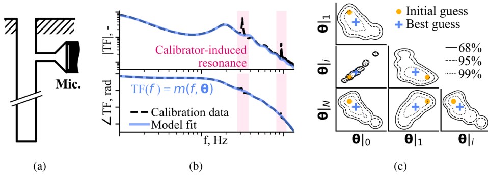
Fig. 18. Illustration of the ASSIST method applied to RMP calibration data. a) Diagram of a semi-infinite waveguide type RMP. b) Empirical TF with spurious resonance and model fit from the ASSIST model. c) Highest density credible intervals of some model parameter combinations with the initial and best guesses for the parameter values.
