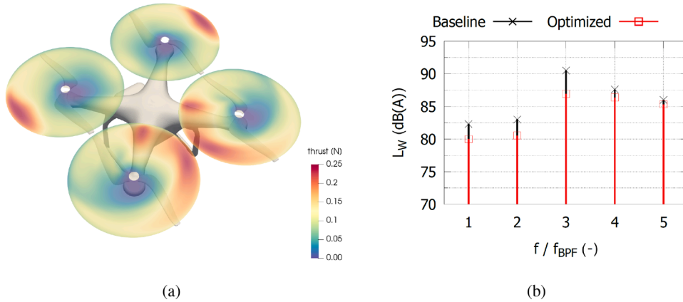
Fig. 7. (a) Propeller blade loading absolute value for the second optimisation case and (b) A-weighted SWL levels for the second optimisation case.
