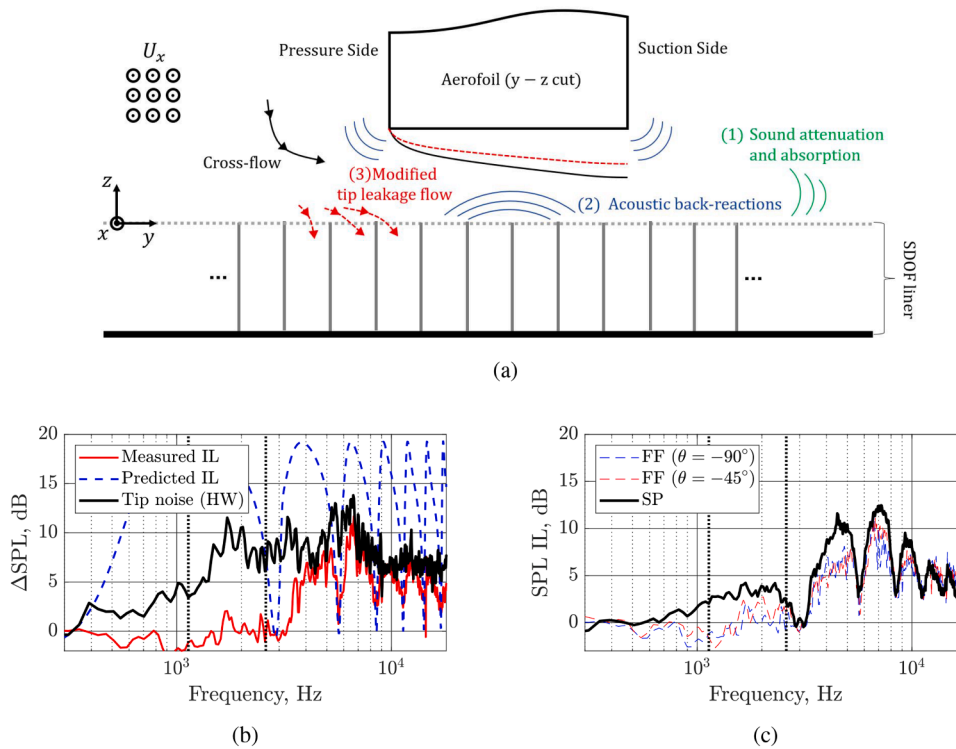
Fig. 17. Noise reduction with over-tip liners; (a) schematic of the proposed noise reduction mechanisms, (b) measured and predicted far-field SPL Insertion Loss (IL) and comparison to tip leakage excess noise of the hard wall (HW) configuration, and (c) comparison of wall pressure (SP) and far-field (FF) SPL insertion loss at two azimuthal \theta locations.
