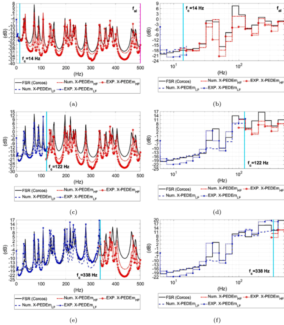
Fig. 24. Panel PAN A (all edges free): structural response (PSD acceleration) to a TBL excitation (Corcos model) at different flow velocities U_0 . Comparison between the numerical FSR (solid line), numerical X-PEDEM applied in the LF (dashed line) and HF domain (dotted-dashed line), experimental X-PEDEM for the LF (dotted line with full circle) and HF domain (dotted line with empty circle) evaluated for N_{acq} = 8 and N_{ex} = 16 . (a) narrow bands for U_0 = 25 m/s ( f_c = 14 Hz); (b) 1/3 octave bands for U_0 = 25 m/s ( f_c = 14 Hz); (c) narrow bands for U_0 = 75 m/s ( f_c = 122 Hz); (d) 1/3 octave bands for U_0 = 75 m/s ( f_c = 122 Hz); (e) narrow bands for U_0 = 125 m/s ( f_c = 338 Hz); (f) 1/3 octave bands for U_0 = 125 m/s ( f_c = 338 Hz).
