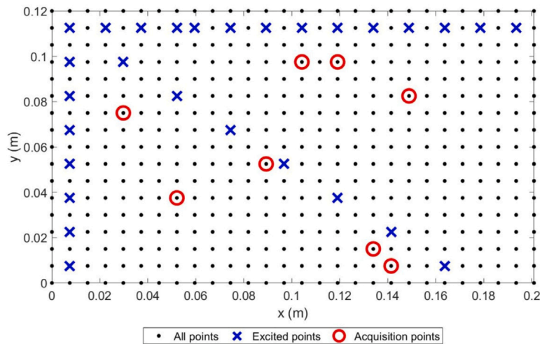
Fig. 23. Configuration for the position of excitation points (blue crosses) and for acquisition points (red circles) over a generic mesh grid of a panel. (For interpretation of the references to colour in this figure legend, the reader is referred to the web version of this article.)
