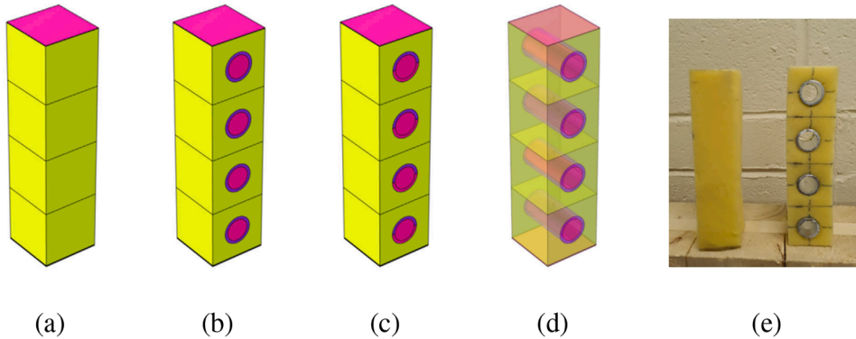
Fig. 11. (a) Homogeneous acoustic package; (b) Hollow inclusions; (c) Half-cut hollow inclusions; (d) Helmholtz resonators; (e) tested sample.
