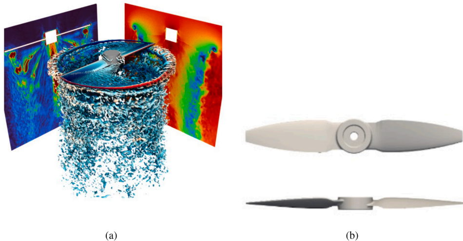
Fig. 6. (a) Instantaneous Q-criterion isosurfaces coloured by vertical velocity and contours of instantaneous vorticity and velocity magnitudes; and (b) optimised geometry.
