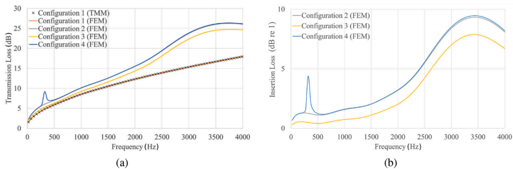
Fig. 13. Numerical transmission loss (a) and Insertion Loss (b) of Configurations from 1 to 4 (TMM and FEM results.).
