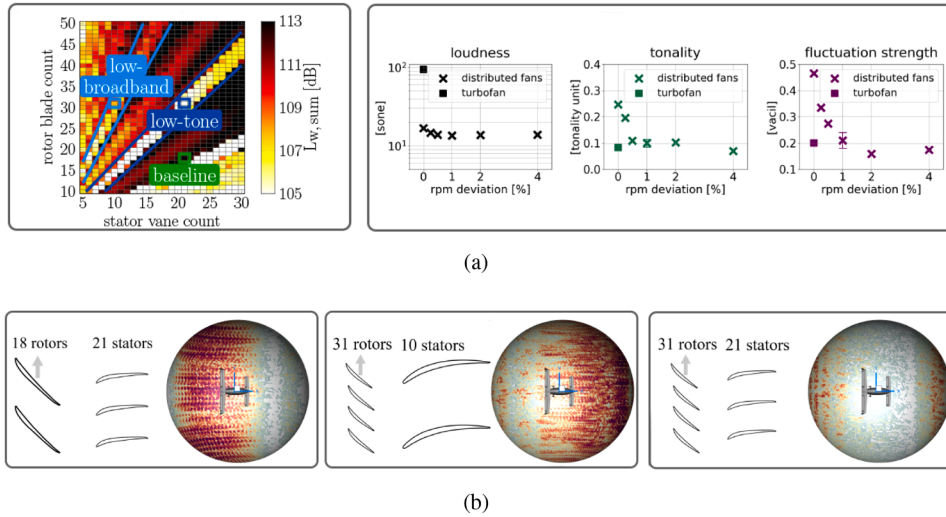
Fig. 21. a) Tonal interaction noise levels for different rotor / stator blade counts and impact of rotational speed (rpm) deviations on Sound Quality Metrics for the low-broadband fan. b) 2D cross-sections of three selected fan designs (left: baseline, center: low-broadband, right: low-tone) and tonal noise directivities obtained from a distributed propulsion system plotted as hemispheres.
