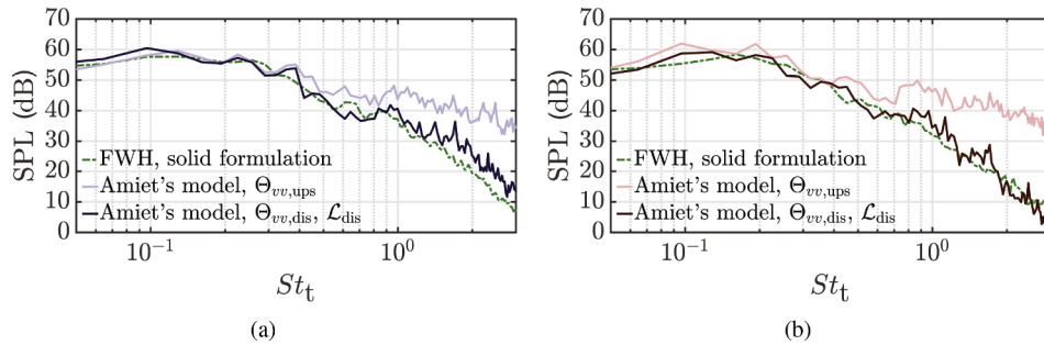
Fig. 25. SPL for an observer placed above the leading edge ( R = 1.2 m, \theta = \pi/2 ), for the (a) NACA 0012 and the (b) NACA 0012-103 airfoils. Amiet's model implementations using the upstream spectrum \Theta_{vv,ups} and the distorted spectrum \Theta_{vv,dis} along with the corrected aeroacoustic transfer function \mathcal{L}_{dis} are compared to the results of the FW-H analogy. The reference pressure used to calculate the SPL is 2 \times 10^{-5} Pa.
