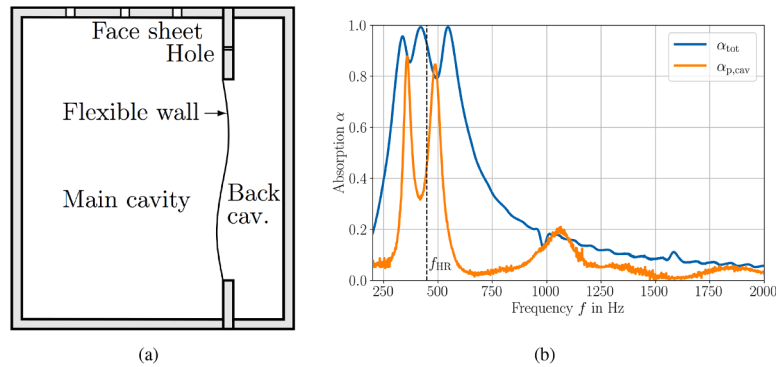
Fig. 14. (a) Schematic cell. (b) Normal incidence absorption of the whole resonator (blue), only the plate with back cavity (orange) determined using cavity microphones and theoretical Helmholtz resonance frequency (black). (For interpretation of the references to colour in this figure legend, the reader is referred to the web version of this article.)
