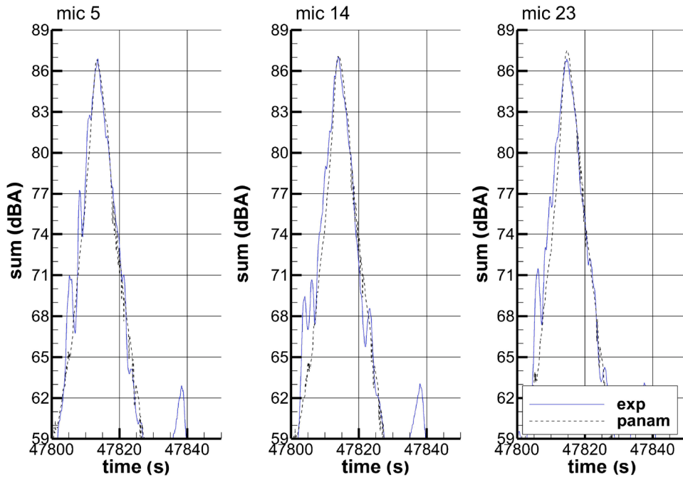
Fig. 1. Assessment of noise mitigation measures: Measured (blue) vs. PANAM results (black). (For interpretation of the references to colour in this figure legend, the reader is referred to the web version of this article.)
