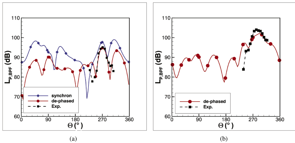
Fig. 8. Fly-over noise directivity for AoA = 0^\circ (a) and AoA = 10^\circ (b) compared to experimental results.
