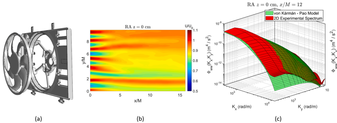
Fig. 22. Automotive low-speed cooling fan (a); SPIV streamwise velocity component highlighting the radiator fins' wakes (b); von-Kármán-Pao-corrected turbulence spectrum compared to the experimentally measured one (c).
