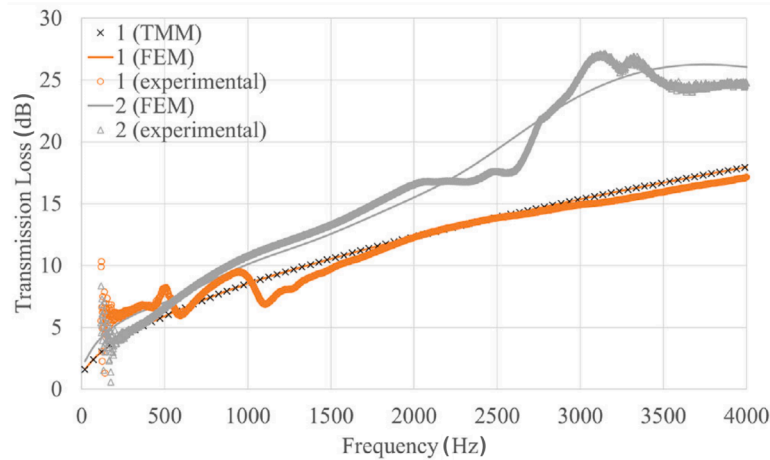
Fig. 12. Numerical and experimental comparison of transmission loss of configurations 1 and 2.
