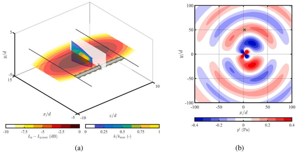
Fig. 3. (a) the acoustic sound map of a porous coated cylinder for a one-third octave frequency band of 2.5 kHz superimposed on the turbulence kinetic energy contour. The maps are normalised by their respective maximum values. (b) a snapshot of the total acoustic pressure radiated at the vortex-shedding frequency.
