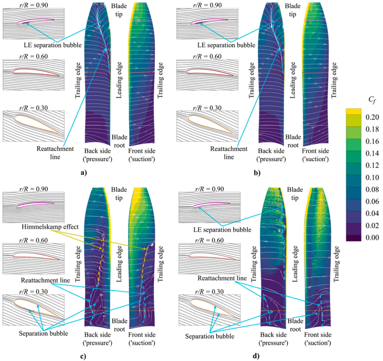
Fig. 5. Visualisation of flow around propeller blades at the positive thrust condition ( J = 0.60 ) using skin friction coefficient and shear lines: a) SRANS, b) URANS, c) LB-VLE _{y^+ \geq 15} , d) LB-VLES _{y^+ \leq 10} .
