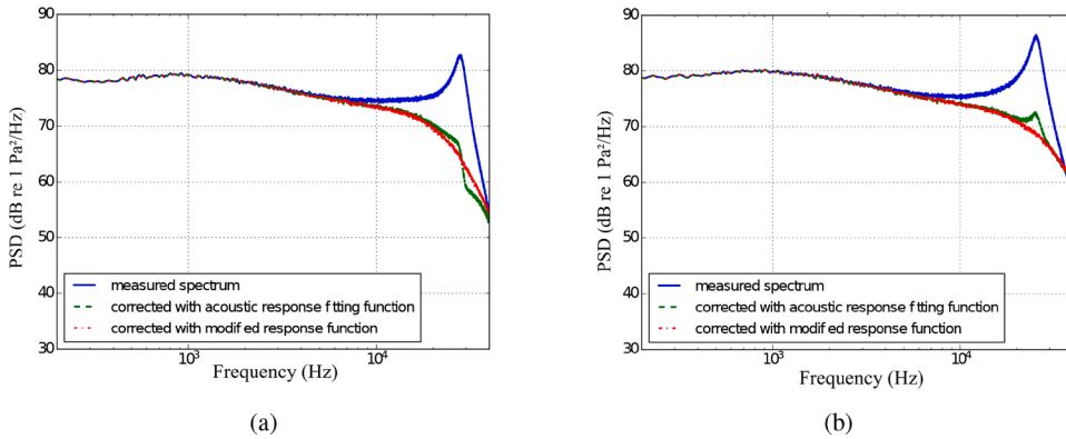
Fig. 19. Measured and corrected wall pressure spectra in zero pressure gradient flows with U_\infty = 60 m/s, (a) d = 0.5 mm (b) d = 0.35 mm.
