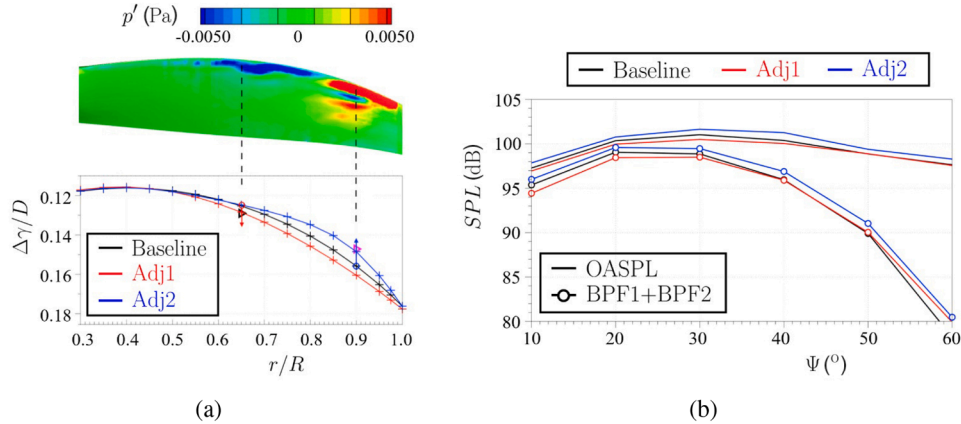
Fig. 4. (a) Surface pressure p' contribution (of baseline configuration) to the first interaction tone BPF1 + BPF2, and adjustment of rear blade sweep. (b) Upstream directivity of rear blade noise due to (aft) blade sweep adjustments.
