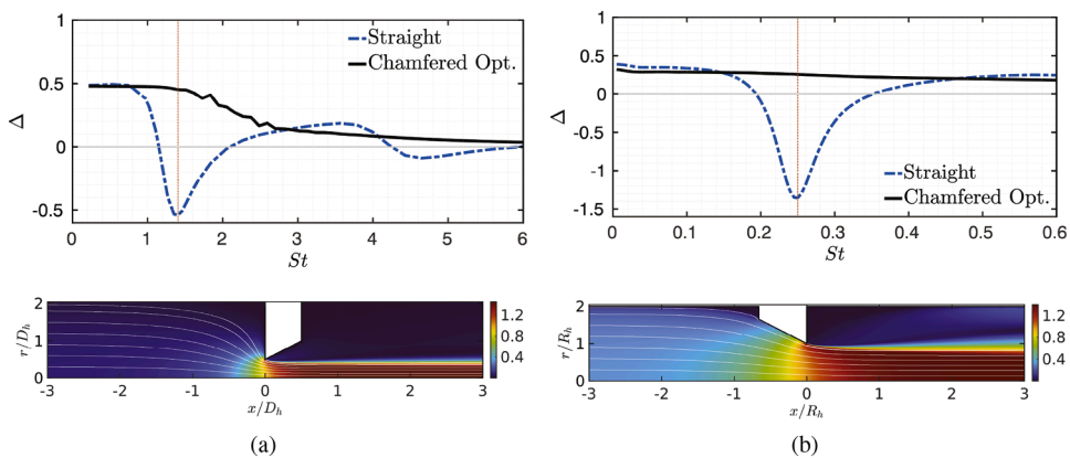
Fig. 15. Acoustic absorption coefficient (top) for straight (blue dash-dotted line) and optimally-chamfered perforation (black solid line). Mean flow velocity magnitude for optimal configurations (bottom). Laminar (a) and turbulent (b) bias flow. (For interpretation of the references to colour in this figure legend, the reader is referred to the web version of this article.)
