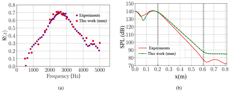
Fig. 16. (a) Real part of the liner impedance obtained from normal incidence experiments performed at the LAUM laboratory, and (b) numerical results at SPL 150 dB and SPL along the opposite wall to the liner at 1000 Hz in grazing wave conditions, tested by the NASA Langley Liner Physics team, with vertical black dashed lines delimiting the liner position.
