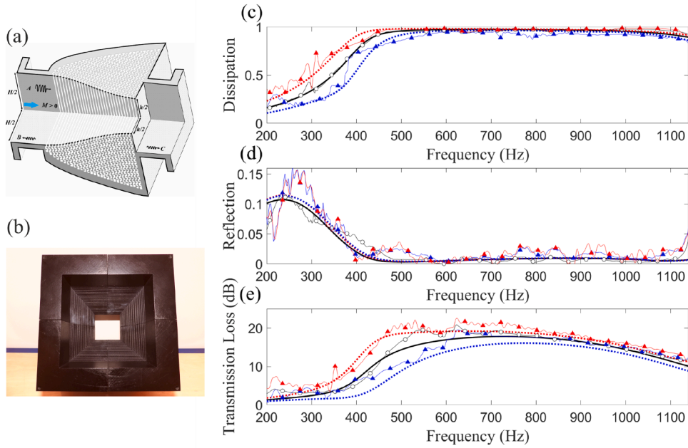
Fig. 10. (a) Sketch of the converging coiled silencer under a left excitation along the flow direction (DPC); (b) Picture of the silencer cavity mouths viewed from the inlet section; (c) Dissipation, (d) reflection and (e) TL spectra of the optimised rainbow-trapping silencer simulated by the TMM (black solid, no-flow; blue dots, DPC: M_{in} = 0.04 ; red dots, UPC: M_{in} = -0.04 ) and measured in the aeroacoustic test bench (white circles, no-flow; blue triangles, DPC: M_{in} = 0.04 ; red triangles, UPC: M_{in} = -0.04 ). (For interpretation of the references to colour in this figure legend, the reader is referred to the web version of this article.)
