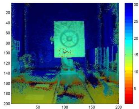
Figure 7. The CamCube provided by PMD-Technologies GmbH and a typical 3D image showing a satellite mockup in EPOS-laboratory
