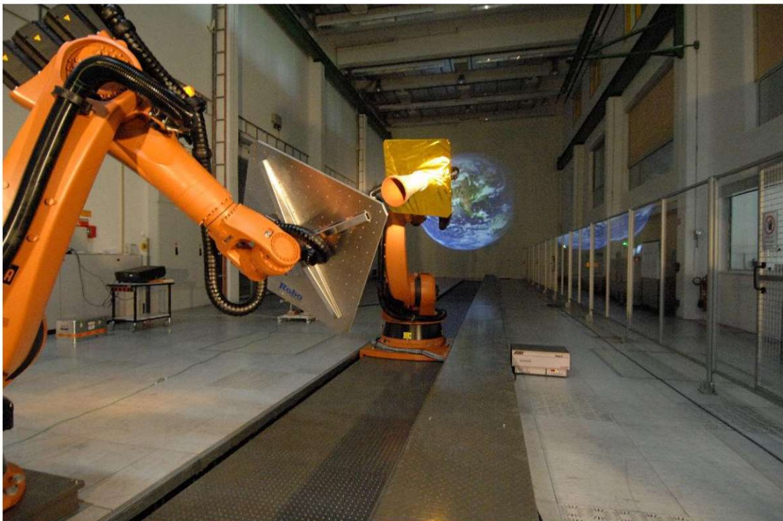
Figure 8. The new EPOS 2.0 facility Credit: DLR, Robo Technology
