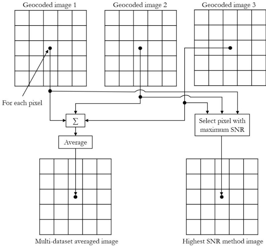
Figure 3.9: "Multi-Dataset Averaging Method" (left) and "Highest SNR Method" (right).
