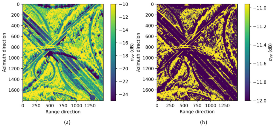
Figure 3.7: \sigma_{\text{VV}}^o images. (a) \sigma_{\text{VV}}^o image for Cologne motorway intersection. (b) \sigma_{\text{VV}}^o image showing primarily reflections from lane divider and flyover walls.
