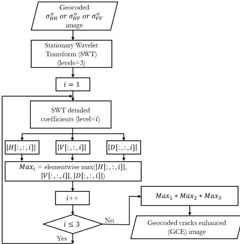
Figure 6.5: Cracks enhancement procedure using the SWT.
