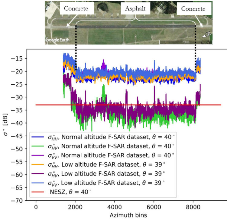
Figure 3.1: \sigma^{\circ} vs NESZ plots for the Kaufbeuren runway. The Google Earth image shown at the top highlights the asphalt and concrete regions of the runway.
