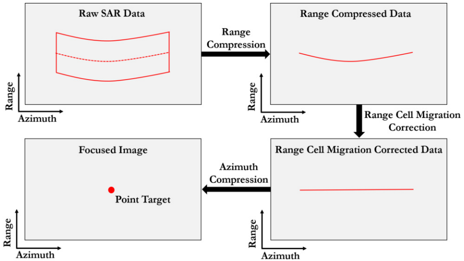
Figure 2.3: Major steps in focused SAR image generation from raw data.
