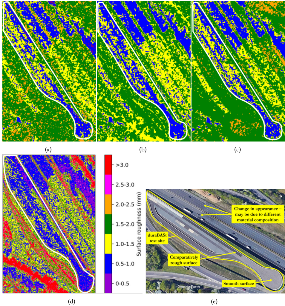
Figure 4.9: Surface roughness results for the duraBASt test site (white and yellow border), with results obtained using (a) artificial neural network, (b) support vector regression, (c) random forest regression, and (d) new semi-empirical models. (e) Corresponding Google-Earth image.
