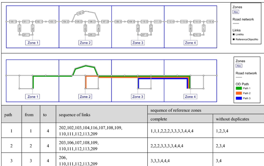
Fig. 5 Matching algorithm for DRT trips. (Source: Friedrich et al. 2018, (7, p. 1644))
