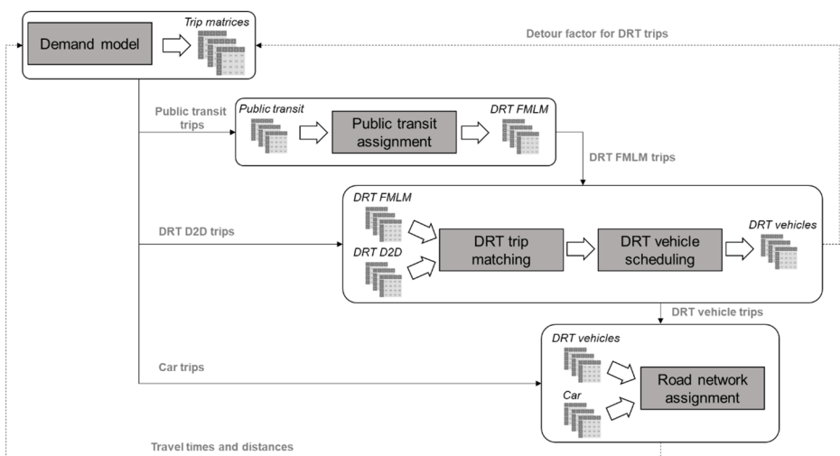
Fig. 4 Schematic overview of the model processes
