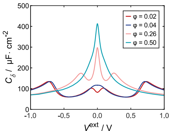
Fig. 5. Differential capacitance C_\delta versus applied potential V^{\text{ext}} of a symmetric electrolyte for different dilutions \phi including solvation.
