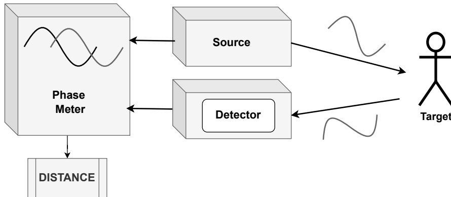
Figure 2.3: AMCW Working Principle. A source emits a modulated wave towards a target, and the reflected wave is captured by a detector. The phase shift between the emitted and received signals is measured using a phase meter. This phase difference is proportional to the distance traveled by the wave, allowing the system to calculate the target's distance with high precision.
