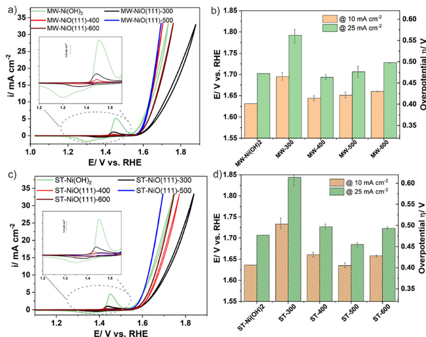
Fig. 6 (a) iR -corrected cyclic voltammograms of (a) MW-NiO(111) nanosheets and (c) ST-NiO(111) nanosheets, measured at 10 mV s -1 in 0.1 M KOH solution. The insets show the Ni 2+ /Ni 3+ redox transitions. Corresponding overpotential comparison at 10 mA cm -2 and 25 mA cm -2 of (b) MW-NiO(111) nanosheets and (d) ST-NiO(111) nanosheets, reproduced from ref. 53 with permission from ACS Appl. Mater. Interfaces, copyright 2024.
