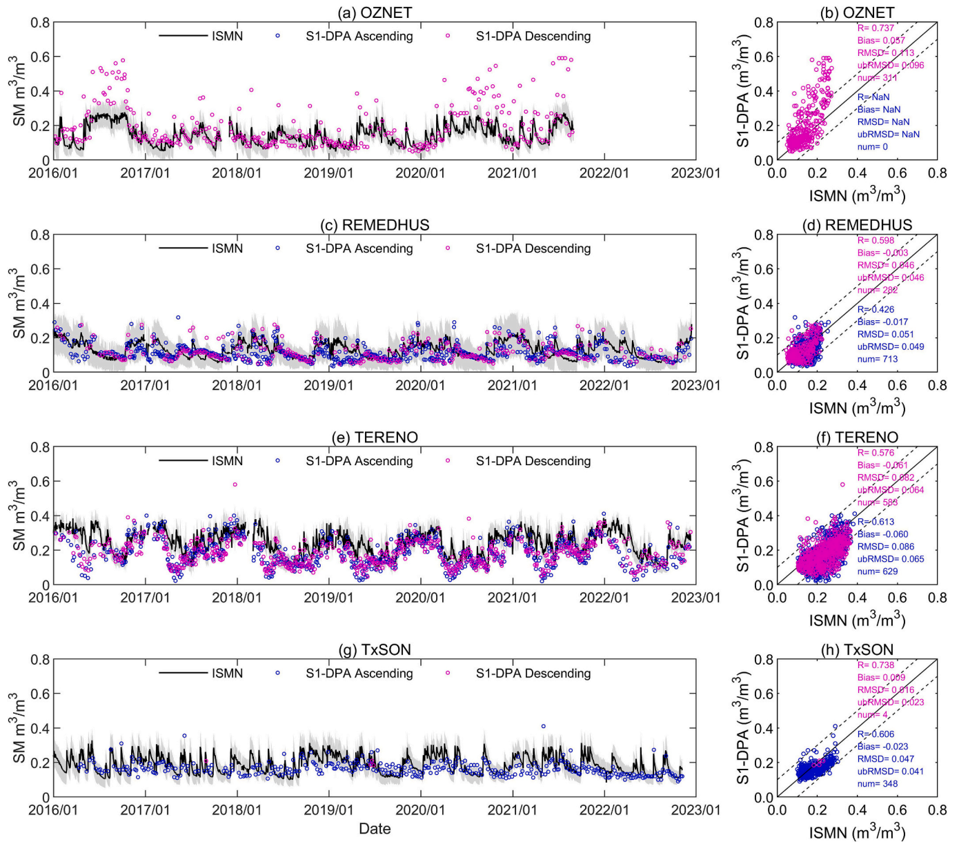
Fig. 4. Temporal variations of the SM derived from S1-DPA and ISMN during 2016–2022: OZNET (a, b), REMEDHUS (c, d), TERENO (e, f), and TxSON (g, h). Data from ascending orbits are shown as blue dots and data from descending orbits as pink dots, while the black lines denote the average of the SM from ISMN and the gray area is the \mu \pm \sigma . The dotted lines in the scatter plots indicate the margin of \pm 0.1 \text{ m}^3/\text{m}^3 . (For interpretation of the references to colour in this figure legend, the reader is referred to the web version of this article.)
