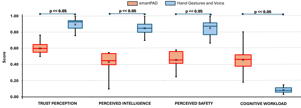
Fig. 7: Comparison of interaction metrics between smartPAD and combined gesture-voice control is shown with normalized scores (0-1) for trust, intelligence, safety, and cognitive workload. All differences are statistically significant ( p \ll 0.05 ), with combined gesture-voice control consistently outperforming smartPAD across all metrics.
