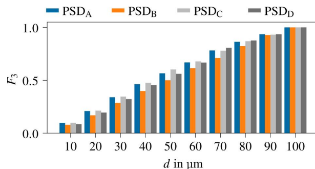
Fig. 12 Normalized cumulative volume based spray particle size distribution sampled from SPH simulations for all four studied operating conditions
