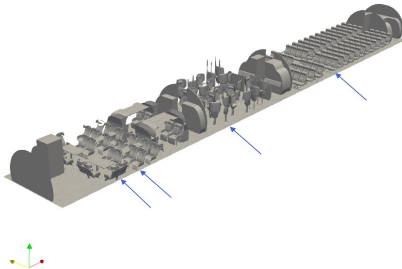
Figure 6: Modified novel cabin design
