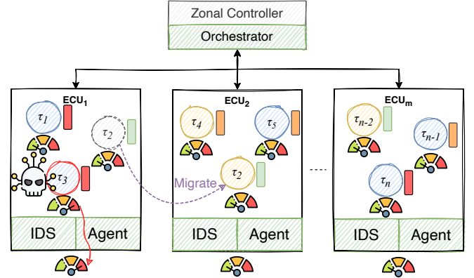
Fig. 1. SHIFTGUARD illustration. The ECUs are connected via a gateway. High-critical (yellow) and low-critical (blue) tasks coexist on the same ECU. The tasks have a required security level (e.g., high \square , medium \square , and low \square ). An IDS monitors task behavior and maintains each task’s security level (meter). A migration agent and orchestrator handles task migration based on the required level. In this case, \tau_2 moves from ECU 1 to ECU 2 as a compromised task \tau_3 (red) reduces ECU 1 ’s overall “trustworthiness” (depicted with red meter) needed to run \tau_2 . The shaded green components (IDS, agent, and orchestrator) operate in a privileged space.
