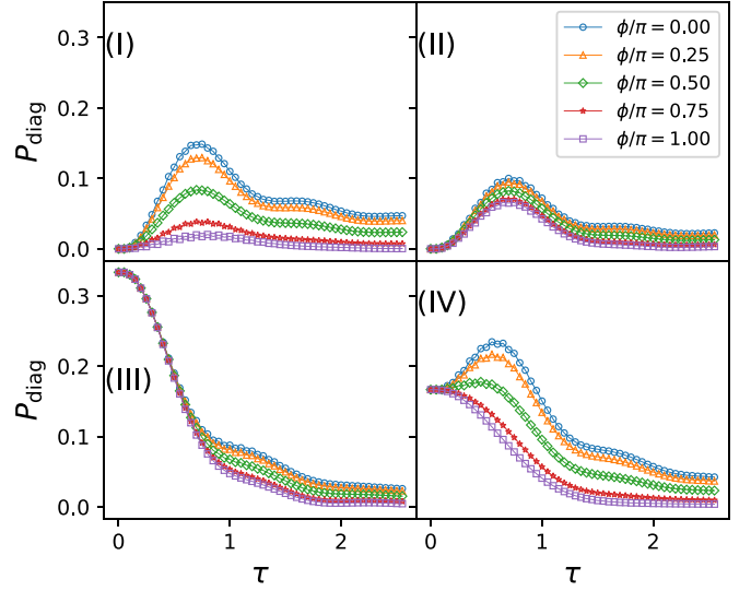
FIG. 2. The two-particle coincidence probability as defined in Eq. (9), for different values of the particle exchange statistics parameter \phi . Bosons tend to occupy equal spatial modes during the evolution, leading to pronounced peaks in the probability of coincidence events. For fermions, such coincidences are less likely due to the Pauli exclusion, although peaks might still develop as in (II). Data corresponds to the different initial conditions (I), (II), (III), and (IV) from Fig. 1, with L = 16 , t = 0.05 and a total of n = 50 time steps, with \tau = nt .
