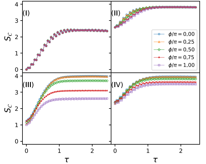
FIG. 5. Entanglement entropy from Eq. (15) for the initial conditions in Fig. 1 for the state \rho_C defined in Eq. (13). Note that states (II), (III), and (IV) have initially significant entanglement. The von Neumann entanglement entropy grows with increasing the number of steps, signaling thermalizing behavior of the internal degrees of freedom with the environment. Note that specially for cases (III) and (IV), statistics of particles play a significant role in the reach value. Data correspond to t = 0.05 , a total of 50 time steps, and L = 40 .
