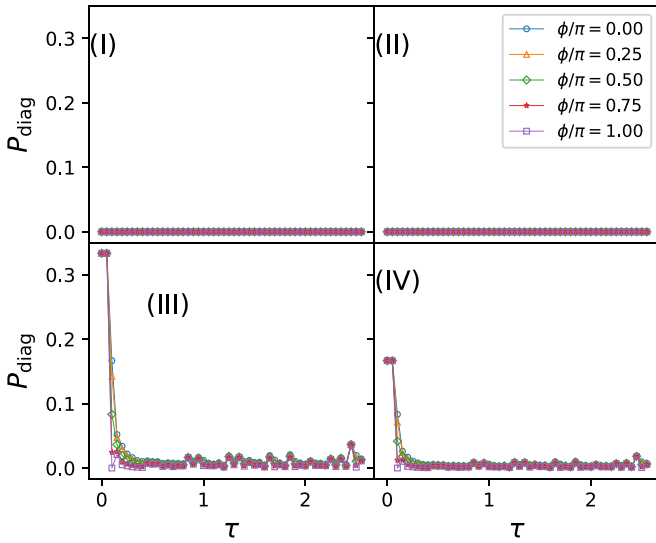
FIG. 10. The same figure as Fig. 2, for the model described in Eq. (D1). Data correspond to a total of 50 time steps, and L = 40 . Note that the time axes have been scaled by a factor t = 0.05 , with \tau = nt , for comparison purposes.
