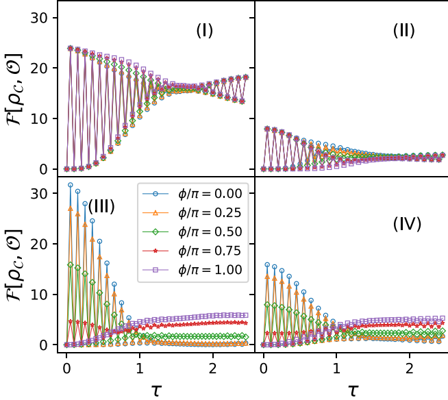
FIG. 4. Quantum Fisher Information from Eq. (12) for the initial conditions in Fig. 1, for the state \rho_C defined in Eq. (13). For (II), particles with \phi = 0 retain a higher value for the QFI than particles with \phi = \pi . In contrast, in configurations (III) and (IV) evolution of the QW leads to an increment in the QFI for particles with \phi = \pi , whereas for particles with \phi = 0 the QFI tends to decrease. Data correspond to t = 0.05 , a total of 50 time steps, and L = 40 .
