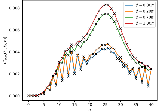
FIG. 8. Benchmarked calculation for two-particle correlations on a square lattice of L \times L dimensions, with L = 3 , t = 0.1 , N = 4 particles and 40 total steps, for different values of \phi in the initial state. The solid lines correspond to the exact numerical calculation by acting directly with the operators on the full state of dimension (2L^2)^N , whereas crosses indicate the values calculated with Eq. (B2) using the single-particle wave function coefficients. The N = 4 particles are initialized at (x, y, \sigma) \equiv (0, 0, \uparrow), (0, 2, \downarrow), (2, 0, \downarrow), (2, 2, \uparrow) . The correlation is calculated for \sigma_1, \sigma_2 = \uparrow, \downarrow and \vec{r}_1 = \vec{r}_2 = (2, 2) .
