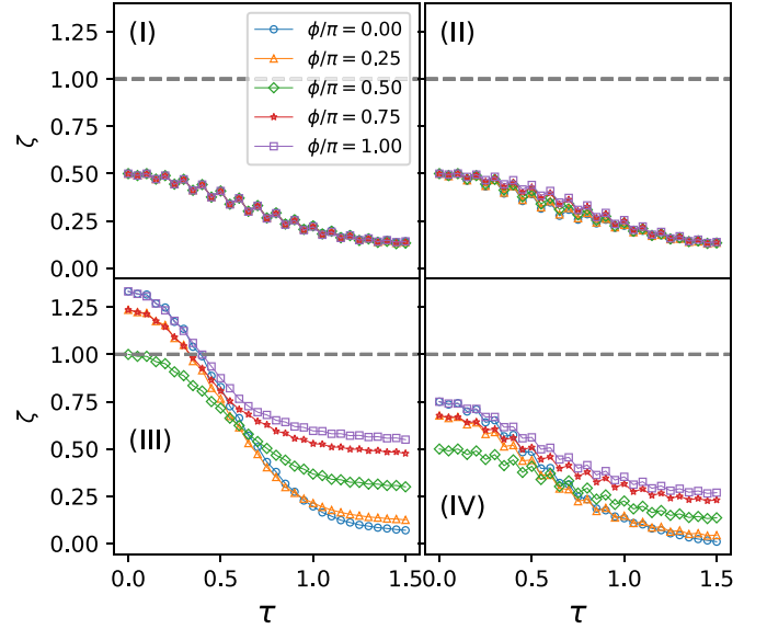
FIG. 7. Performed Bell tests for the four different initial conditions in Fig. 1. Only condition (III) shows a violation of the Bell inequality in Eq. (C3) during the initial time steps, except for \phi = \pi/2 , where the inequality is satisfied. The classical bound at \zeta = 1 has been represented by a dashed grey line. Data correspond to 30 time steps, t = 0.05 and L = 40 .
