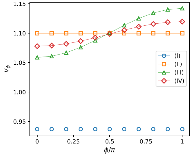
FIG. 11. The same figure as Fig. 4, for the model described in Eq. (D1). Data correspond to a total of 12 time steps, and L = 40 . In this case, no scaling of the x axes was performed to extract the velocities, i.e., v_\phi is obtained by setting t = 1 in Eq. (11).
