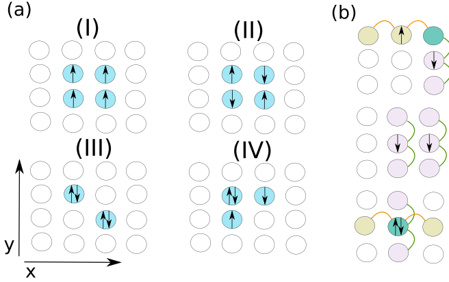
FIG. 1. (a) Different initial state configurations for the state |\Psi_0\rangle defined in Eq. (2), for N = 4 particles on a square lattice of L \times L lattice sites with L = 4 . Occupied spatial modes allocating particles with \sigma = \uparrow, \downarrow internal degrees of freedom are filled in blue, whereas empty spatial modes are represented by a white background circle. The initial state |\Psi_0\rangle incorporates different particle statistics through the phase \phi . (b) Illustration of the conditional hopping process described in Eq. (4) for initial product states in the |x, y, \sigma\rangle basis; hopping between nearest neighbors have been represented with lines, and allowed spatial modes due to hopping processes have been colored. The green regions represent spatially shared modes due to shared hopping into that lattice position.
