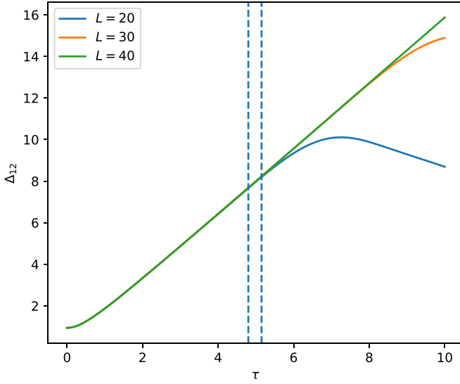
FIG. 9. System size scaling of the interparticle distance \Delta_{12} for the QW with initial configuration given by (III) in Fig. 1, with \phi = \pi , \tau = nt with t = 0.05 . The deviation from linear behavior observed for smaller system sizes corresponds to boundary effects from particles reaching the edges of the lattice. The slope of \Delta_{12} in the linear behavior region determines the propagation speed v_\phi . The slope v_\phi is extracted in the region delimited by the dashed lines.
