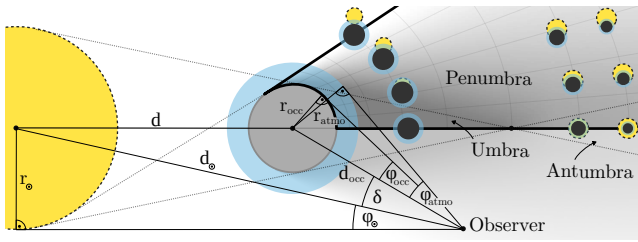
Figure 2: This figure shows the lengths and angles used in this paper. It extends the nomenclature introduced in Figure 2 of [SGAG22] with the radius r_{atmo} , the angular radius \varphi_{atmo} , and the average distance between Sun and occluder d . The small glyphs provide an approximate visualization of how Sun and occluder may look from the respective position in the shadow cone. For a more detailed visualization, refer to Figure 4. The thick dark line encloses the area for which we will precompute the eclipse shadow.
