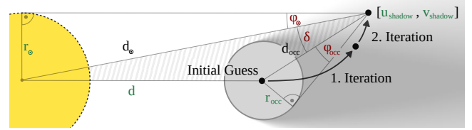
Figure 8: This shows a schematic overview of the iterative search required to reconstruct \varphi_{\odot} , \delta , and \varphi_{occ} (red) for some given u_{shadow} , v_{shadow} , d , r_{\odot} , and r_{occ} (green). d_{occ} and d_{\odot} are iteratively updated to find the correct position in space. The law of cosines is used in the hatched triangle to compute d_{\odot} based on the other two sides and \delta (see Equation 6).
