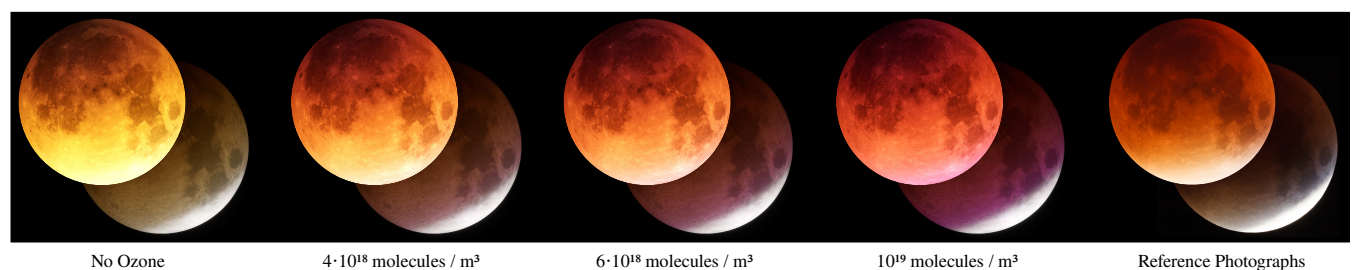
Figure 13: Our system allows for a fine-grained control of the atmospheric properties. For the left images, we simulated an atmosphere without ozone. The centre images have been generated using a tent-shaped ozone distribution with a peak altitude at 25 km, a width of 15 km, and the peak molecular density number shown in the caption. The right image shows two reference photographs of the 2015 lunar eclipse. The upper images show the Moon in the umbra, the lower images at the edge of the penumbra.
