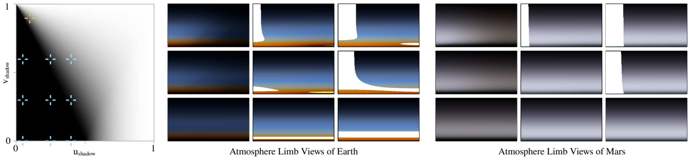
Figure 9: The left graph shows an eclipse-shadow LuT. The u -axis corresponds to the ratio of the angular radii of Sun and occluder which correlates with the distance to the observer. The occluder is at the left edge of the LuT, the end of the umbra is in the middle, and the right edge is infinitely far away from the occluder. The v -axis is mapped to the relative angular distance between Sun and occluder: The umbra core is at the bottom, the outer edge of the penumbra at the top. The extends of this LuT are marked with a thick black line in Figure 2. Next to the LuT, several limb views of the atmosphere around Earth and Mars are shown. The limb views have been captured from positions corresponding to the blue positions marked in the left graph. The orange position is the view from Figure 7.
