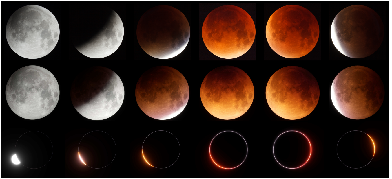
Figure 11: The upper row shows photographs of the lunar eclipse on 2015-09-28 taken at about 30-minute intervals starting at 1:00 AM UTC. All images use the same white balance and relative exposure values of 0 EV, +4 EV, +9 EV, +13 EV, +13 EV, and +9 EV respectively. The centre row shows renderings using our system. If there was no atmosphere, the third and sixth image would be almost completely black (except for the bright rim). The fourth and fifth image would be completely black. The bottom row shows how Earth would look like for an observer on the lunar north pole. If there was no atmosphere, the Sun would only be visible in the first image.
