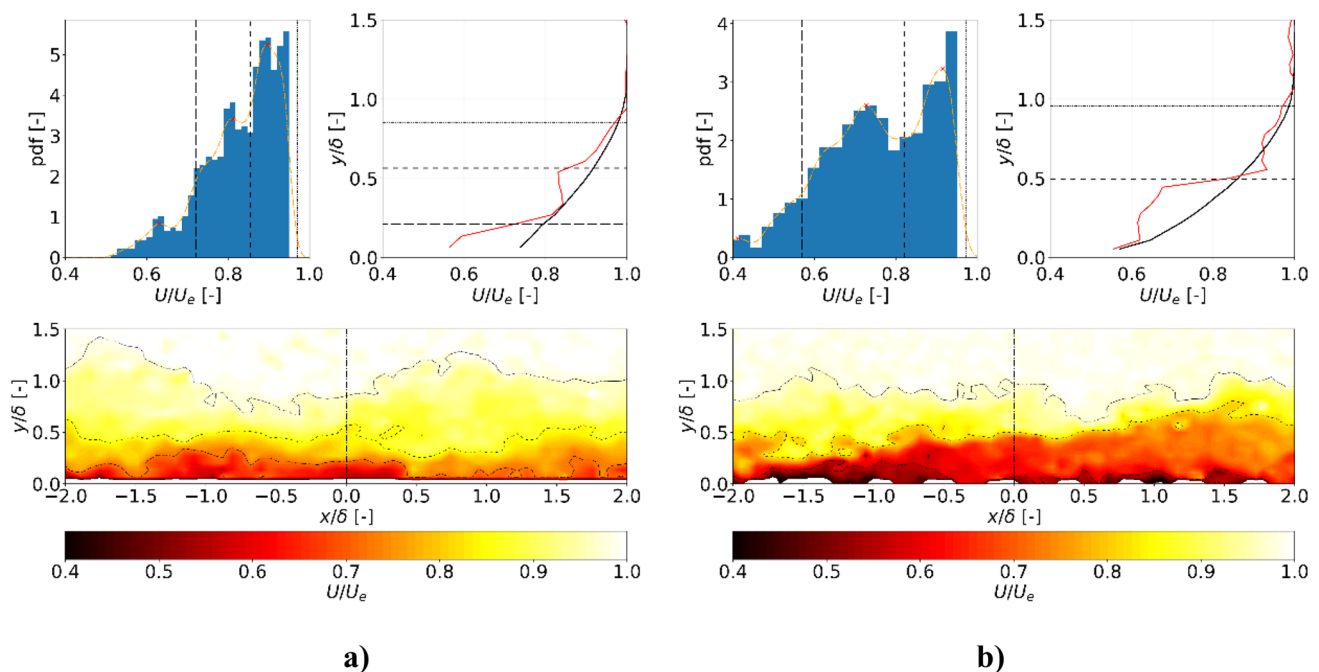
Fig. 14 Compilation of p.d.f. (upper left) based on an instantaneous velocity field (lower middle) and a comparison of an instantaneous (red line) to the mean velocity profile (black line, upper right) for a smooth wall (Run14) and b rough wall data (Run07). Boundaries for
