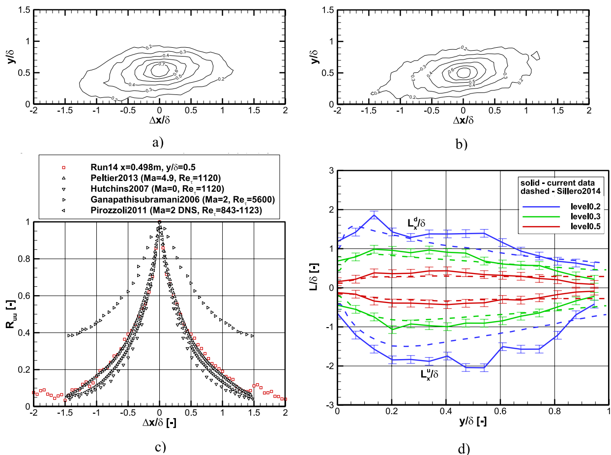
Fig. 10 Two-point correlation results of streamwise velocity fluctuations with (a) and (b) contour plots at y/\delta = 0.5 along smooth (Run14) and rough wall (Run07), respectively, c resulting one-dimensional autocorrelation of the streamwise velocity fluctuations R_{uu}(y_{ref}) at y/\delta = 0.5 for smooth wall (Run14) compared to data from Peltier (2013), Hutchins and Marusic (2007), Ganapathisubramani et al.
