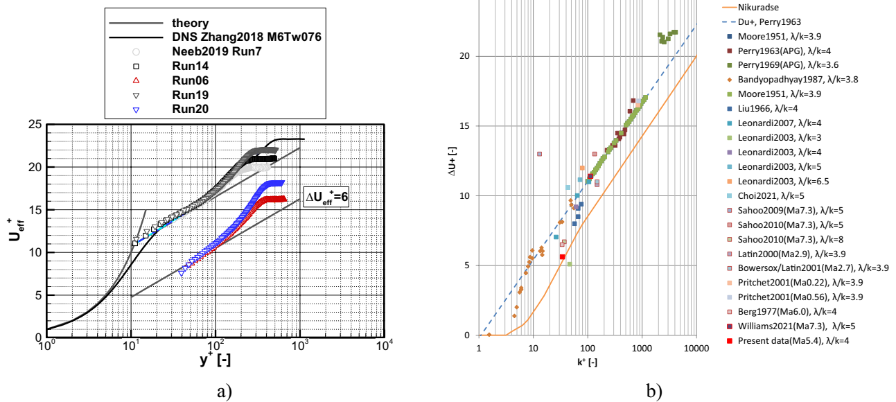
Fig. 7 a Inner scaled van Driest transformed mean velocity profiles along smooth (black, gray) and rough wall (colored) together with the law of the wall and DNS data according to Zhang et al. 2018. b Roughness function \Delta U_{eff}^+ against roughness Reynolds number k^+ for square bars of different wavelength close to a value of \lambda/k = 4 and authors (symbols without and with edge for incompressible and
