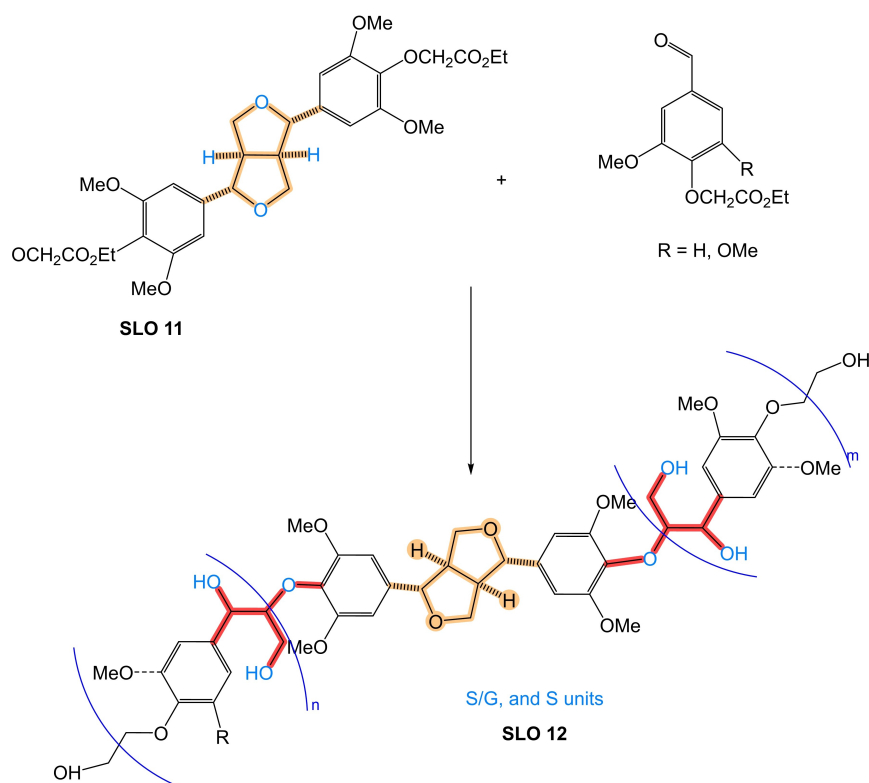
Scheme 4. Mechanisms for the synthesis method of Lancefield and Westwood. Adapted from Ref. [105] Copyright (2015), with permission from RSC.
