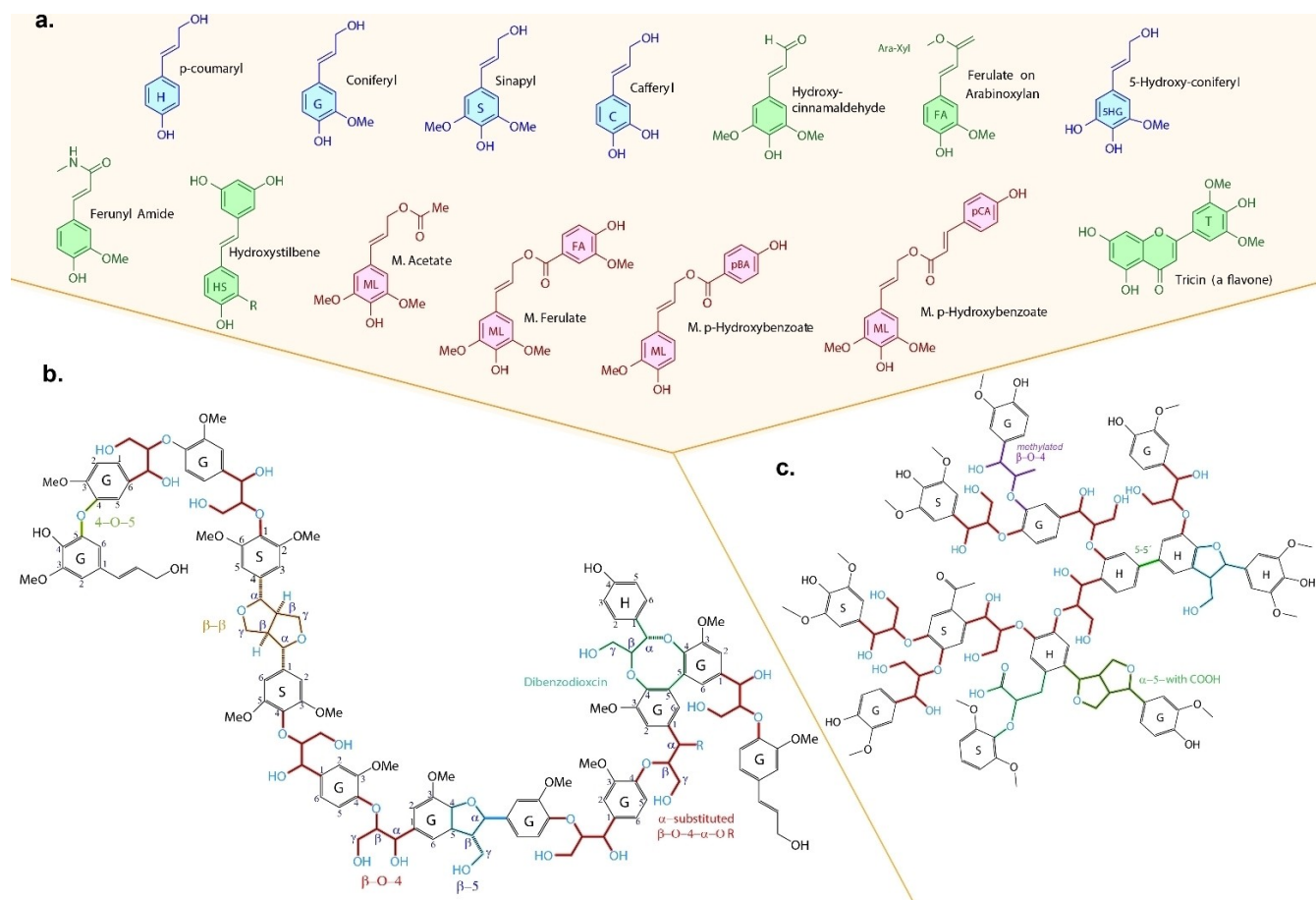
Figure 2. Structures of a) constituent monomer units. Adapted from Ref. [29], Copyright (2021), with permission from Elsevier. b) lignin structure. Adapted from Ref. [25] Copyright (2020), with permission from Wiley, and c) linkages of lignin oligomers. Adapted from Ref. [37] Copyright (2023), with permission from KIT.
