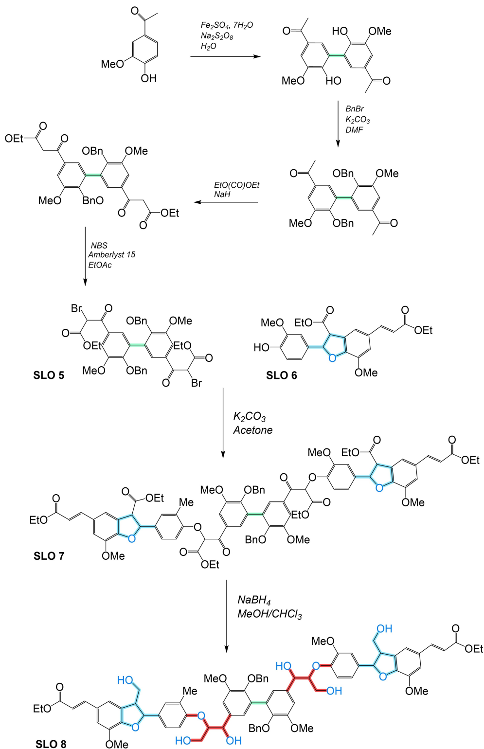
Scheme 3. Mechanisms for the synthesis method of Graham et al. Adapted from Ref. [224] Copyright (2013) with permission from RSC.
