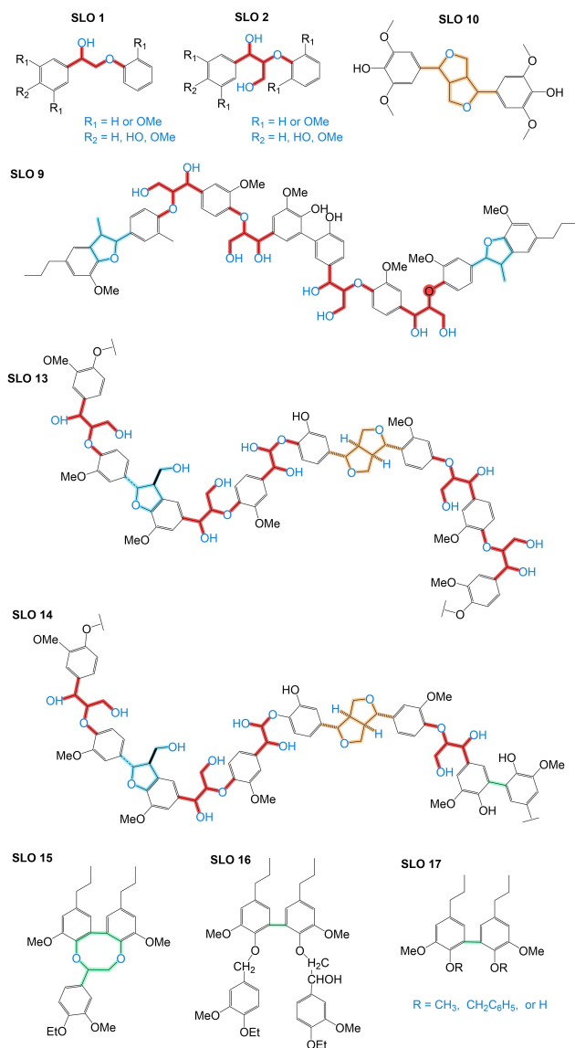
Figure 6. Molecular structures of the SLOs obtained by chemical and enzymatic synthesis referenced in Entries 1, 4, 5, 6, and 7 (Table 6). SLO 1–SLO 2 adapted from Ref. [25] Copyright (2020) with permission from Wiley. SLO 9 adapted from Ref. [224] Copyright (2013) with permission from RSC. SLO 13–14 adapted from Ref. [105] Copyright (2015) with permission from RSC. SLO 15–17 adapted from Ref. [225] Copyright (2004) with permission from Elsevier.
