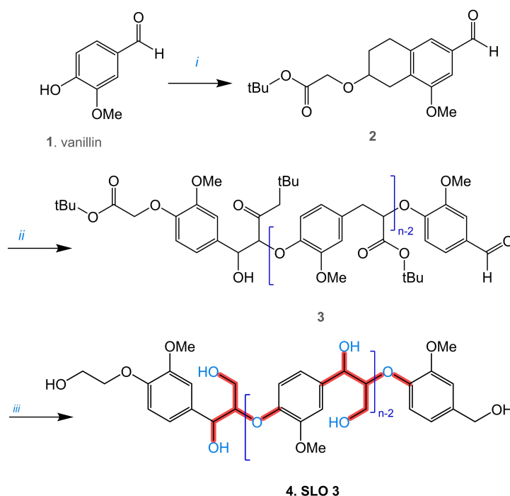
Scheme 1. Mechanisms for the synthesis method of Katahira et al., [23] with slight modifications. Adapted from Ref. [109] Copyright (2021), with permission from De Gruyter.
