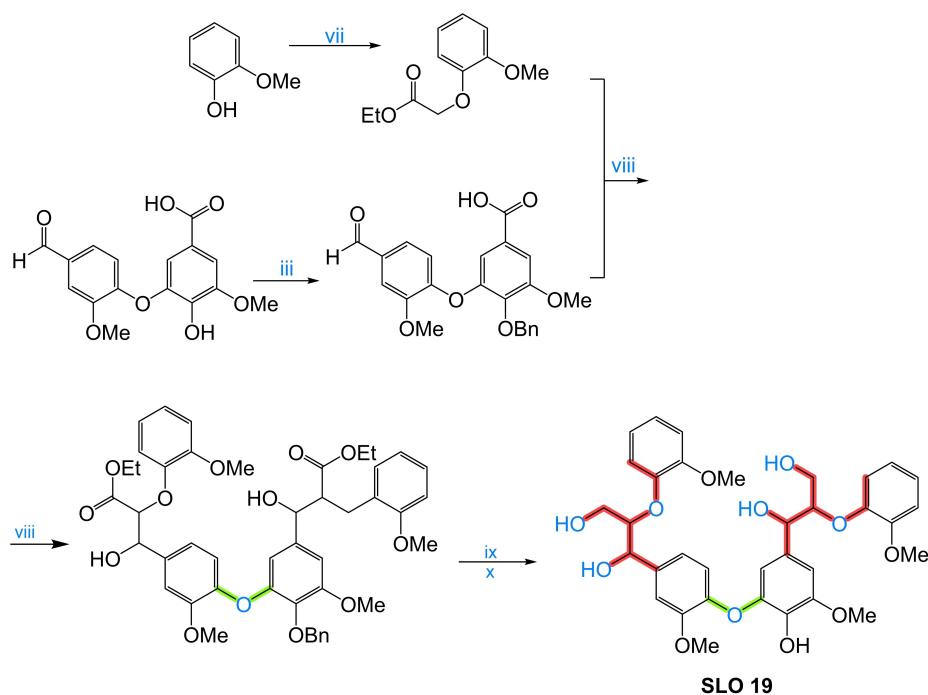
Scheme 6. Mechanisms for the synthesis method of Li et al. Adapted from Ref. [230] Copyright (2020), with permission from Wiley.
