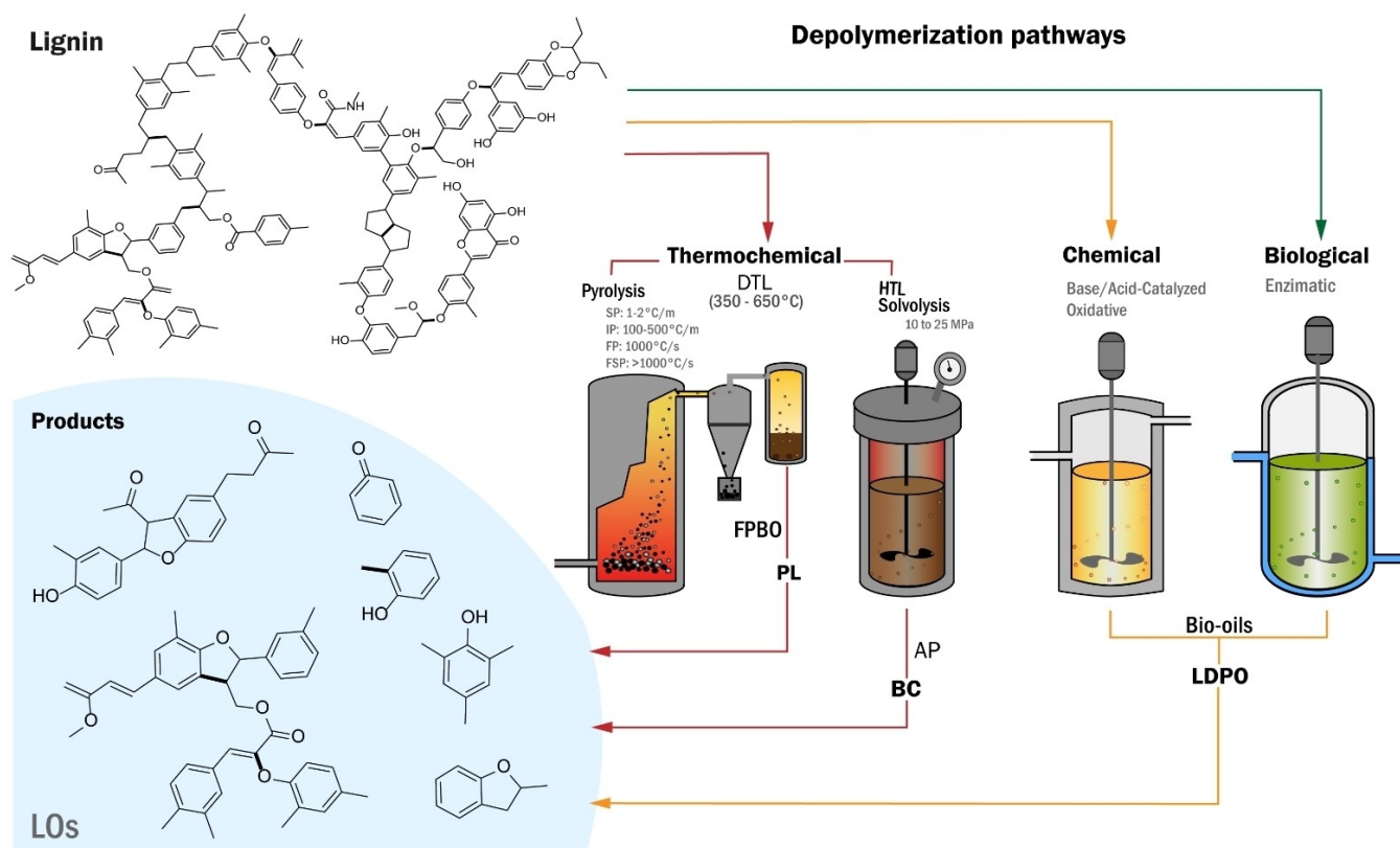
Figure 4. Depolymerization process to obtain liquid products rich in LO. (LDPO stands for lignin-derived phenolics).
