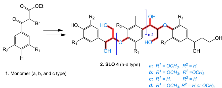
Scheme 2. Mechanisms for the synthesis method of Kishimoto et al. [103,131] Adapted from Ref. [131] Copyright (2008), with permission from RSC.
