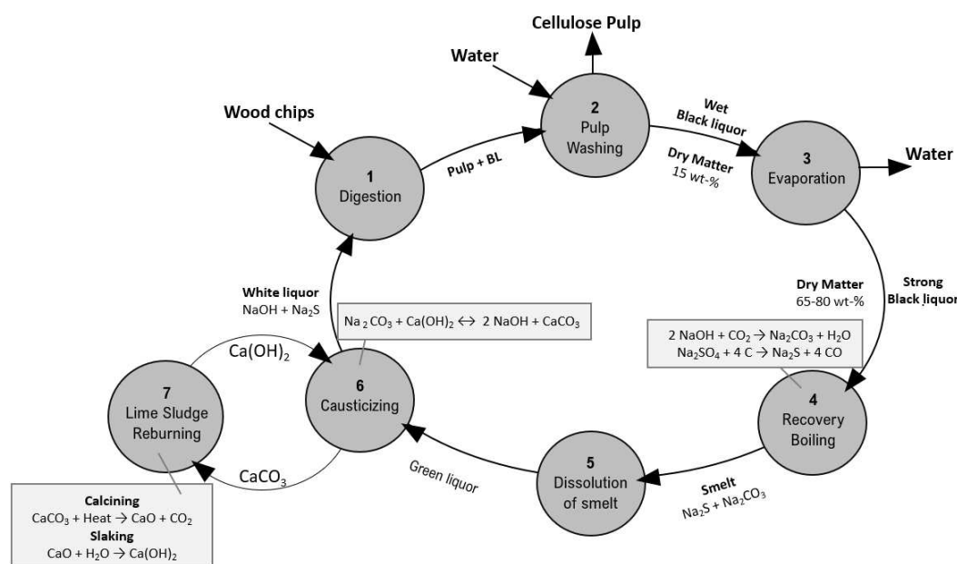
Figure 3. Main material flows in a Kraft pulp mill process. Adapted from Ref. [38] Copyright (1996), with permission from Elsevier.
