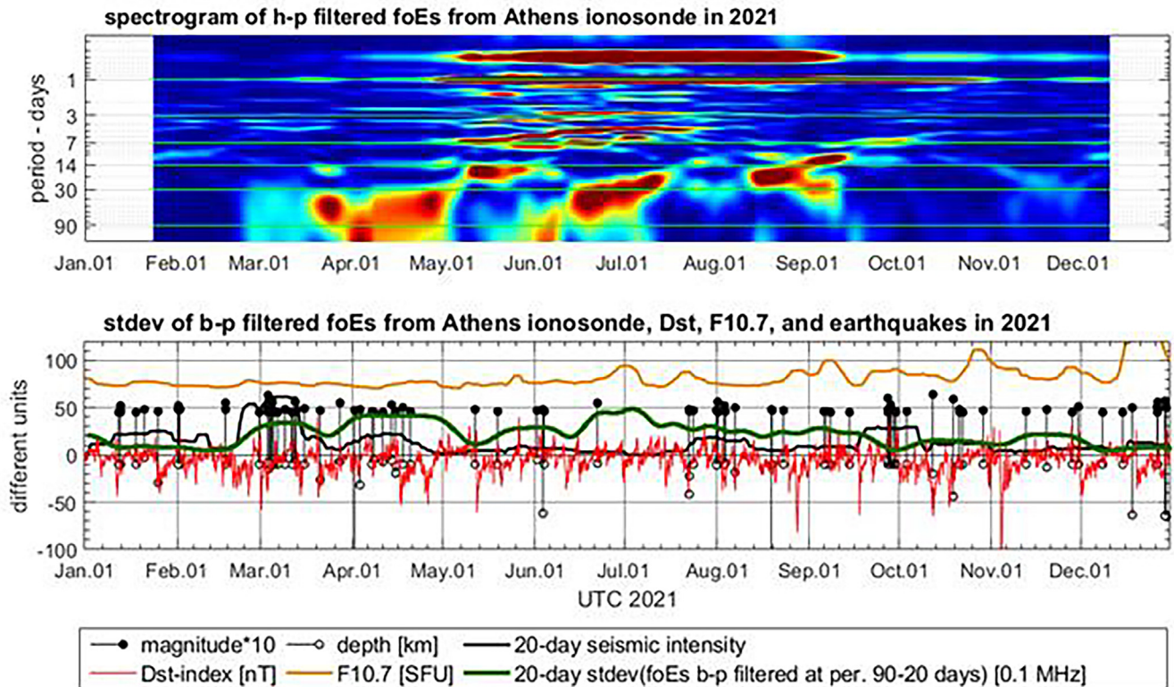
Fig. 9. Results from the sporadic E layer maximum frequency spectrogram from Athens Digisonde presented together with the seismic intensity recorded in the Aegean Sea.
