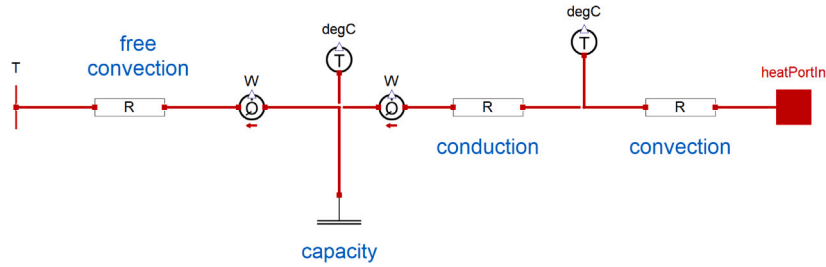
Fig. 4. Heat transfer class: Heat transfer mechanisms convection, conduction and free surface convection are modeled using heat resistances R . Masses and material properties are considered using a heat capacity.
