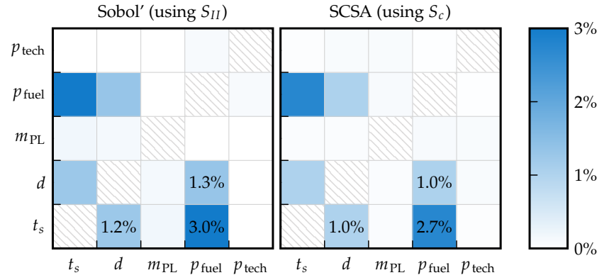
Figure 4.3 Comparison of second order sensitivity measures provided by the variance-based GSA methods using a matrix plot.
