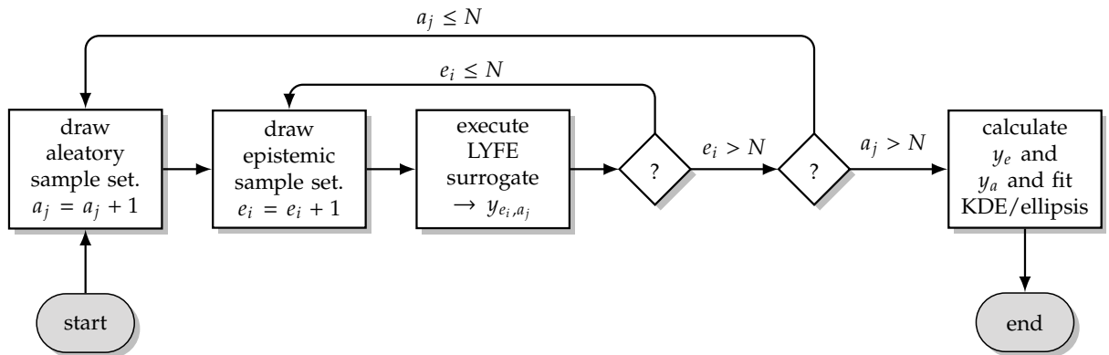
Figure 6.8 Flowchart for novel uncertainty combination approach.
