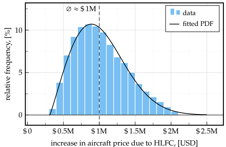
Figure 4.14 Histogram and fitted PDF of the aircraft price increase M_3 due to HLFC with data obtained from different CERs.
