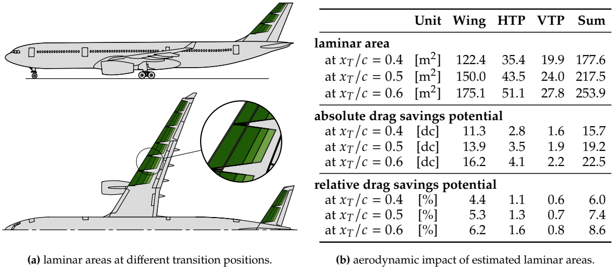
Figure 4.6 Visualization and summary of HLFC application with a transition position x_T/c \in [0.4, 0.5, 0.6] resulting in a uniform distribution of the drag reduction potential \mathcal{D}_1 .
