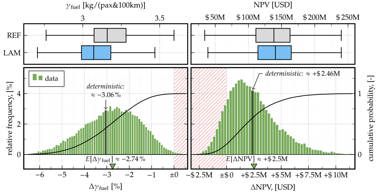
Figure 4.15 Monte-Carlo results of the GSA with fuel efficiencies on the left, NPVs on the right, aircraft design-specific results at the top, and histograms and empirical CDFs of \Delta values at the bottom.
