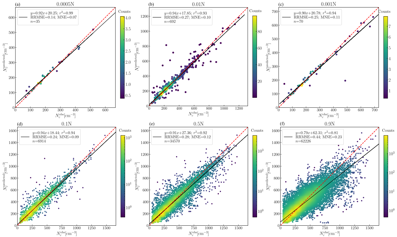
Figure 4. Test of the input sample size for the observation-RFM trained without the corresponding subsamples. The same features N_a , w' , T , and q_v are used as in Figures 2 and 3. The data points for each subsample are randomly selected from the averaged full data set and are excluded from the training data set. N = 69,159 is the size of the full data set.
