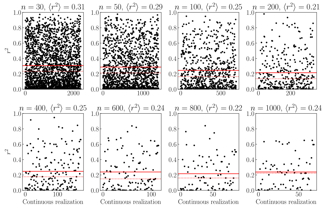
Figure 3. r^2 of N_c = \mathcal{G}(N_a, w', T, q_s) predictions from continuous sampling with different sampling size n using the observation-RFM trained without the subsample. The solid and dashed lines represent mean (denoted as \langle r^2 \rangle in the title of the subplots) and median values of r^2 , respectively. Note that the samples are drawn from running-averaged data set with a window size of 20 data points.
