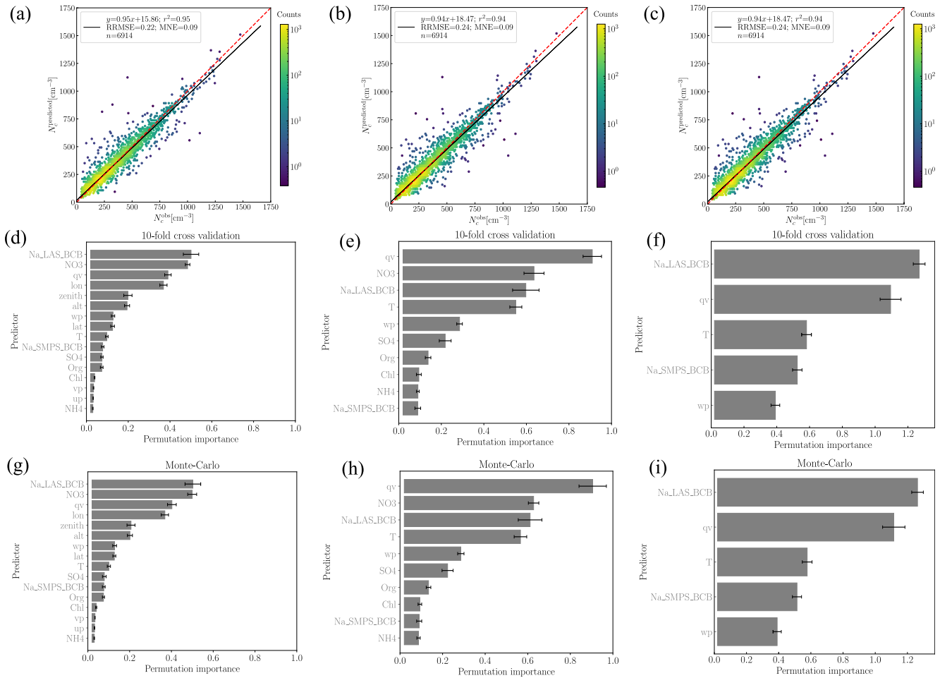
Figure 1. Binned scatter-plot of N_c^{\text{obs}} and N_c^{\text{predicted}} from different predictors (a): N_c = \mathcal{G}(m_{\chi}, N_a, w', u', v', T, q_v, \mathbf{x}, \theta_z) , that is, all available measurements; (b) N_c = \mathcal{G}(m_{\chi}, N_a, w', T, q_v) , and (c) N_c = \mathcal{G}(N_a, w', T, q_v) . Color bar shows the counts of data points in each hexagonal bin. The red dashed line represents the one-to-one line. The solid black line represents the linear regression relation y = ax + b with a and b being the regression coefficients. The test size of the validation data is represented by n in the legend of the scatter-plots. Error bars in the average permutation feature importance (PFI) plots represent \sigma deviation of PFI from the 10-fold and Monte-Carlo cross validations.
