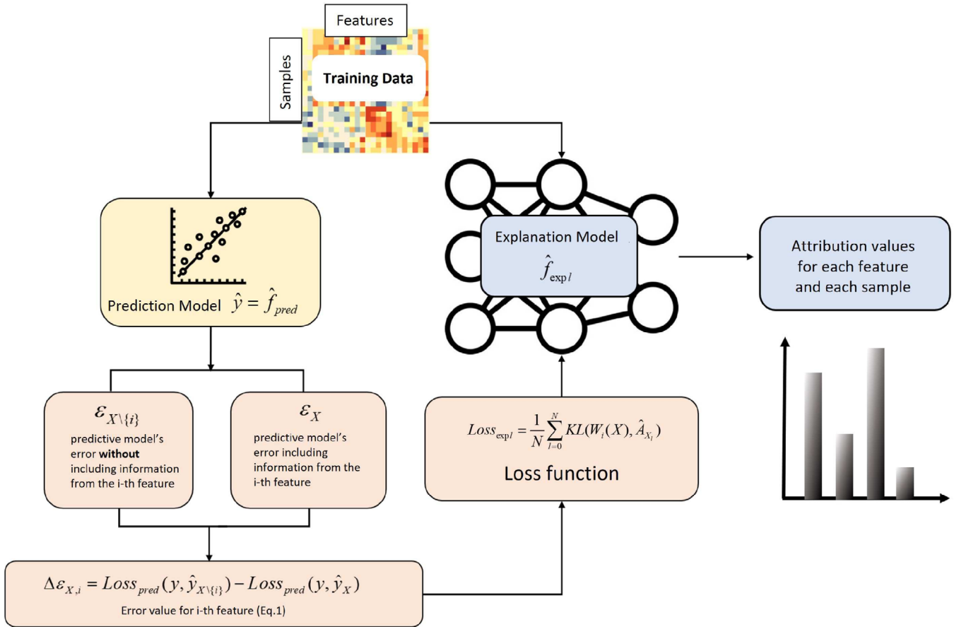
FIGURE 5 | Conceptual diagram of the proposed explanation model.
