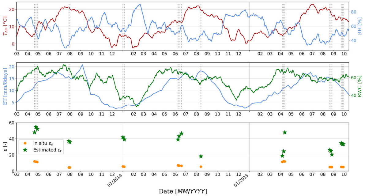
Fig. 8. Seasonal patterns of daily averaged in-situ measured air temperature ( T_{\text{air}} ; ^{\circ}\text{C} ), relative humidity (RH; [%]), MODIS evapotranspiration (ET; [mm/8days]), and AMSR2 relative water content (RWC; [%]) for the period 2013–2015 together with in-situ measured soil permittivity ( \epsilon_s ; [–]) and estimated trunk permittivity ( \epsilon_t ; [–]) at AirMOSS measuring dates of station US-Me2, Metolius, OR. The time series of T_{\text{air}} , RH, and RWC are cleaned for daily dynamics using the Savitzky-Golay filter with a window size of 21 (days), the MODIS ET time series with a window size of three (21 days). Dashed grey lines in the first two subplots indicate the dates of available AirMOSS measurements.
