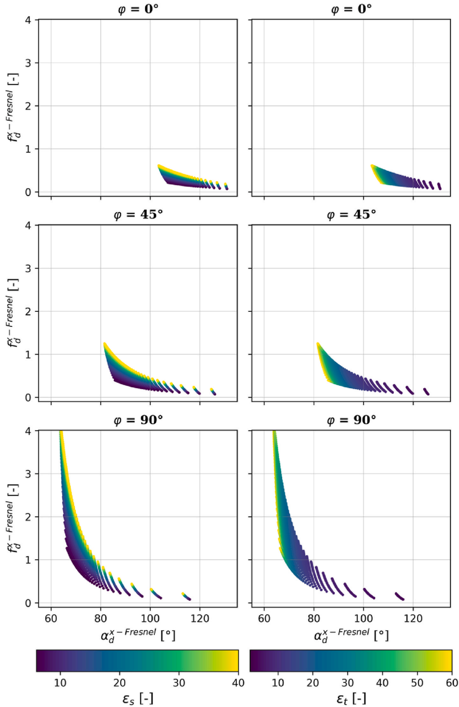
Fig. 3. Sensitivity of the simulated dihedral scattering angle \alpha_d^{x-Fresnel} and intensity f_d^{x-Fresnel} on the soil ( \varepsilon_s \in [6, 40] ) and trunk ( \varepsilon_t \in [2, 60] ) permittivity as well as the phase angle \varphi \in [0, 45, 90]^\circ . In this example, f = 430 MHz, \theta_i = 30^\circ , m_d = 1 , and \theta_1 = 0^\circ .
