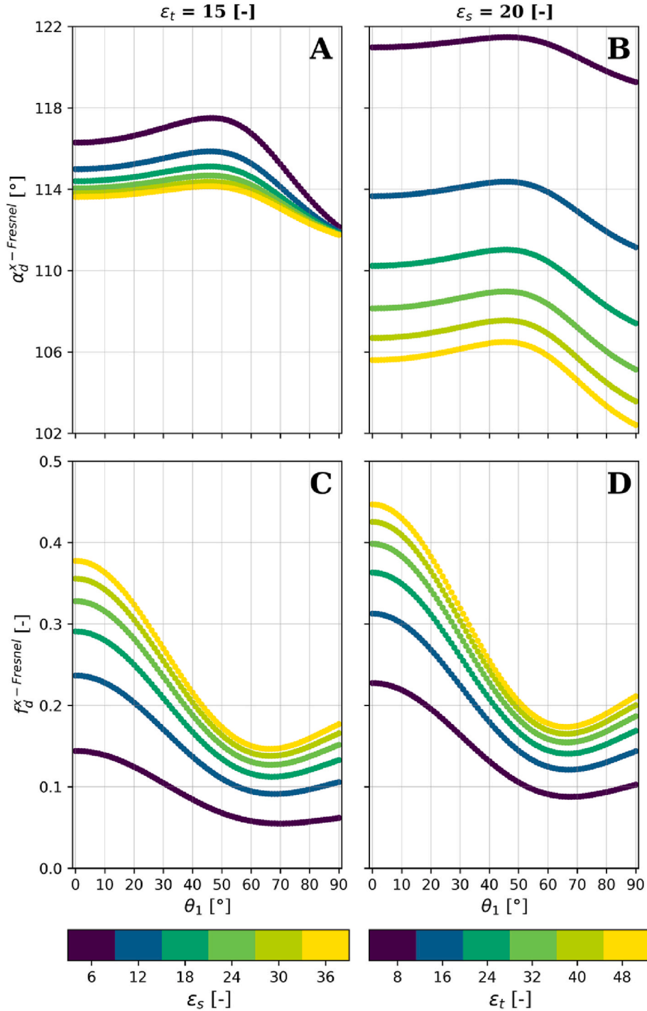
Fig. 4. Sensitivity of the simulated dihedral scattering angle \alpha_d^{x-Fresnel} and intensity f_d^{x-Fresnel} on the rotation limit angle \theta_1 [°] and the soil \varepsilon_s and trunk \varepsilon_t permittivity. In this example, \theta_i = 30^\circ , m_d = 1 , and \varphi = 0^\circ . (A) Results for \alpha_d^{x-Fresnel} with \varepsilon_t = 15 and \varepsilon_s \in [6, 36] . (B) Results for \alpha_d^{x-Fresnel} with \varepsilon_s = 20 and \varepsilon_t \in [8, 48] . (C) Results for f_d^{x-Fresnel} with \varepsilon_t = 15 and \varepsilon_s \in [6, 36] . (D) Results for f_d^{x-Fresnel} with \varepsilon_s = 20 and \varepsilon_t \in [8, 48] .
