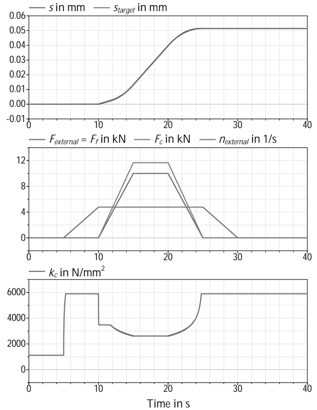
Figure 6: The results for the drilling process based on the dynamics model. The image shows the actual and target position for the drill (top), the external force, the cutting force and the rotational frequency (middle), and the specific cutting force (bottom).
