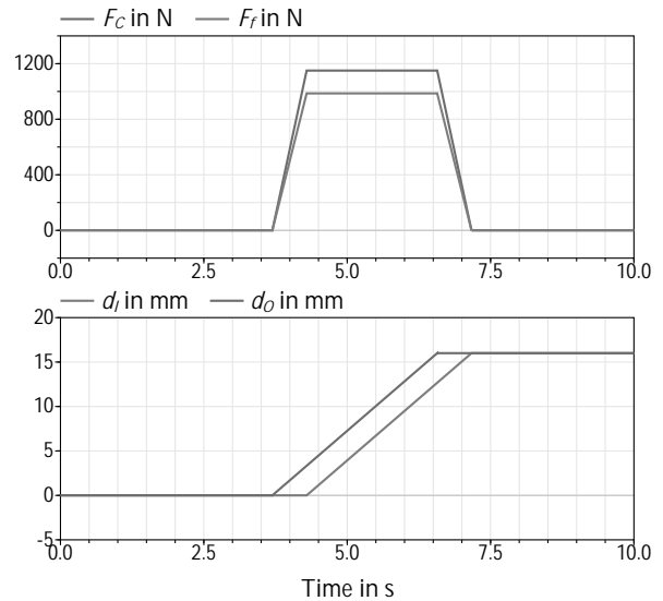
Figure 4: Results for the drilling process of a thin plate. The cutting force and the feed force are shown above. The drilling diameters are shown at the bottom.
