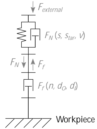
Figure 2: A substitute model of the drilling force model. An external force is applied to the spring-damper element representing the contact model. The contact force is equal to the feed force of the drilling force model, here represented by a damper element, with the damping force dependent on the rotational frequency and the drill diameters.
