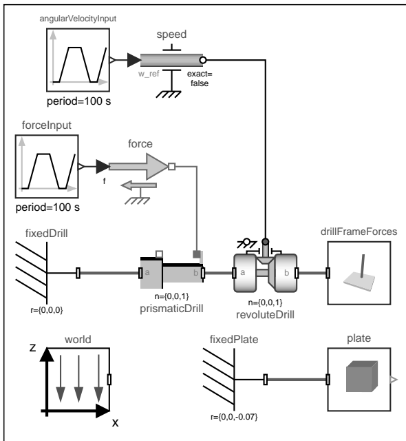
Figure 5: The Modelica model of the drilling process based on the dynamics model. The drilling model applies the forces directly to the frame. An external force and angular velocity are also applied to the frame.
