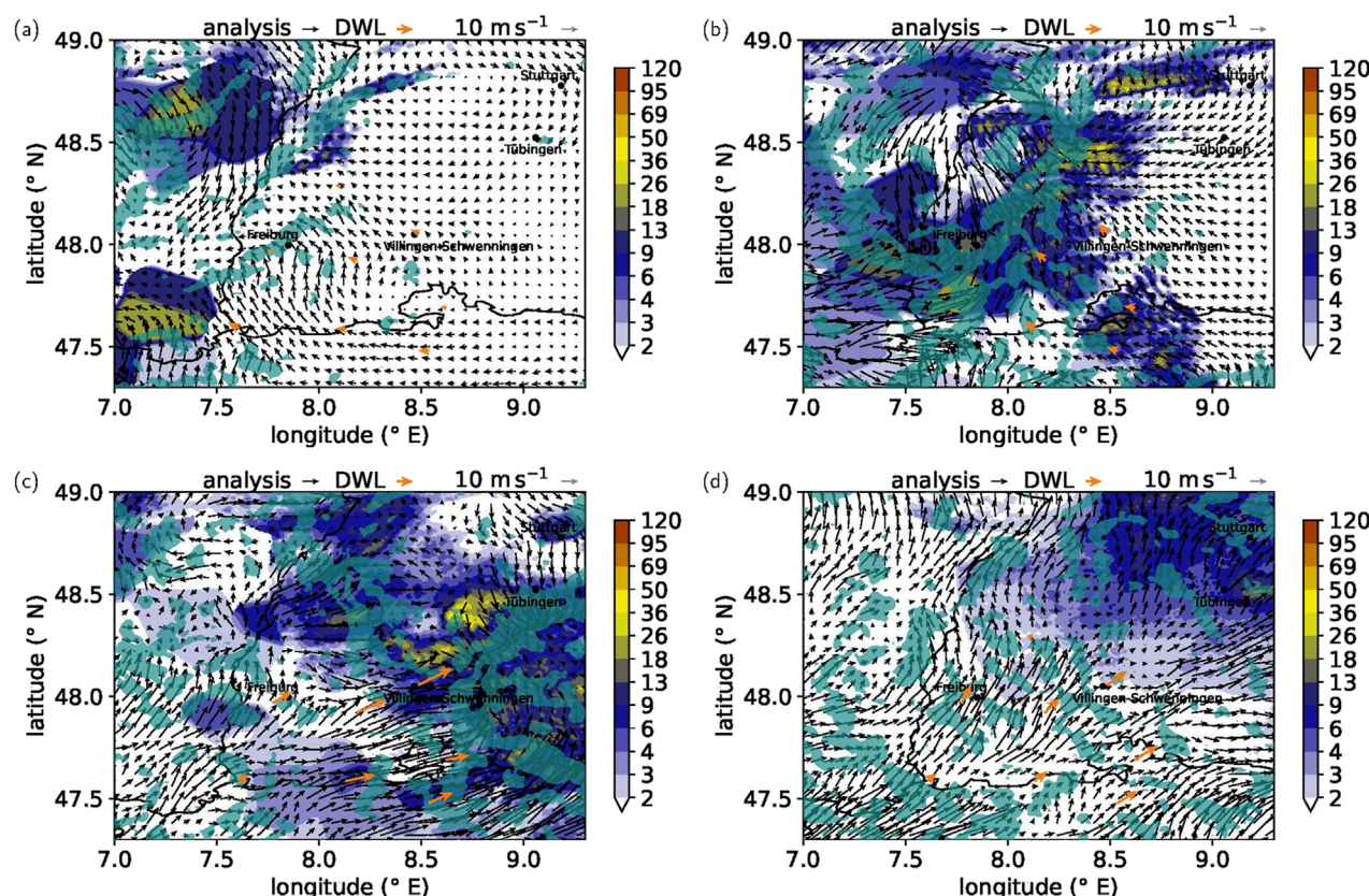
FIGURE 5 ICON-D2 analysis wind field 500 m agl (black arrows) and wind convergence larger than 3.5 \cdot 10^{-4} \text{ s}^{-1} (turquoise shades) on 11 July from 18:00 UTC (a) to 21:00 UTC (d) with 60-min RADOLAN precipitation rate (in \text{mm h}^{-1} , colors). Precipitation is accumulated approximately from the time shown in (a–d) plus 1 h. The orange arrows show the observed wind field at Doppler wind lidar sites.
