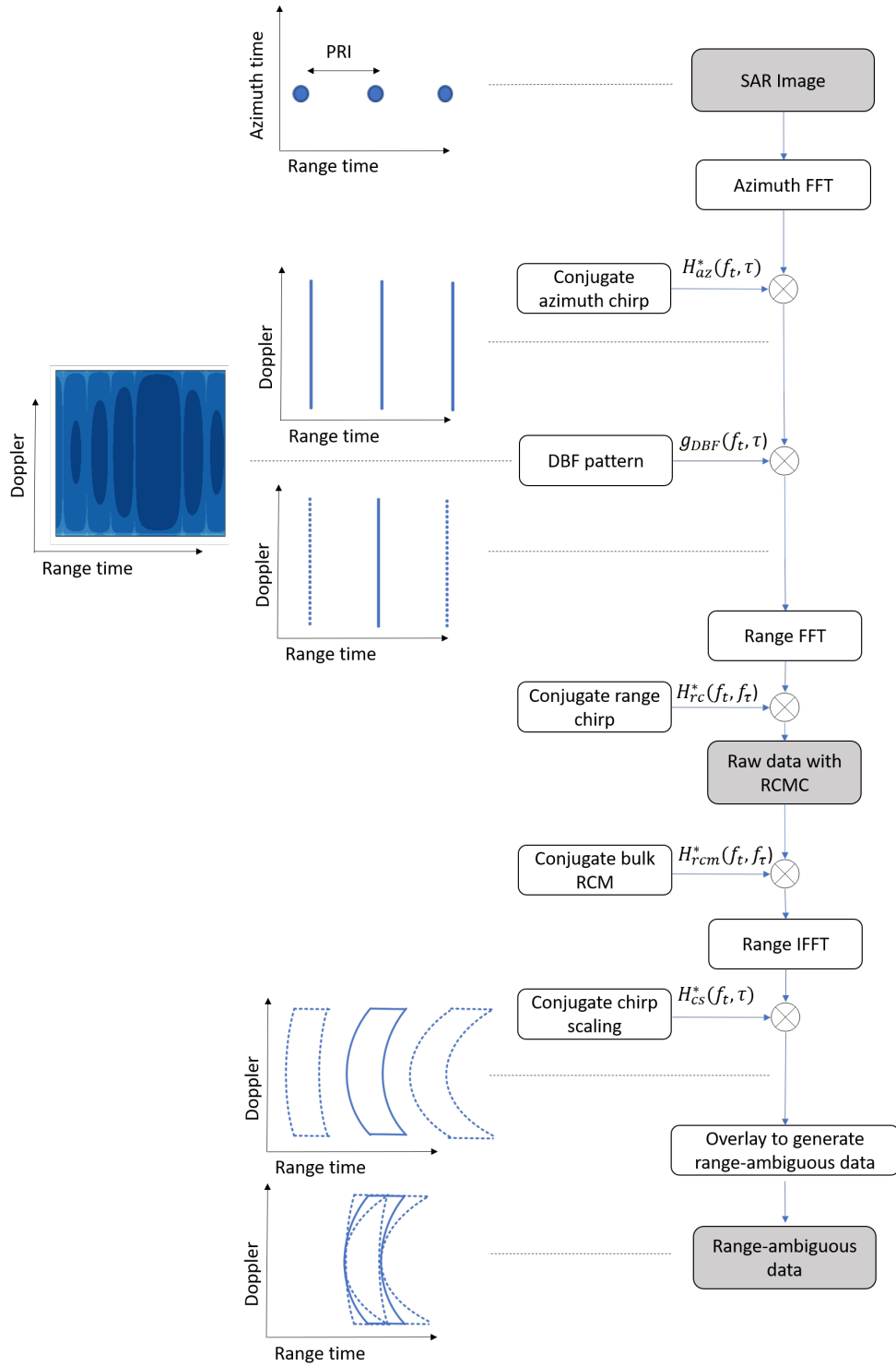
Figure 5.1: Flowchart illustrating the process of generating range-ambiguous raw data for a single swath (right), including the target's response representation (left). On the left, the useful target and the range-ambiguous target are represented by solid and dashed curves, respectively.
