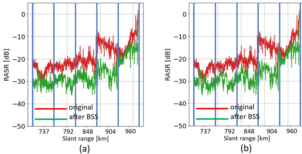
Figure 5.24: Comparison of RASR performance when the order of implementing two strategies is reversed: (a) azimuth sub-band approach implemented first, followed by the stacking approach, as seen in Figure 5.22(c); and (b) stacking approach implemented first, followed by the azimuth sub-band approach.
