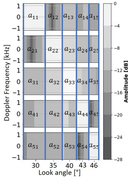
Figure 5.12: Mixing matrix, \mathbf{A}_{PLA} , extracted from SCORE DBF antenna patterns. The blue vertical lines indicate the boundary between the simulated swath segments.
