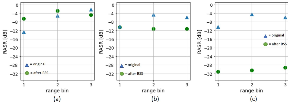
Figure 3.9: RASR performance of BSS in (a) raw signals, (b) range-compressed signals, and (c) fully focused signals. In (b), the RASR values in range bin 1, before and after the BSS method, is superimposed.
