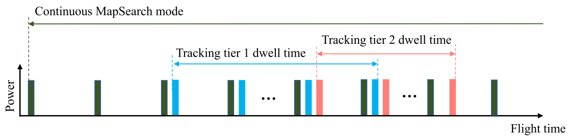
Figure 3.9: Timing example showing the transmit pulses of the interleaved ADOB-SAR modes: the continuous MapSearch and two Tracking tiers with specific dwell times.
