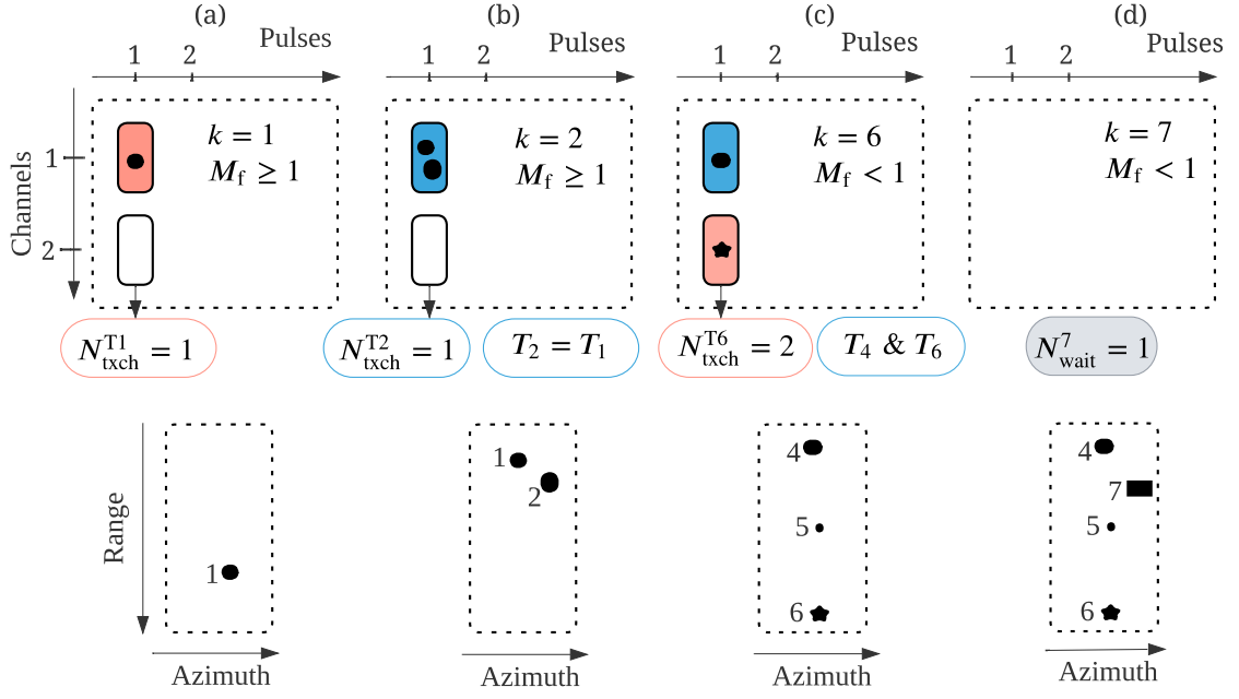
Figure 6.22: Examples of transmit channel configurations for different target scenarios and free time margins based on the three beam assignment conditions.
