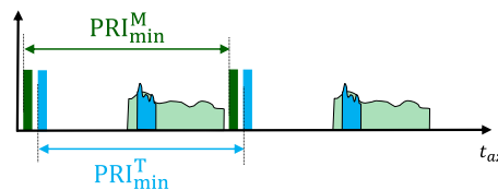
Figure 6.15: The maximum Tracking PRF, which is defined as the maximum MapSearch PRF that satisfies the range ambiguity-free timing within the swath, defined in (5.10).
