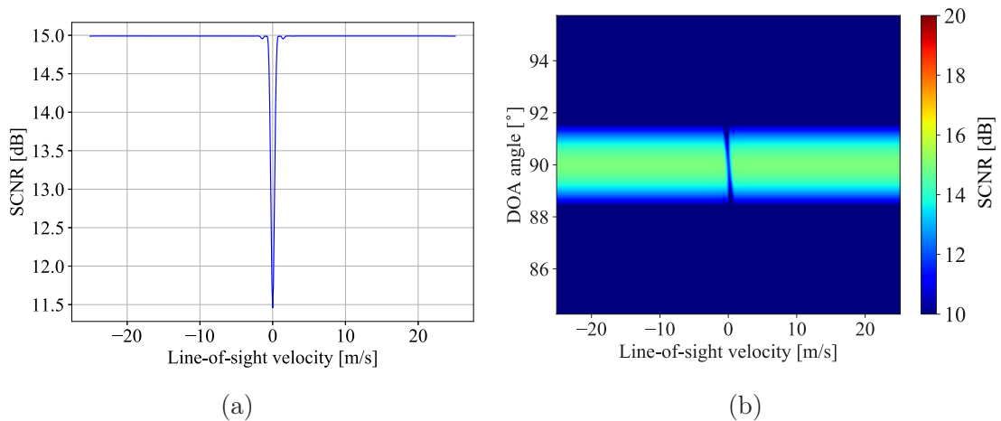
Figure 7.8: Simulated SCNR during the MapSearch mode over the line-of-sight target velocity for a duty cycle of 2.25% and a PRF of 1800 Hz. In (a), the SCNR is plotted as a cut over the broadside direction of the antenna array. (b) shows the output SCNR of one azimuth receive channel.
