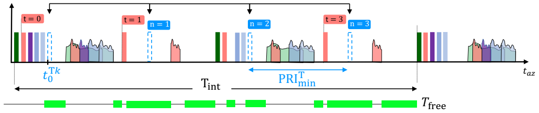
Figure 6.17: Timing schedule snapshot highlighting the condition on using the maximum Tracking PRF for a new target k , given the start time of its first transmitted pulse t_0^{\text{Tk}} .
