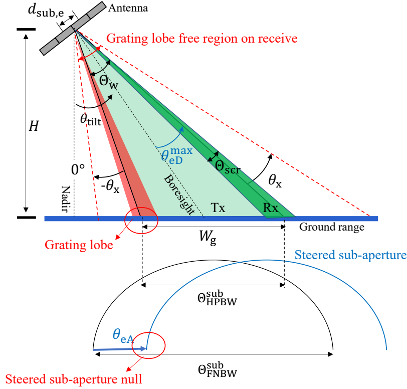
Figure 4.28: Elevation geometry of the SCORE Hybrid Beamforming method 2, where the sub-aperture pattern with the beamwidth \Theta_{\text{HPBW}}^{\text{sub}} = \Theta_w is steered to \theta_e^{\text{max}} to place its first null at the grating lobe caused by the digital SCORE steering.
