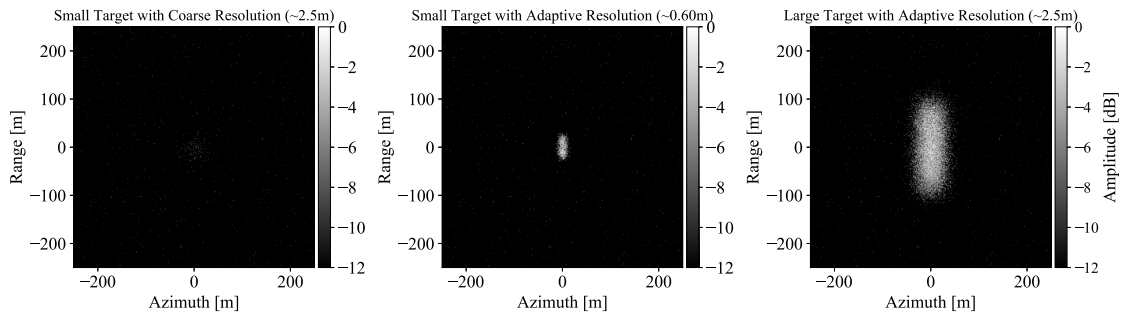
Figure 6.3: SAR simulated images of different targets (small: 20 \text{ m}^2 and large: 400 \text{ m}^2 ) with various adaptive resolutions based on their sizes.
