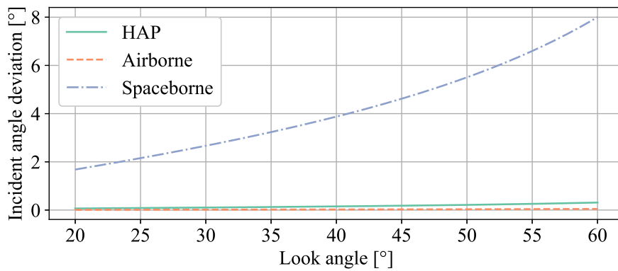
Figure 3.3: Comparison between the incident angle deviations caused by a non-flat Earth for a high-altitude with 20 km, airborne with 3 km, and spaceborne platform with 540 km altitude.
