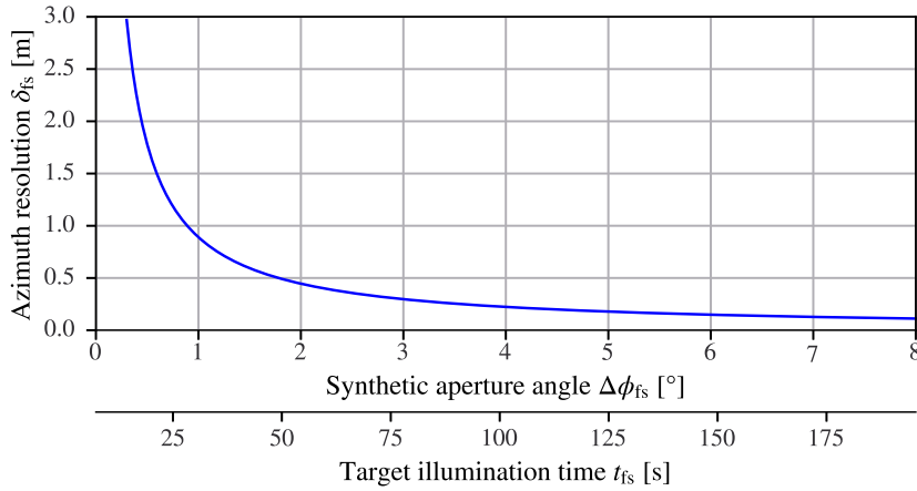
Figure 4.34: Azimuth resolution of the Follow Spot SAR imaging mode plotted versus the synthetic aperture angle \Delta\phi_{fs} and illumination time t_{fs} .
