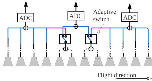
Figure 4.42: A schematic of the reconfigurable antenna array architecture on receive. The number of channels can be changed adaptively depending on the mode.
