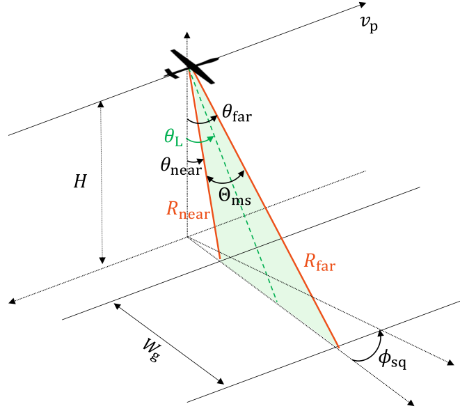
Figure 4.12: 2-D geometry featuring the elevation parameters of the boresight direction, the near and far slant ranges R_{near} and R_{far} and their corresponding looking angles \theta_L , \theta_{near} , and \theta_{far} taking into consideration the platform altitude H .
