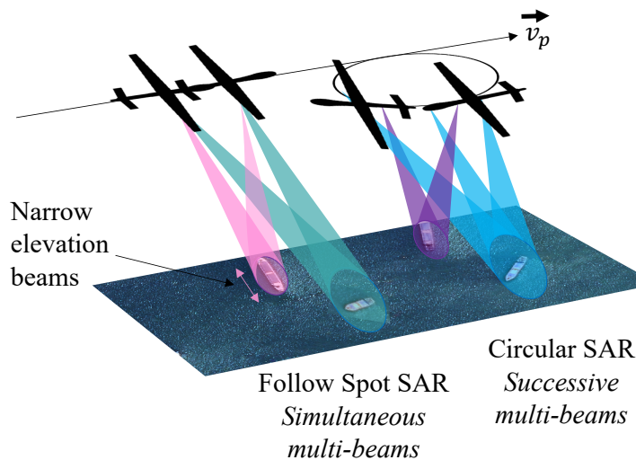
Figure 4.32: Schematic representation of the Tracking mode imaging techniques: Follow Spot SAR and Circular SAR with simultaneous or successive multi-beams.
