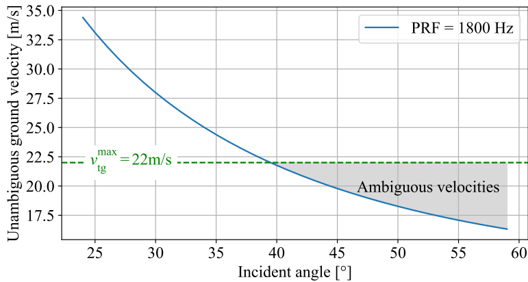
Figure 7.6: Maximum unambiguous velocities versus the incident angle for the selected MapSearch PRF of 1800 Hz.
