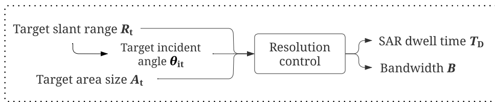
Figure 6.5: Schematic representation of the resolution control process, where the bandwidth and the SAR dwell time are adapted for each target depending on its slant range, size, and incident angle, as given in (6.3) and (6.4).
