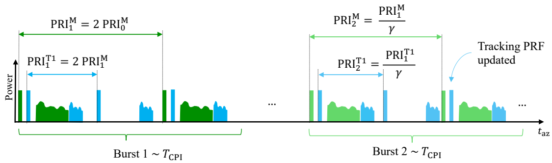
Figure 5.14: Tracking PRF update when the burst mode with PRF alternating is activated according to Section 5.1.4. In burst 2, the Tracking PRF of tier 1 is changed according to the condition (5.26).
