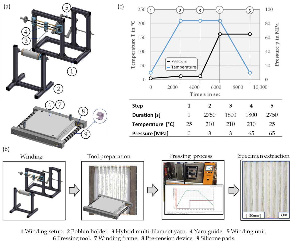
Figure 3. (a) Winding unit and press tool adapted to the tape geometry, (b) process overview of the tape manufacturing, and (c) time-temperature profile of the press process.
