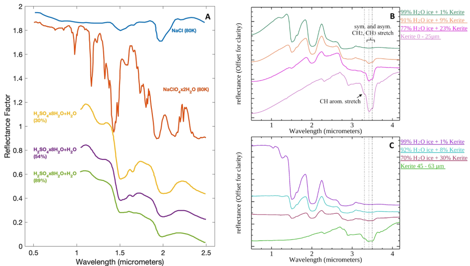
Fig. 2 (A) Spectra of Cl-salts (Hanley et al. 2014) compared to hydrated sulfuric acid (Carlson et al. 1999a). Spectra of typical bitumen kerite (grain sized range 0–25 \mu\text{m} in (B) and 45–63 \mu\text{m} in (C)) measured at 173 K with varying portions of water ice (Ciarniello et al. 2021). Spectra illustrate the detectability of the typical absorptions related to aromatic CH, and \text{CH}_2/\text{CH}_3 aliphatic/aromatic symmetric and asymmetric stretch (contributing to complex broad band between 3.18 and 3.64 \mu\text{m} ) as indicated by the dashed lines depending on grain size of kerite and varying portions of water ice
