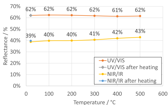
Fig. 4. Effective reflectance values obtained from spectral weighting with the spectrum of the Xe short arc based solar simulator for the UV/VIS range and with a black-body spectrum at 600 °C for the NIR/IR range, respectively.
