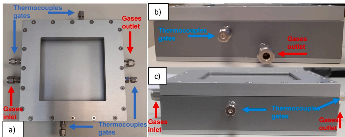
Fig. 2. Images of the photo-thermal reactor from a) the top, b) the right side and c) the front side highlighting the locations of gas inlet, outlet, and thermocouple ports.
