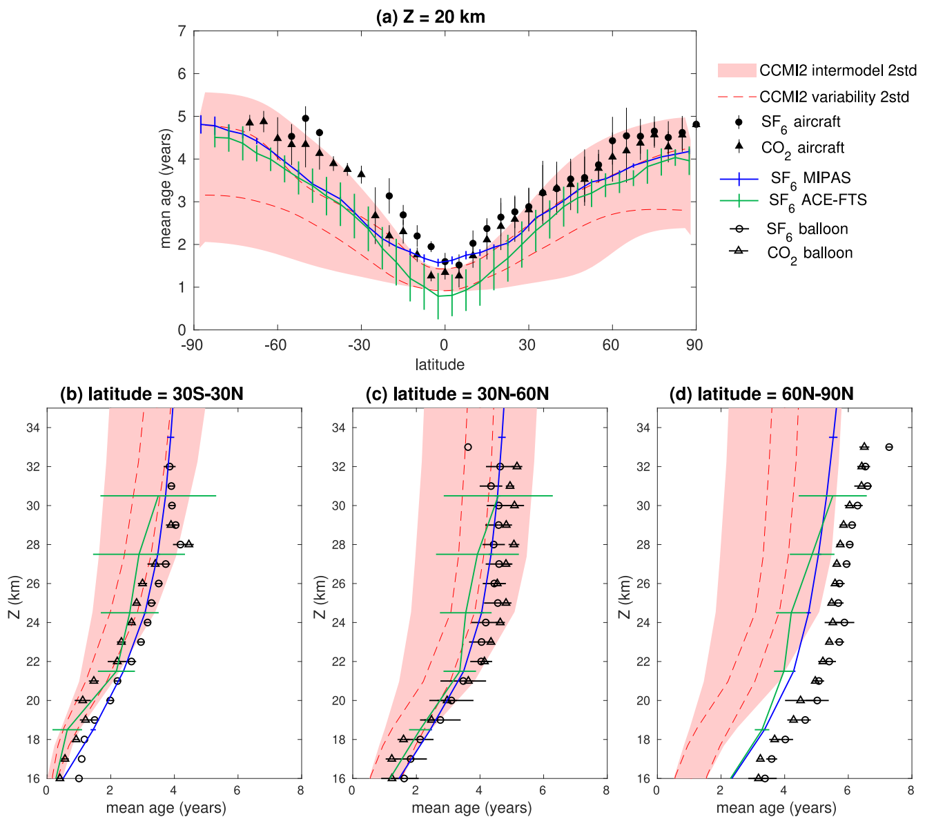
Figure 10. (a) Latitudinal structure of mean age of air at 20 km from observations and models as a function of latitude. (b–d) Mean age vertical profiles in the tropics (30°S–30°N), mid-latitudes (30°N–60°N) and high latitudes (60°N–90°N). In situ aircraft and balloon observations as described in Section 4.4, (black symbols), satellite estimates include MIPAS (blue) and Atmospheric Chemistry Experiment Fourier Transform Spectrometer (green). All SF 6 -based ages have been corrected for the chemical sink. Model data is from CCM2 refD1 simulations from 6 models, averaged over 1975 to 2018, with the intermodel spread shown as the two standard deviation range across models (shading), and the interannual and intraseasonal variability is shown as the two standard deviation averaged for all models (dashed lines).
