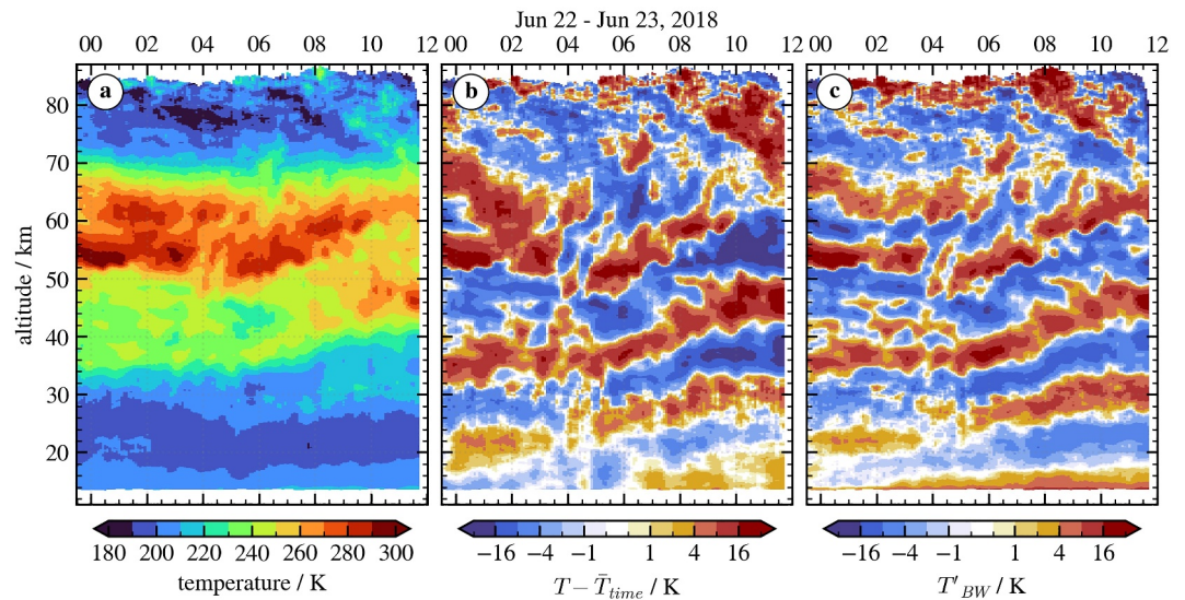
Figure 5. Night-time temperature measurements of CORAL located in Río Grande, Argentina (53.79°S, 67.75°W) from June 22 to 23, 2018. Shown are retrieved temperature profiles (a), temperature perturbations T' = T - \bar{T}_{time} after subtracting a nightly (temporal) mean (b) and T' after applying a vertical high-pass Butterworth filter with a cutoff wavelength of \lambda_{z,cut} = 20 km (c).
