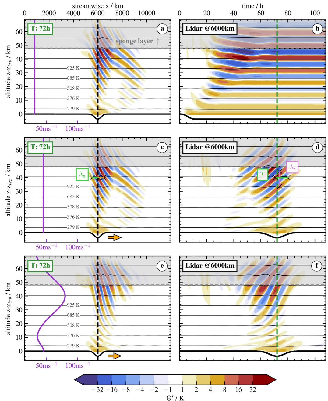
Figure 1. Vertical cross-sections (a), (c) and (e) after t = 72 hr with ambient wind profiles in purple and time-height diagrams (b), (d) and (f) at the outlined position for three different simulations. The first simulation (a) and (b) features a stationary obstacle at the lower boundary and a constant wind profile. In the second simulation (c) and (d) the trough moves to the right with a constant speed c_{eff} = 13.88 \text{ m s}^{-1} and the wind is increased by the same amount. The last simulation (e) and (f) represents a simulation with a more realistic stratospheric wintertime wind profile. The assessment of \lambda_z and period T from the time-height diagram is labeled in (d), two consecutive \lambda_x are labeled in (c). Contour lines represent constant potential temperature and the amplitude of the lower boundary is scaled by a factor of 5.
