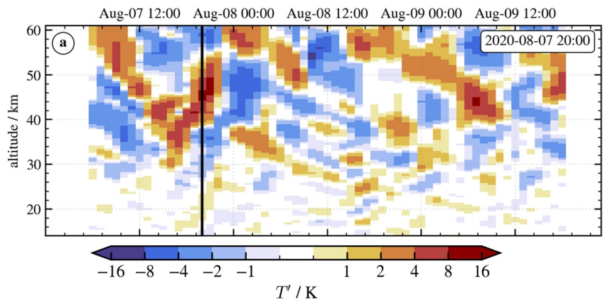
Figure 9. Time-height diagram that mimics the measurement of a zenith-pointing lidar for the same period as in Figure 8(a) but for a virtual lidar location west of CORAL's location over the Pacific Ocean (new Longitude: 92.5°W). Again, temperature perturbations are obtained by subtracting a 12 hr running mean. A corresponding time series of the ERA5 composition similar to Figure 8 is available through the Zenodo repository (Binder & Dörnbrack, 2023).
