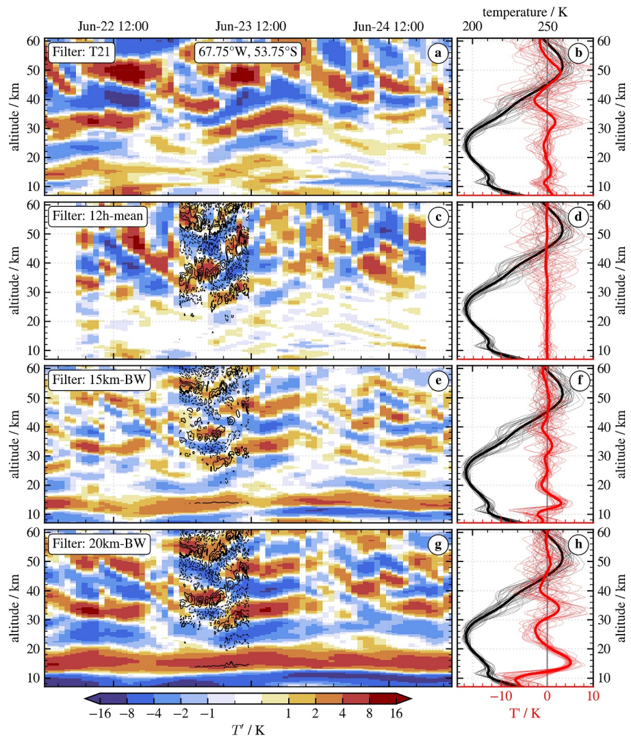
Figure 10. Similar composition as Figure 2 showing time-height diagrams for CORAL's location for a 3-day period in June 2018. Thin black lines show corresponding temperature perturbations from CORAL measurements. Solid lines refer to positive, dashed lines to negative perturbations.
