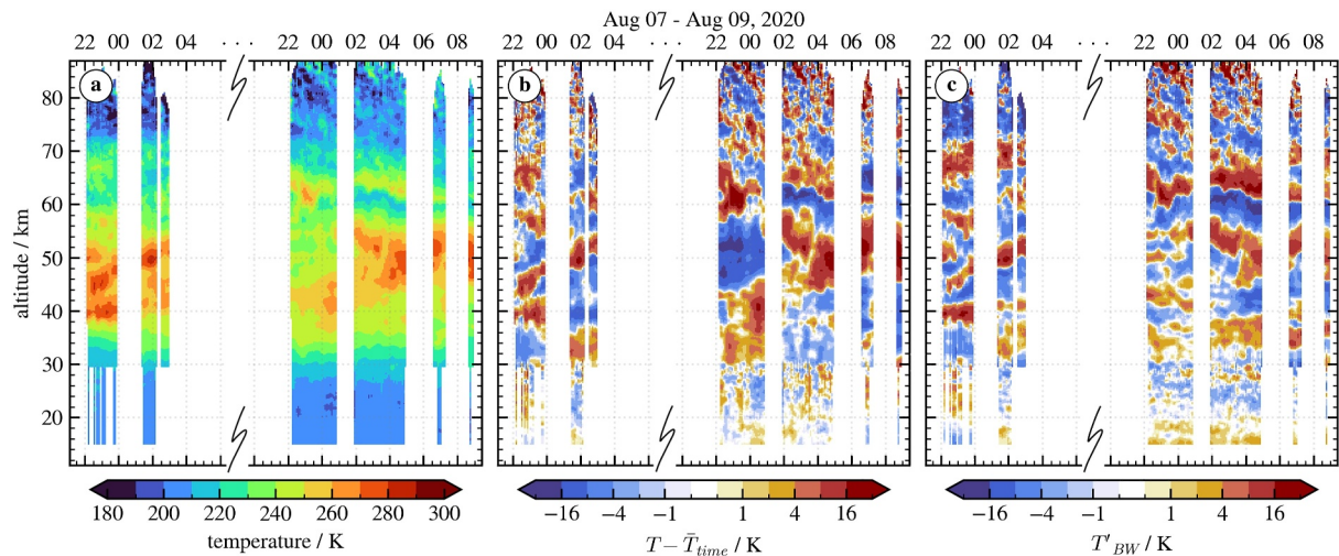
Figure 6. Identical to Figure 5 showing night-time measurements for two consecutive nights from August 7 to 9, 2020. The time frame between the measurements (06:00–20:00 UTC on 8 August 2020) is removed and periods of missing data are related to cloud coverage.
