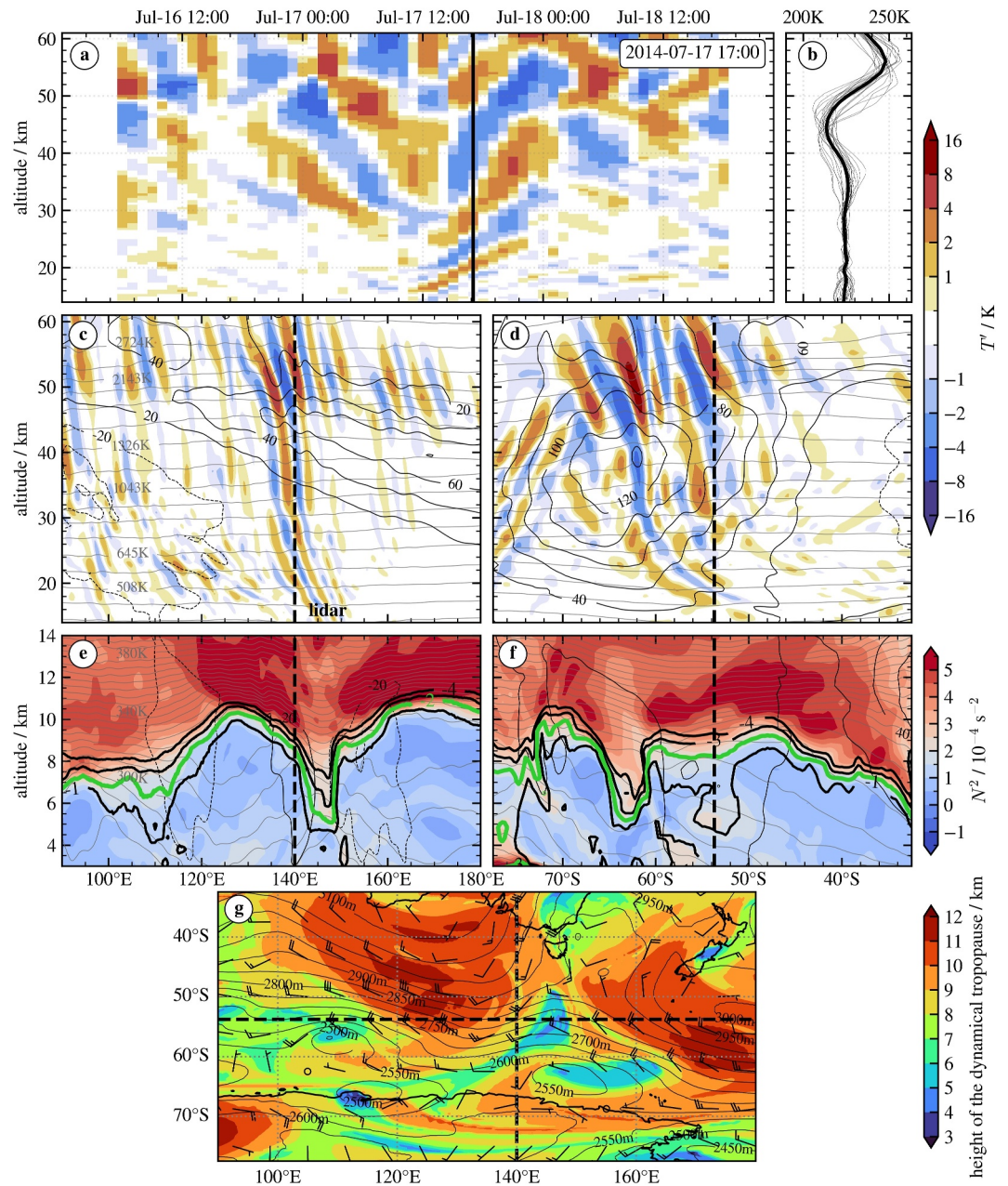
Figure 4. ERA5 overview for a location over the Southern Ocean (53.75°S, 140°E) during research flight RF25 of the DEEPWAVE campaign. Panels (a) and (b) are similar to Figures 2(c) and 2(d) emulating the measurements of a vertically staring ground-based lidar. Panels (c) and (d) are vertical sections of stratospheric T^p along sectors of the latitude circle (c) and meridian (d) of the virtual lidar location. (e) and (f) are corresponding vertical sections of thermal stability N^2 ( 10^{-4} \text{ s}^{-2} , color-coded), potential temperature (K, thin gray lines), and potential vorticity (1, 2, 4 PVU: black, 2 PVU: green) in the vicinity of the dynamical tropopause. Thin black lines in the vertical sections are zonal (d) and meridional (e) and (f) wind components (solid: positive, dashed: negative). Panel (g) is a horizontal section of the height of the 2 PVU surface (km, color-coded), geopotential height (m, solid lines) and wind barbs at the 850 hPa level. The black vertical line in (a) marks the time (17 July 2014, 17 UTC) for (c)–(g) and dashed lines in (c)–(g) highlight the location of the virtual lidar and profiles in (a) and (b).
