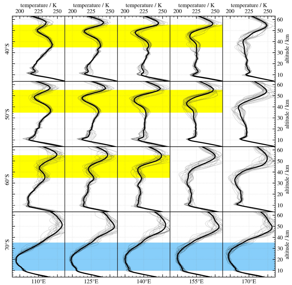
Figure 3. Latitude-longitude matrix of vertical temperature profiles of ERA5 at 20 evenly spaced locations in the Southern Hemisphere. The period 7 July 2014–9 July 2014 includes DEEPWAVE research flight RF25. Thick black lines are temporal mean profiles, thin black lines represent individual profiles every 2 hr for the 3-day period. The yellow band indicates profiles with a pronounced temperature minimum between 35 and 55 km complicating the application of vertical filters to separate the signal into background and GWs. The blue band marks profiles with a significant temperature decrease in the stratosphere due to the polar vortex.
