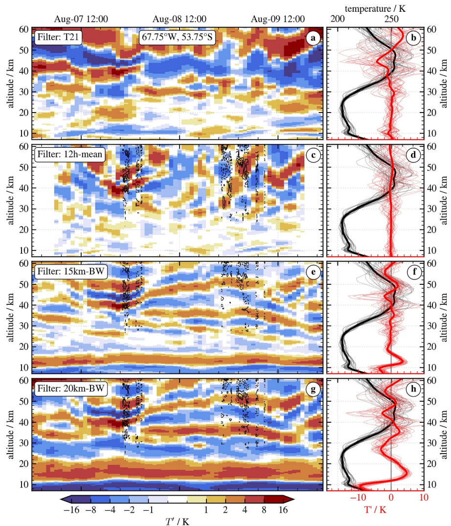
Figure 11. Identical to Figure 10 showing time-height diagrams for CORAL's location for a 3-day period in August 2020 with two consecutive nights with CORAL measurements.
