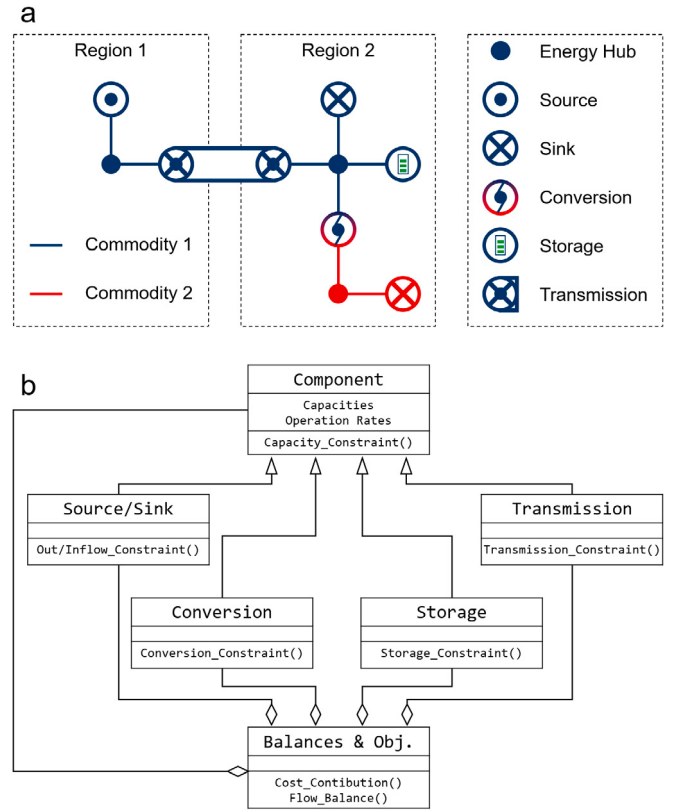
Fig. 5. (a): a demonstrative multi-nodal energy system model with basic components for supply, demand, conversion, storage, and transmission between regions; (b): a typical framework architecture in which specialized components inherit from a general component class and whose costs and inputs or outputs contribute to the objective function and energy balances, respectively.
