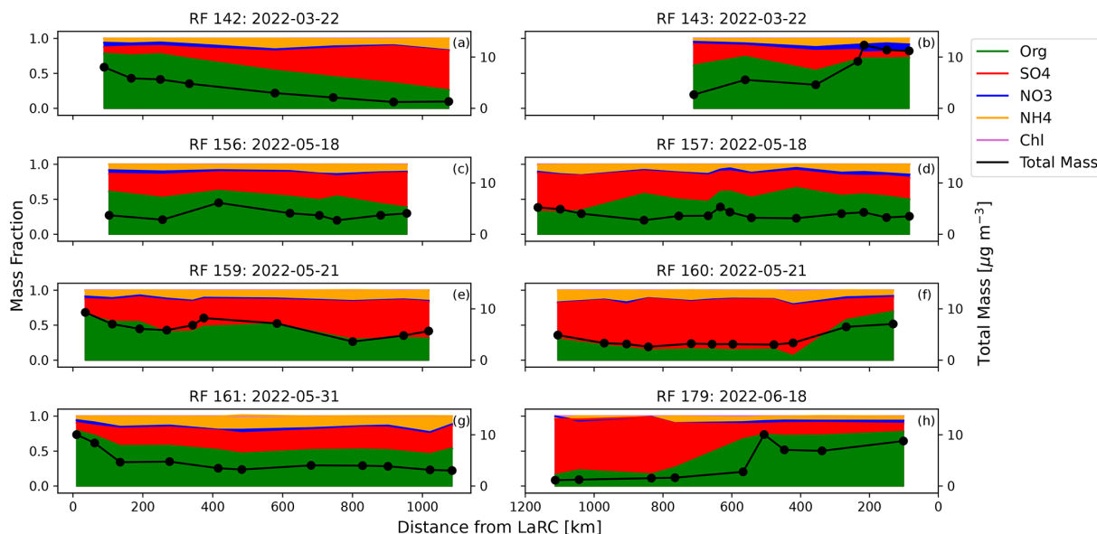
Figure 13. Speciated mass fractions for submicrometer non-refractory aerosol components as measured by the AMS in the BL. Total AMS non-refractory aerosol mass is displayed with black line. Data averaged across 10 min time intervals.
