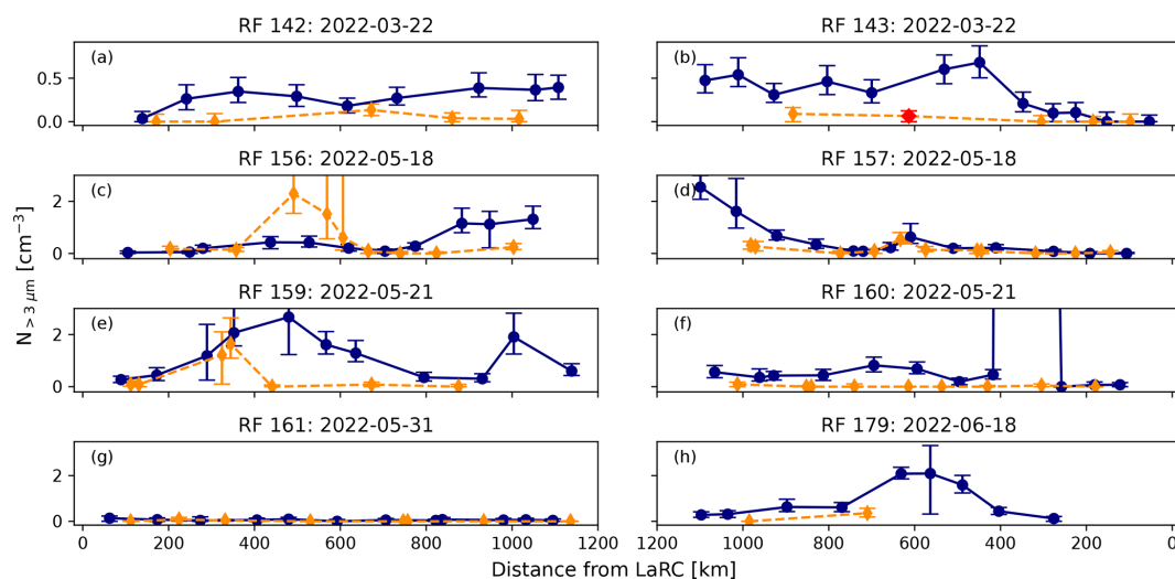
Figure 8. The same as Fig. 6 but for D_p > 3 \mu\text{m} .
