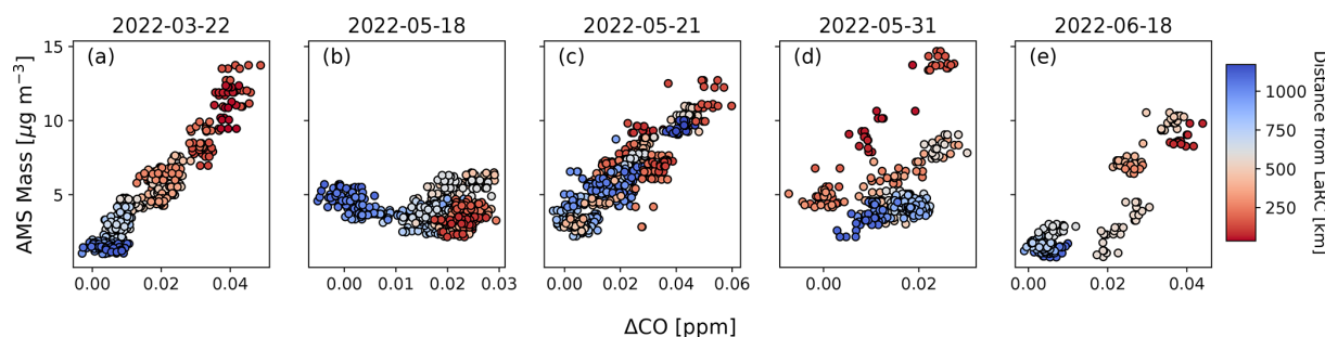
Figure 15. BL total AMS submicrometer non-refractory mass versus \Delta\text{CO} colored by distance relative to the LaRC.
