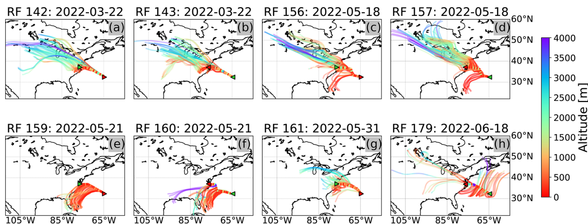
Figure 2. HYSPLIT 3 d back-trajectories ending at the location of the Falcon aircraft along its flight path. The altitude of the air mass is shown by color bar.
