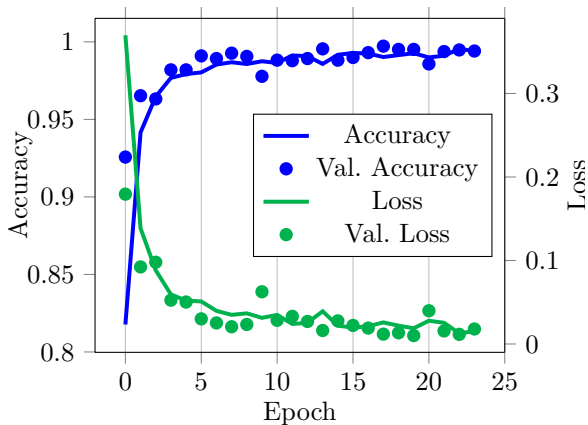
Fig. 9 Training and validation accuracy and loss of the best CNN model from the AC 2-class classifier gridsearch
