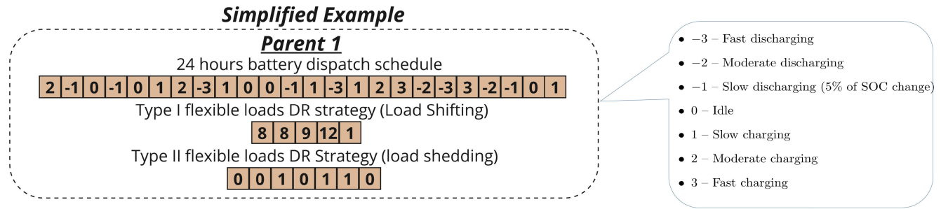
FIGURE 8. Example-Chromosome representation in the genetic algorithm.
