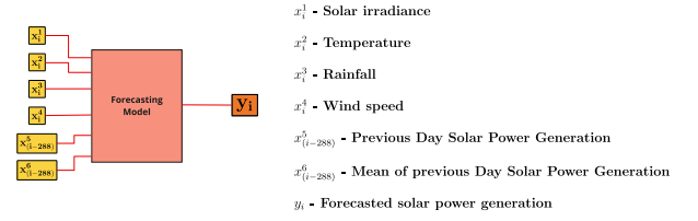
FIGURE 6. Solar forecasting model.
