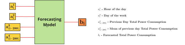
FIGURE 7. Building load forecasting model.
