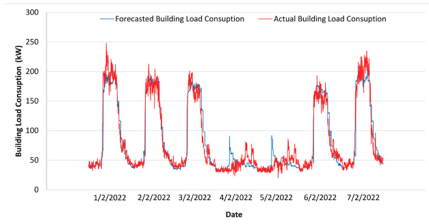
FIGURE 14. Load consumption forecasting.
