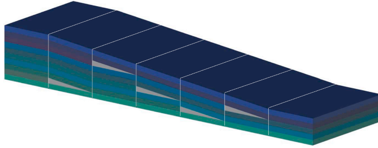
Figure 1: Blended laminate structure [6]
