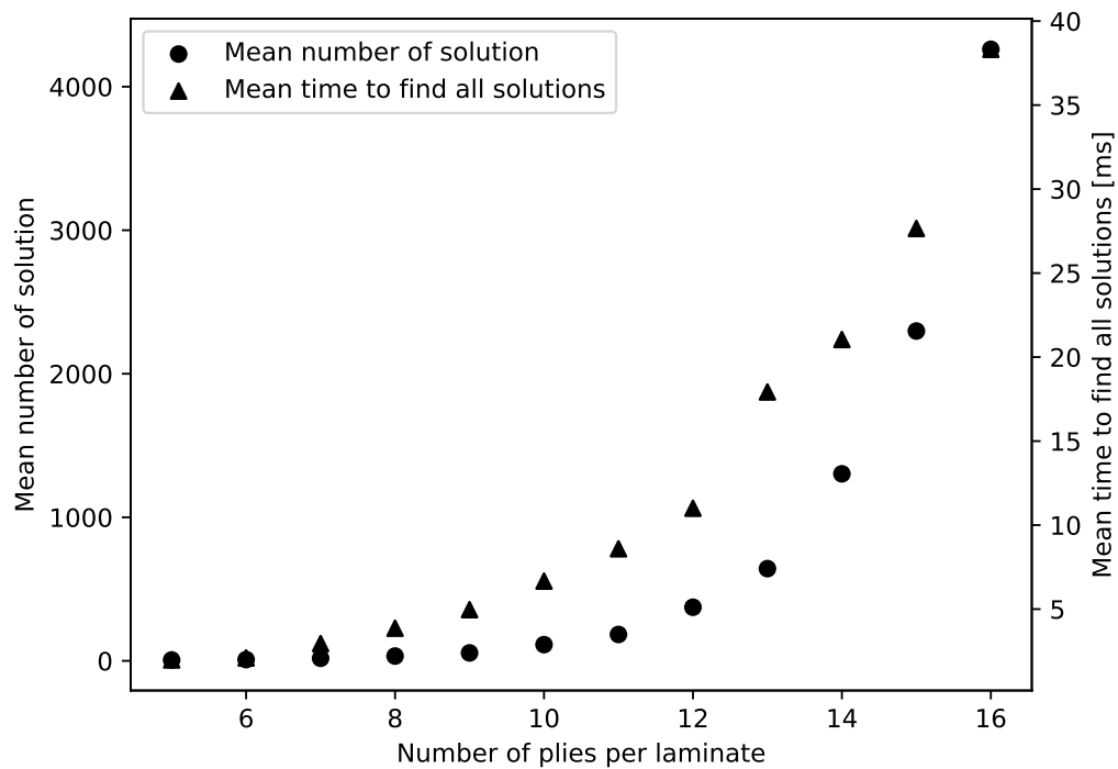
Figure 26: Number of solutions computation time with randomly generated laminates with different stacking sizes
