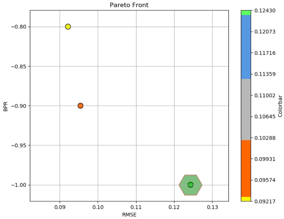
Figure 32: Pareto Front of wing box use case
