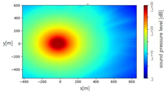
Figure 8: Simulated sound pressure level on the ground for Harsewinkel.
