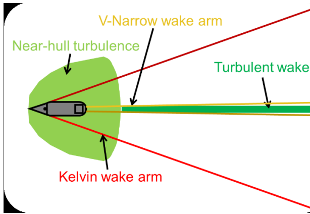
FIGURE 2. SCHEMATIC REPRESENTATION OF FOUR WAKE COMPONENTS MOST FREQUENTLY DETECTABLE IN SAR IMAGERY
