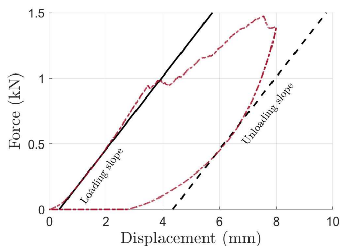
Figure 7. Illustration of slopes measurements during loading and unloading in Quasi-Static Indentation (QSI) tests of wood veneer laminates.
