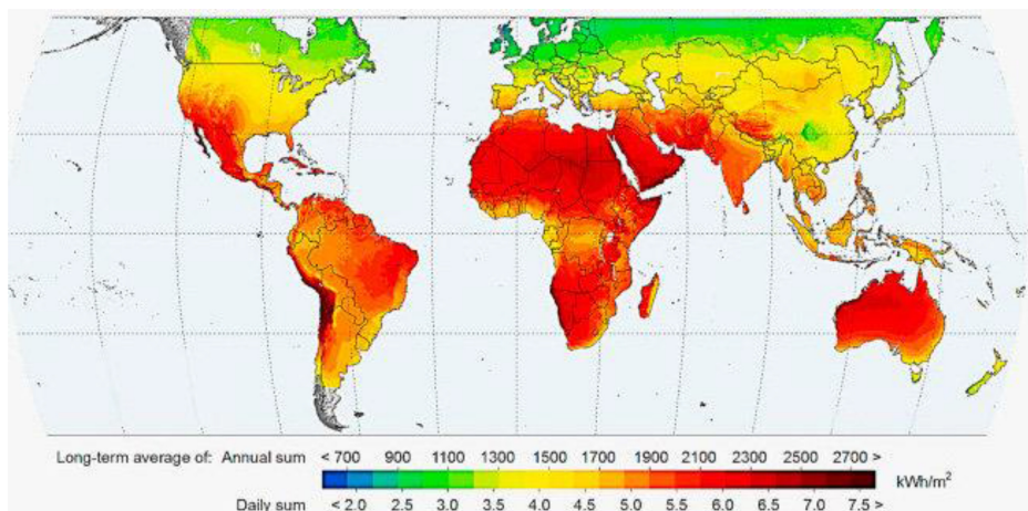
Figure 6.8. Global map of annual solar horizontal radiation [62]
