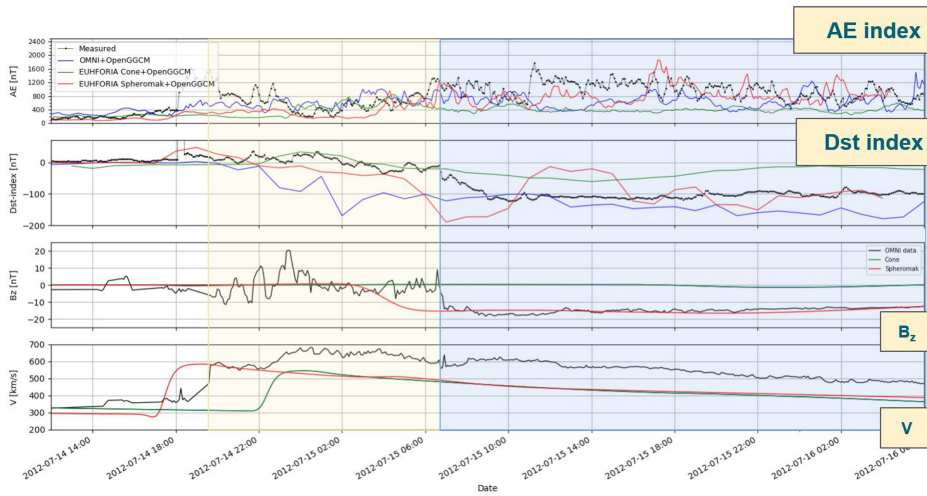
Figure 6.53. Preliminary result from coupling EUHFORIA to the magnetospheric model OpenGGCM. Reprinted by permission from Springer Nature, [247], copyright (2008). The standard nowcast, using measurements at L1, are compared with forecasts (3 days ahead) using synthetic L1 data from EUHFORIA. When a spheromak (magnetized) CME model is used, the forecast can stand the comparison with the nowcast. From top to bottom: comparison of AE index measurements to nowcast (OMNI-OpenGGCM) and forecasts based on EUHFORIA with a cone CME and a spheromak CMEs; the same for the Dst index; the measured B_z component compared to the predictions; and the same comparison for the radial velocity. (Source: Maharana et al (to be submitted).)
