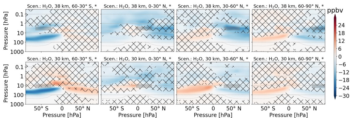
Figure 5. Zonal mean of \text{CH}_4 perturbation (volume mixing ratio, ppbv) for scenarios where \text{H}_2\text{O} is emitted. The first and second rows refer to 38 and 30 km altitudes of emission, respectively. Columns represent the latitude region of emission. The emission regions are shaded in gray. Lines indicate statistically insignificant results, and the probability level is written in the title of each subplot.
