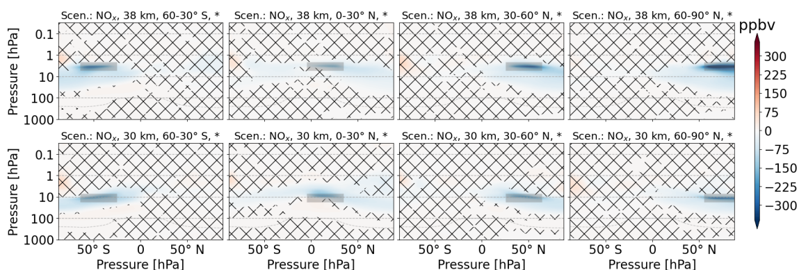
Figure 6. Zonal mean of \text{O}_3 perturbation (volume mixing ratio, ppbv) for scenarios where \text{NO}_x is emitted. The first and second rows refer to 38 and 30 km altitudes of emission, respectively. Columns represent the latitude region of emission. The emission regions are shaded in gray. Lines indicate statistically insignificant results, and the probability level is written in the title of each subplot.
